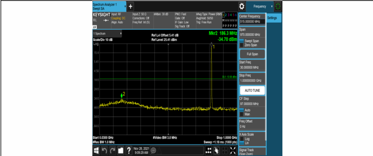
Band26-1.4MHz-QPSK-26740-6RB#0-Range1:30~1000MHz
