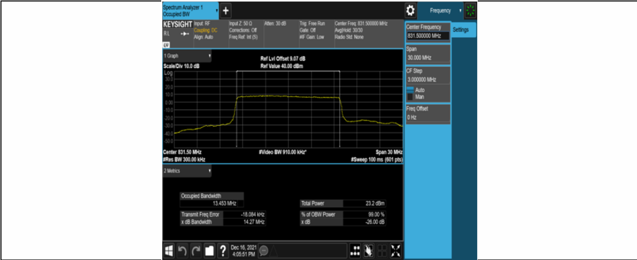
Band26-15MHz-QPSK-26865-75RB#0
