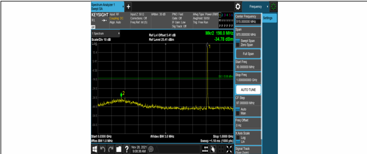
Band26-1.4MHz-QPSK-26697-6RB#0-Range1:30~1000MHz
