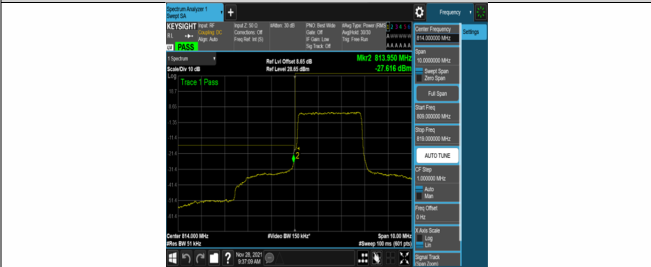
Band26-3MHz-QPSK-26705-15RB#0
