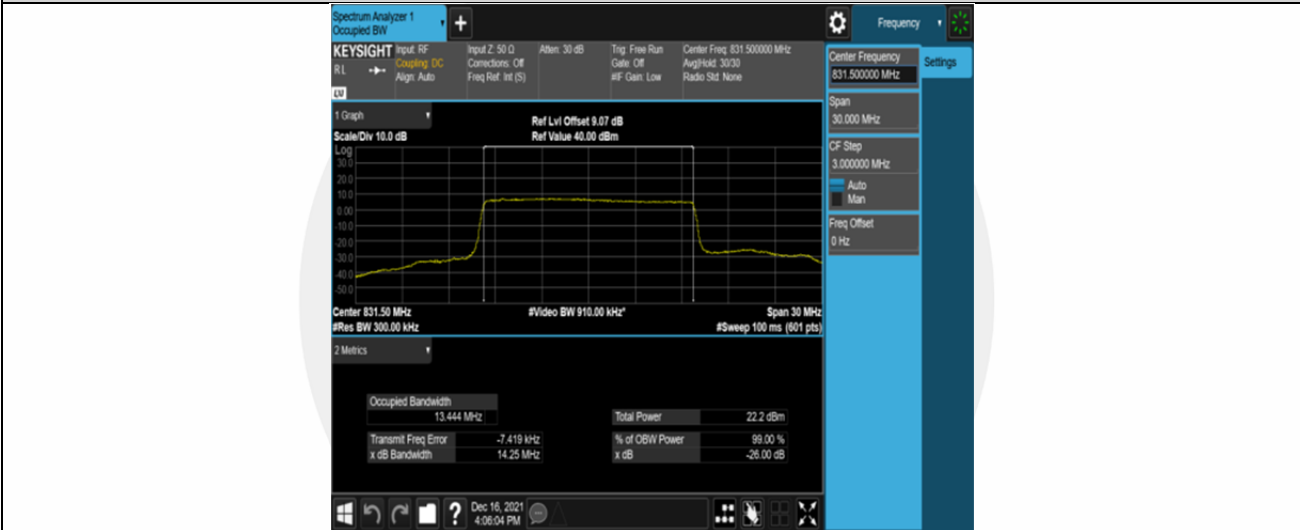
Band26-15MHz-16QAM-26865-75RB#0
