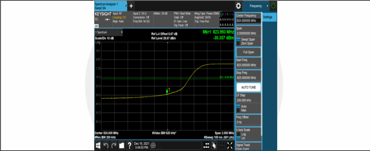
Band26-10MHz-16QAM-26840-50RB#0
