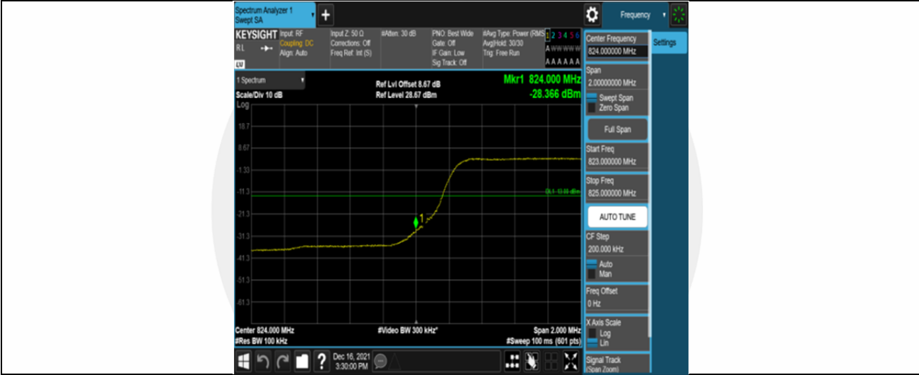
Band26-5MHz-16QAM-26815-25RB#0
