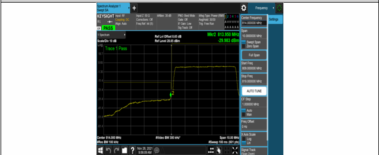
Band26-5MHz-16QAM-26715-25RB#0
