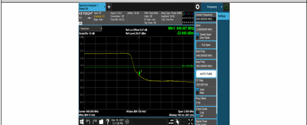
Band26-3MHz-QPSK-27025-15RB#0
