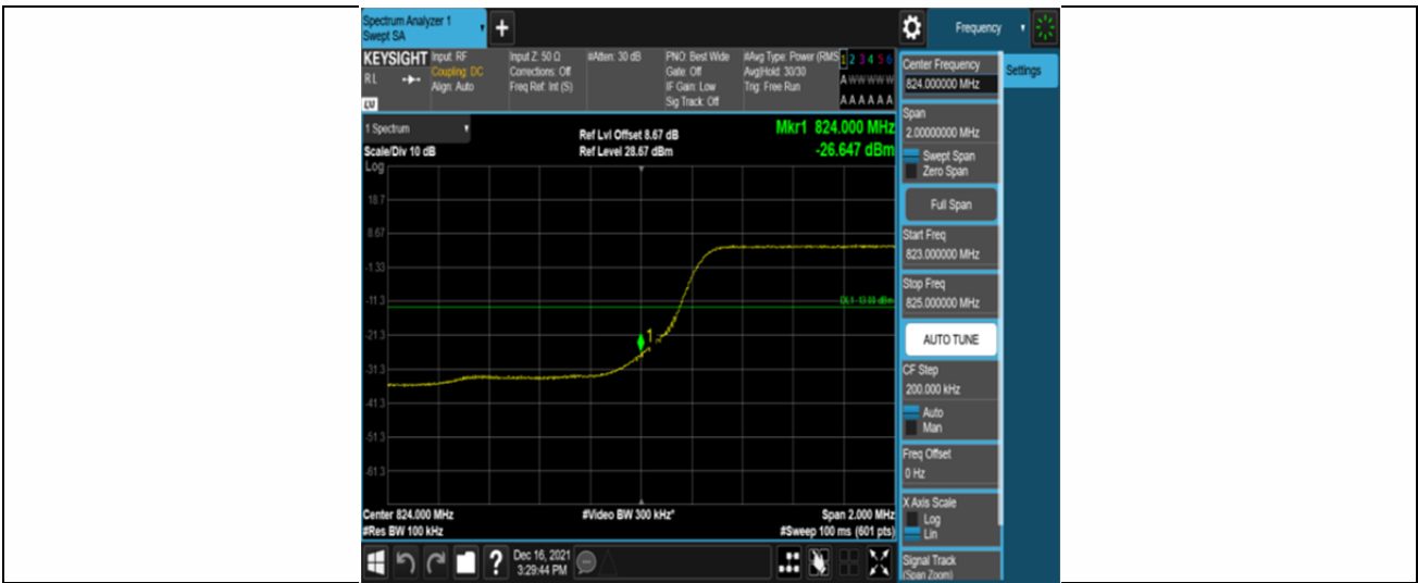
Band26-5MHz-QPSK-26815-25RB#0
