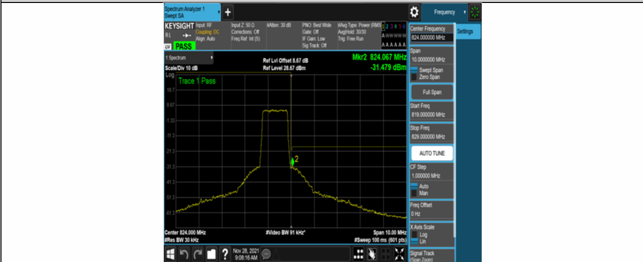
Band26-1.4MHz-16QAM-26783-6RB#0
