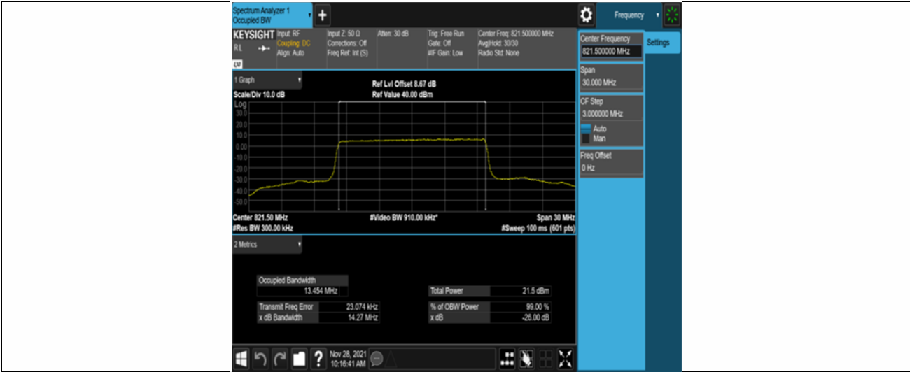
Band26-15MHz-16QAM-26765-75RB#0
