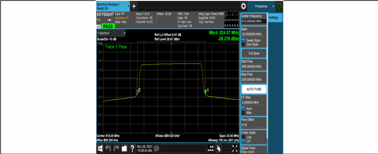
Band26-10MHz-QPSK-26740-50RB#0
