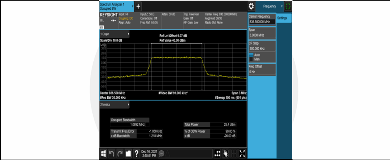
Band26-1.4MHz-QPSK-26915-6RB#0
