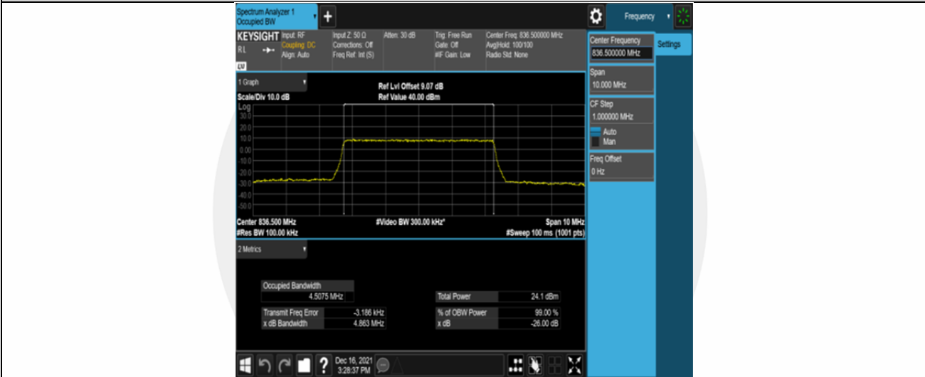
Band26-5MHz-16QAM-26915-25RB#0
