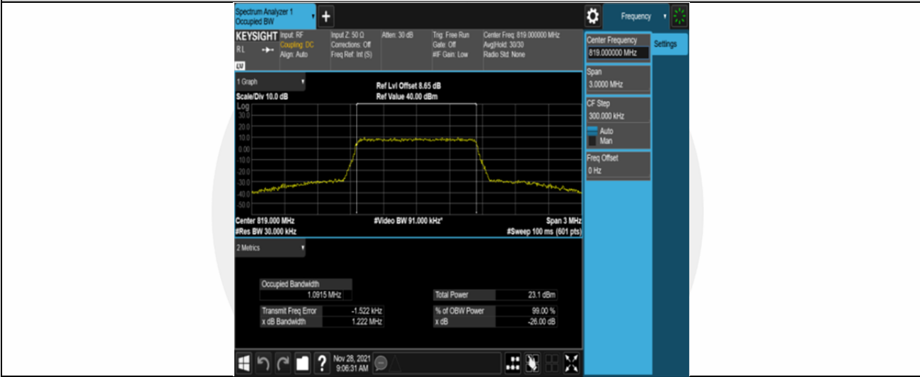
Band26-1.4MHz-16QAM-26740-6RB#0
