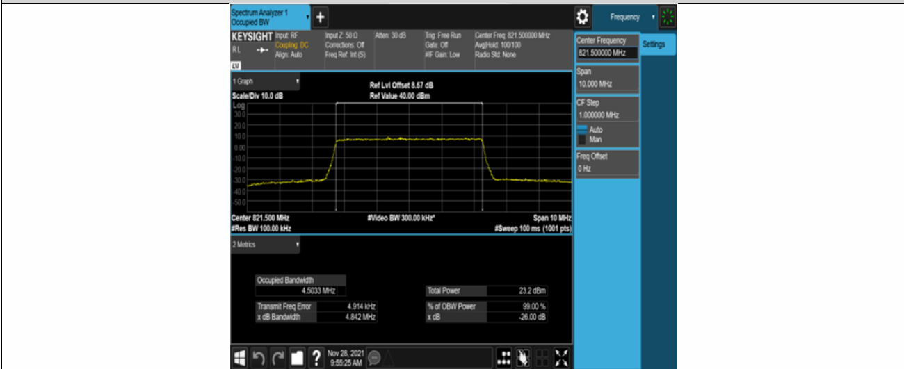
Band26-5MHz-16QAM-26765-25RB#0
