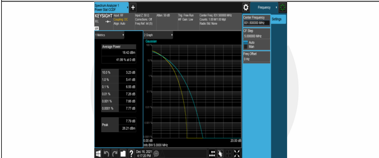
Band26-15MHz-16QAM-26865-75RB#0
