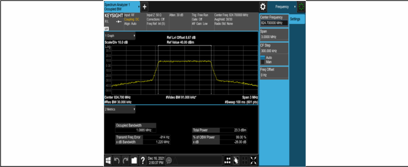
Band26-1.4MHz-16QAM-26797-6RB#0
