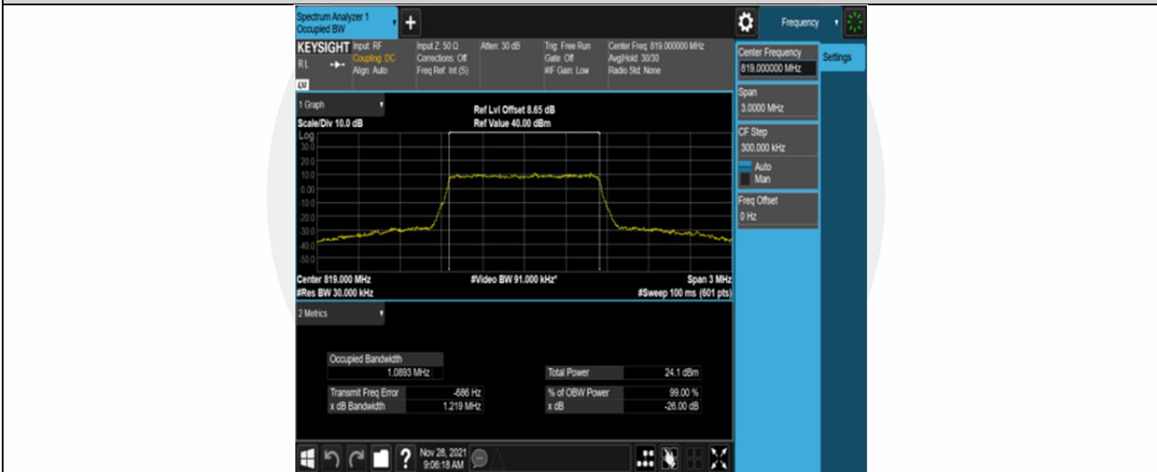
Band26-1.4MHz-QPSK-26740-6RB#0
