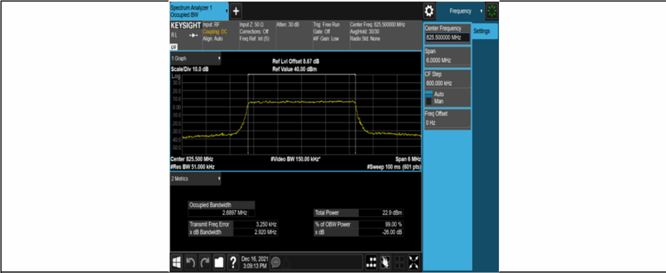
Band26-3MHz-16QAM-26805-15RB#0
