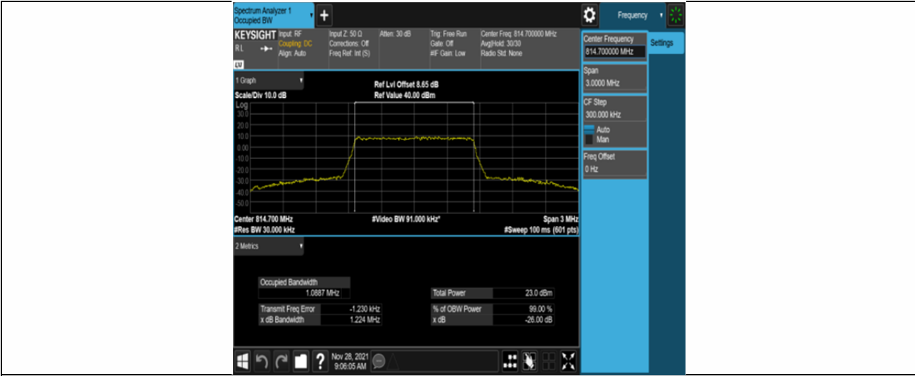
Band26-1.4MHz-16QAM-26697-6RB#0
