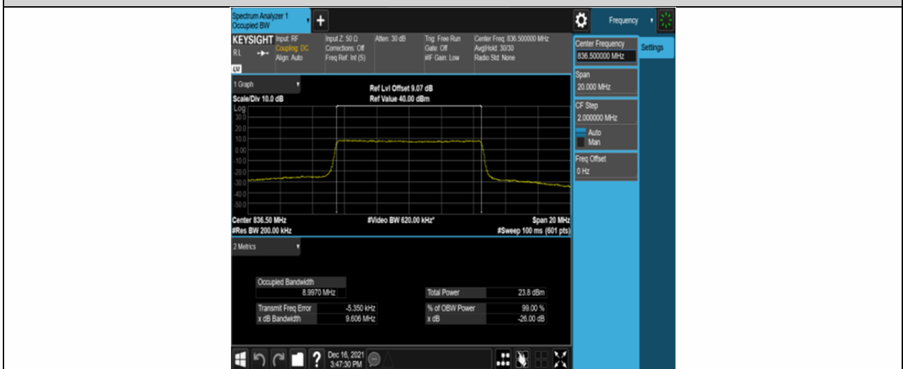
Band26-10MHz-QPSK-26915-50RB#0
