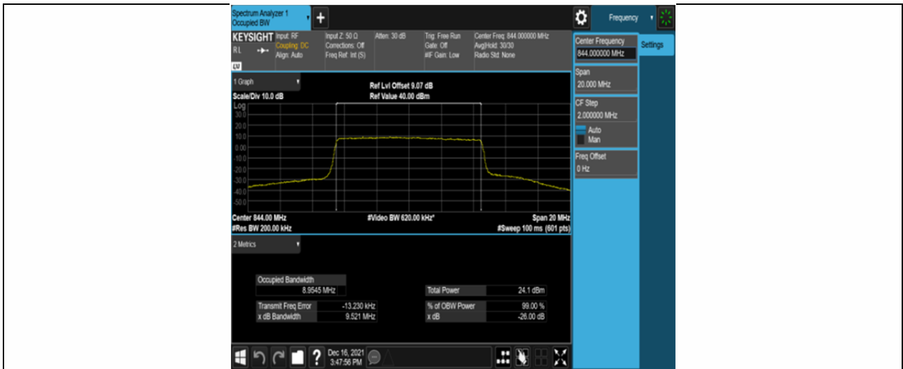
Band26-10MHz-QPSK-26990-50RB#0
