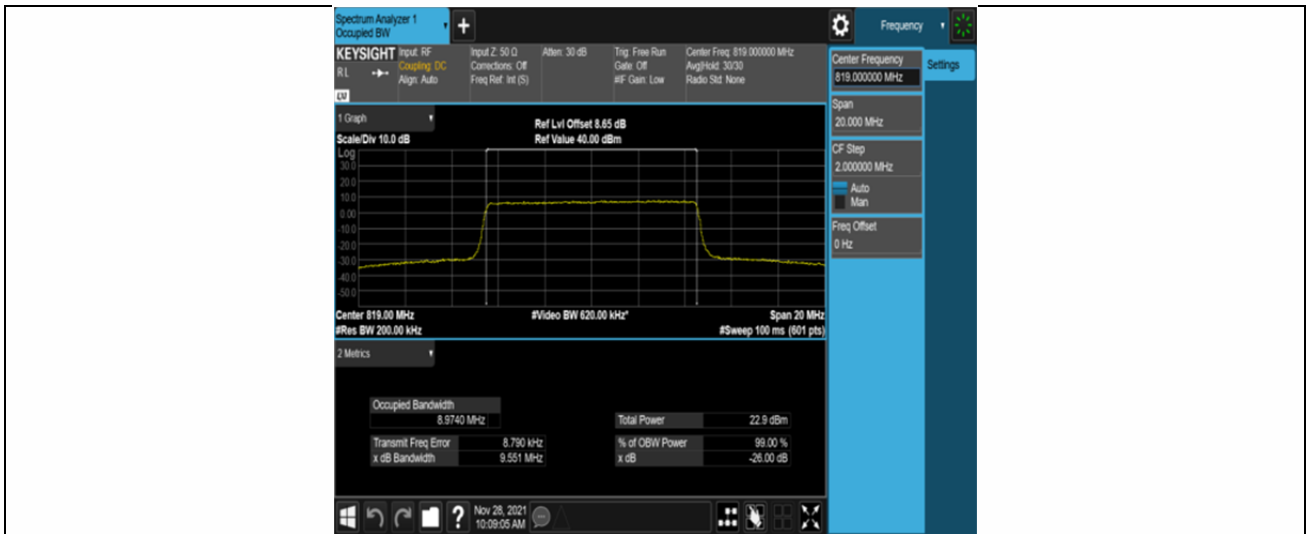
Band26-10MHz-QPSK-26740-50RB#0
