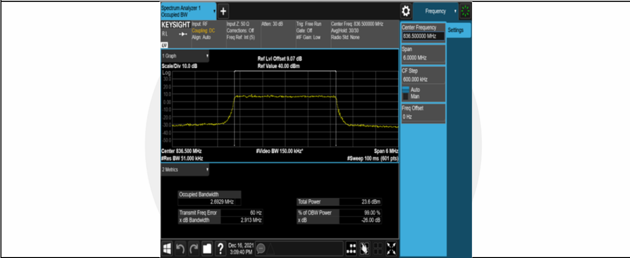
Band26-3MHz-16QAM-26915-15RB#0
