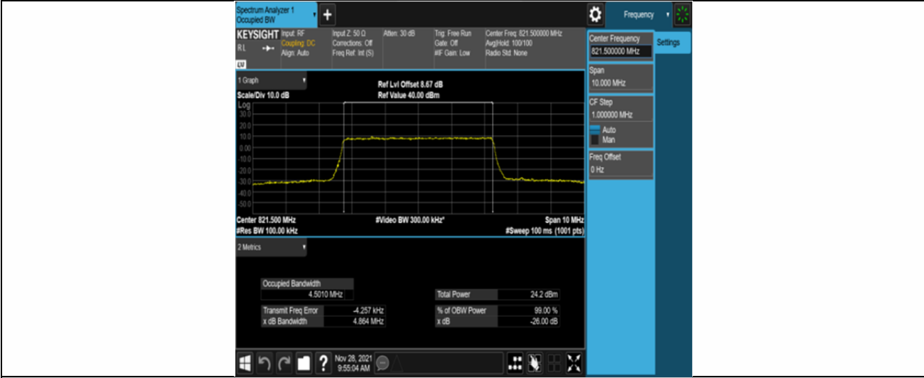
Band26-5MHz-QPSK-26765-25RB#0
