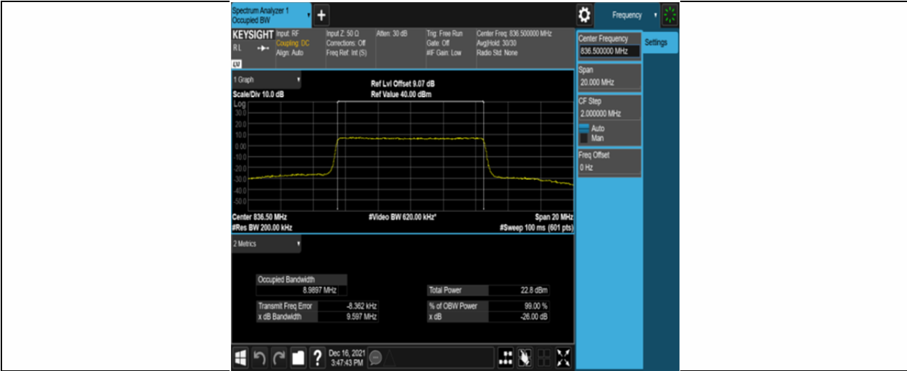
Band26-10MHz-16QAM-26915-50RB#0
