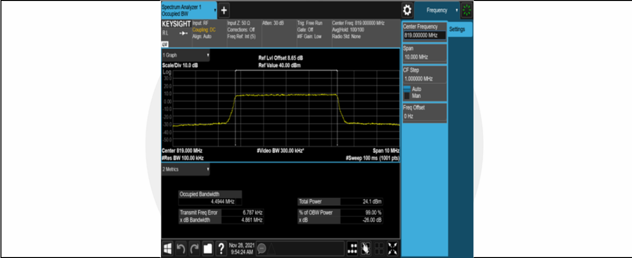
Band26-5MHz-QPSK-26740-25RB#0
