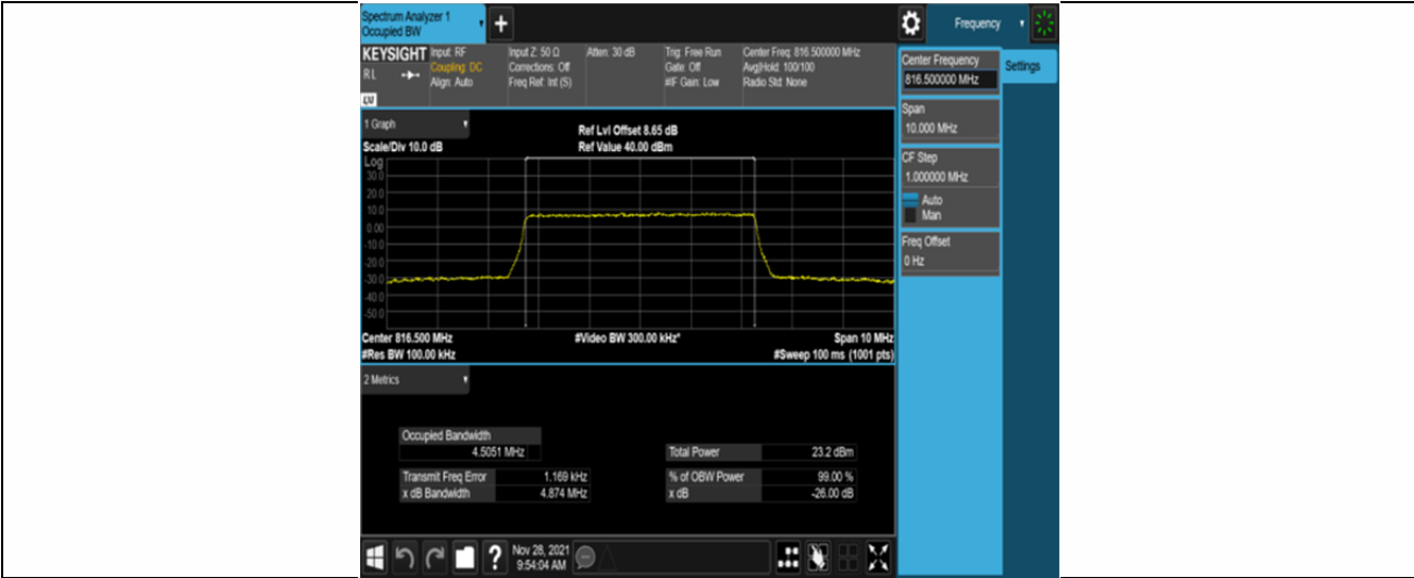
Band26-5MHz-16QAM-26715-25RB#0
