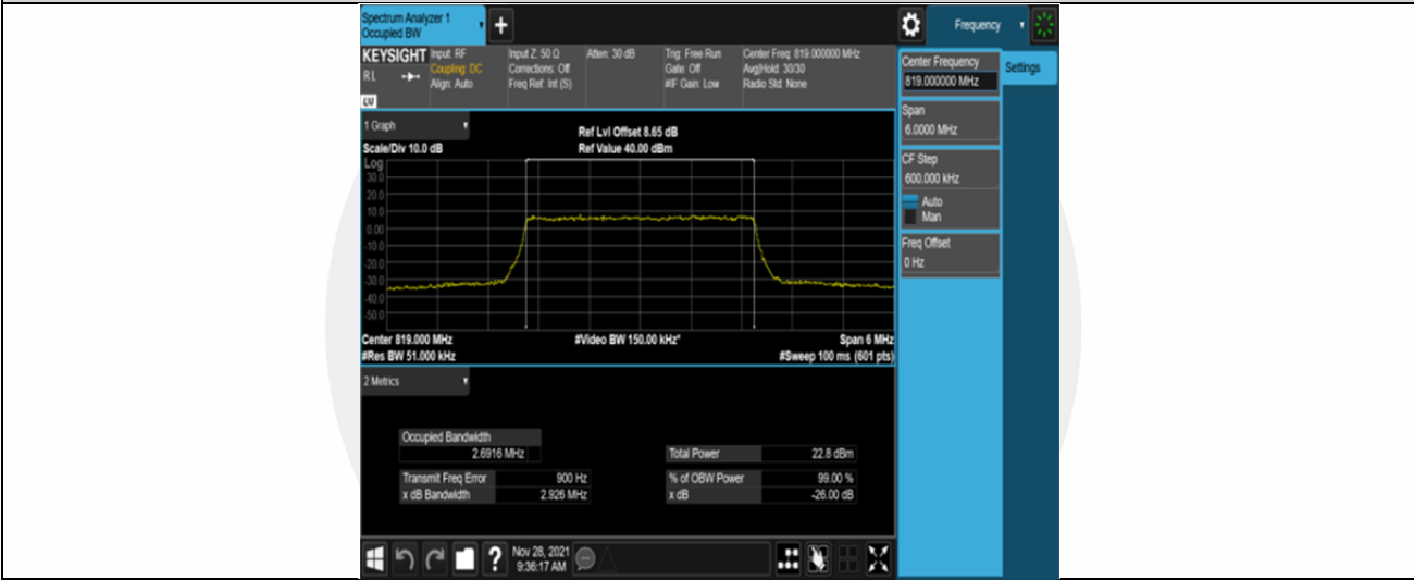
Band26-3MHz-16QAM-26740-15RB#0
