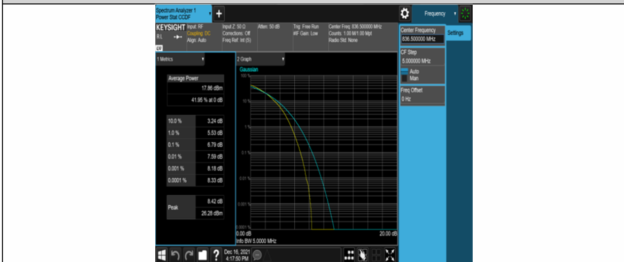
Band26-15MHz-16QAM-26915-75RB#0
