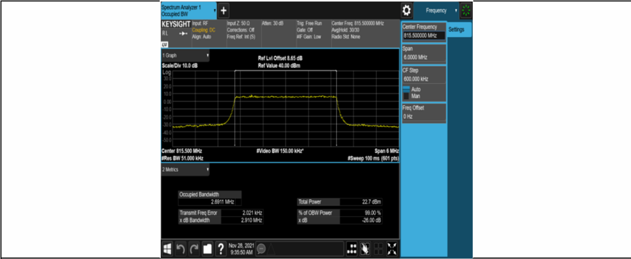
Band26-3MHz-16QAM-26705-15RB#0
