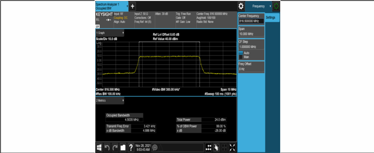
Band26-5MHz-QPSK-26715-25RB#0
