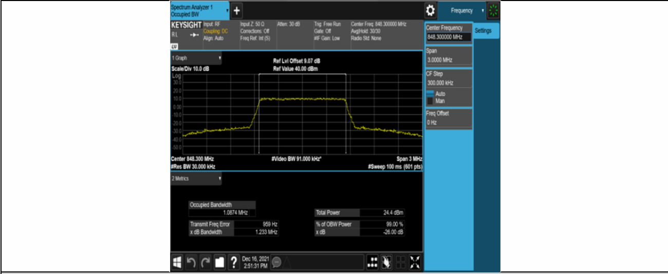
Band26-1.4MHz-16QAM-27033-6RB#0
