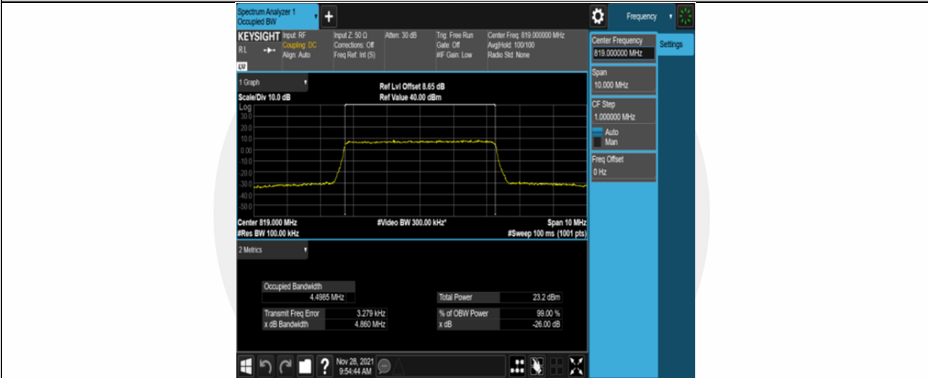
Band26-5MHz-16QAM-26740-25RB#0
