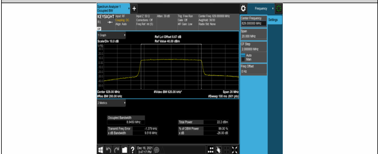
Band26-10MHz-16QAM-26840-50RB#0
