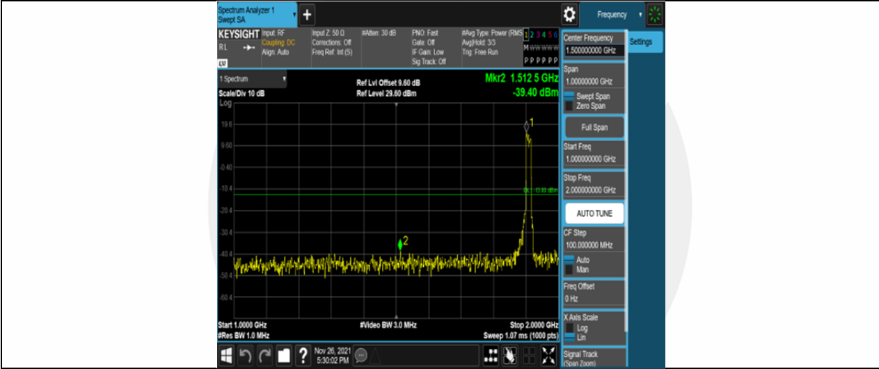
Band25-15MHz-16QAM-26615-75RB#0-Range2:1000~2000MHz
