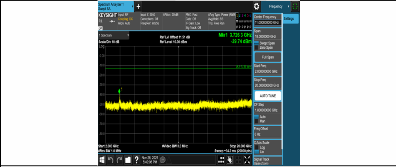
Band25-20MHz-QPSK-26140-100RB#0-Range3:2000~20000MHz
