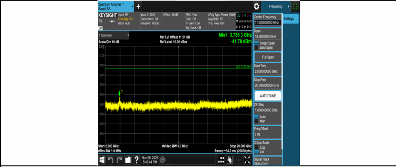
Band25-20MHz-16QAM-26140-100RB#0-Range3:2000~20000MHz
