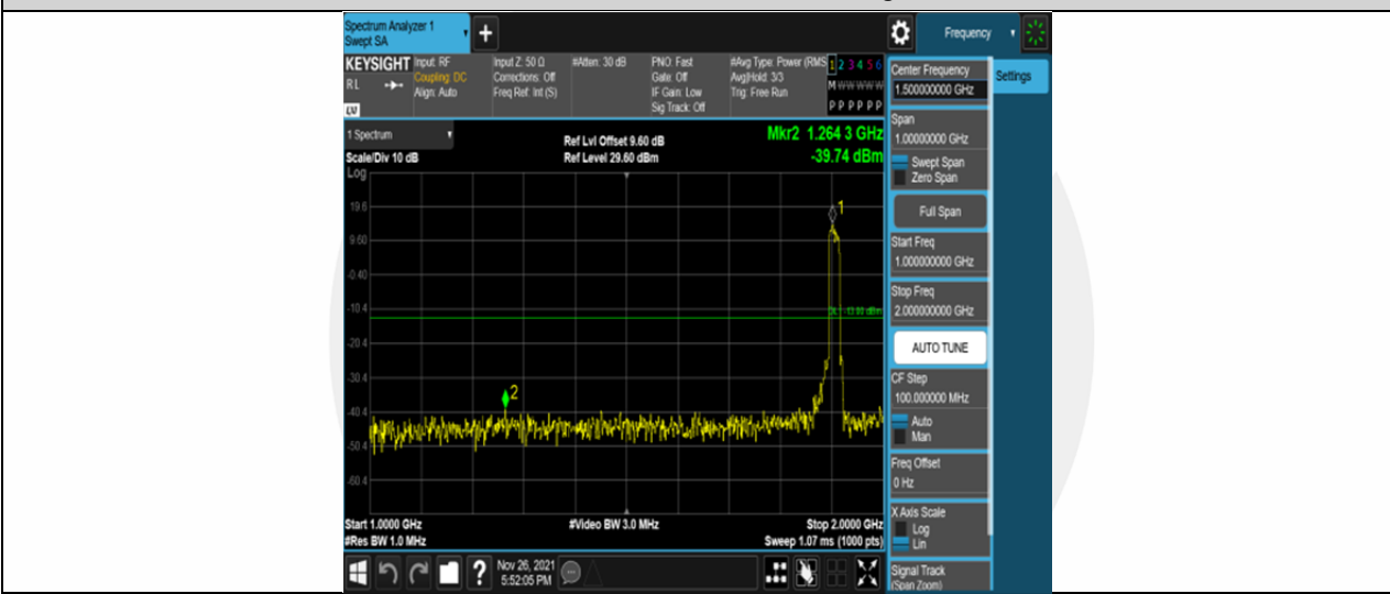
Band25-20MHz-16QAM-26590-100RB#0-Range2:1000~2000MHz
