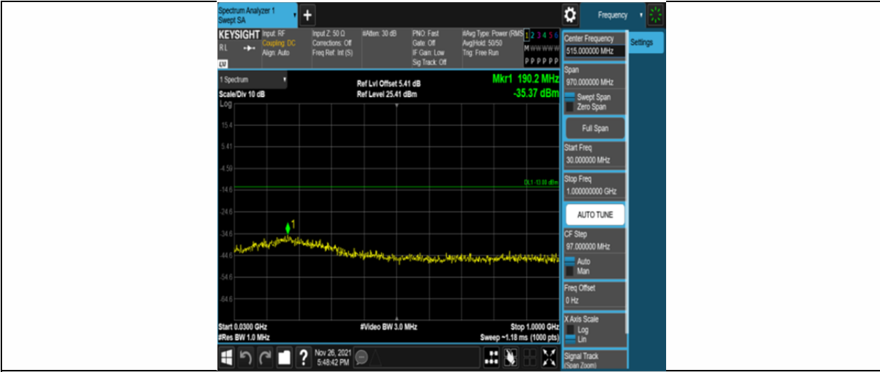
Band25-20MHz-QPSK-26140-100RB#0-Range1:30~1000MHz
