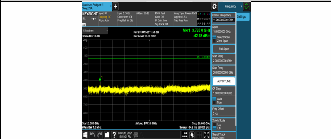
Band25-20MHz-16QAM-26365-100RB#0-Range3:2000~20000MHz
