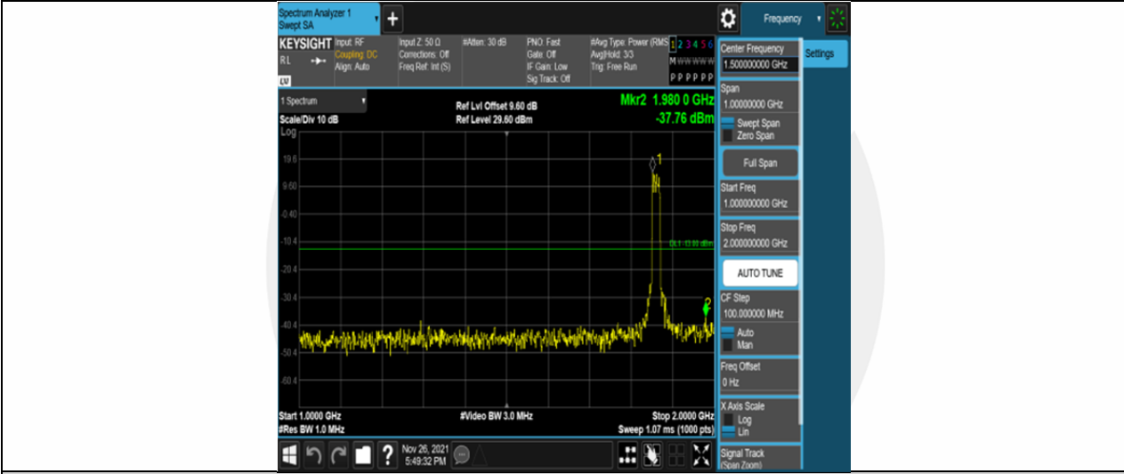
Band25-20MHz-16QAM-26140-100RB#0-Range2:1000~2000MHz
