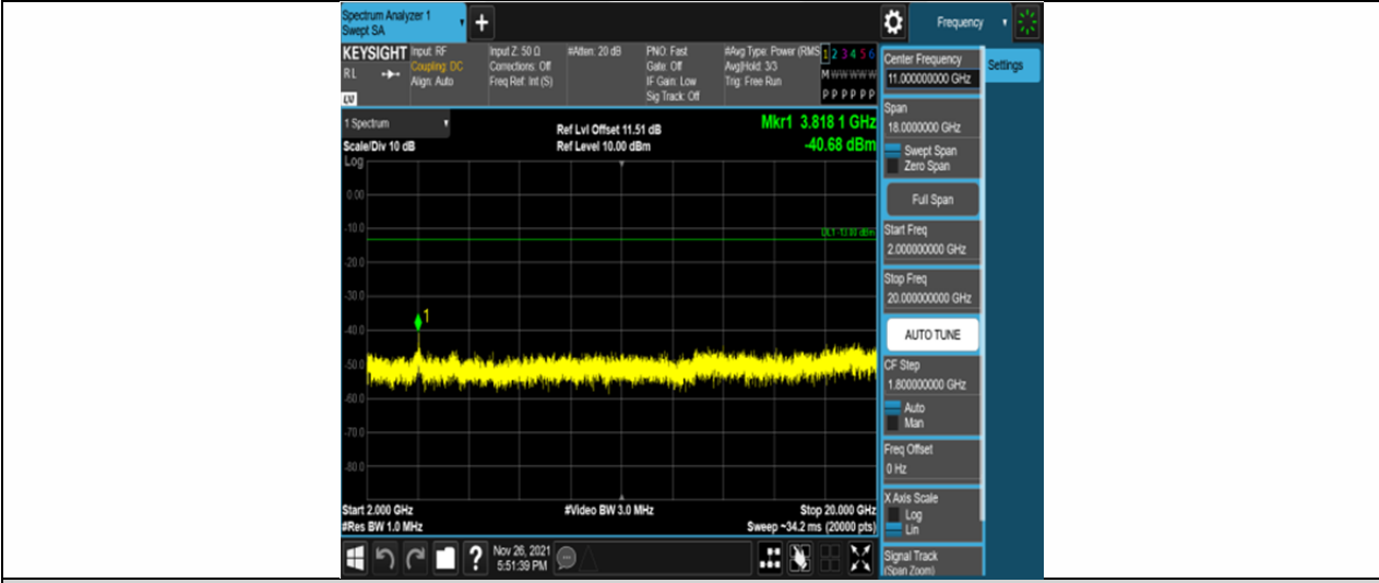
Band25-20MHz-QPSK-26590-100RB#0-Range3:2000~20000MHz
