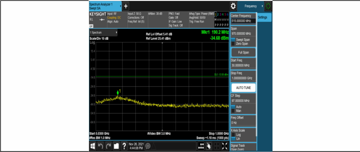
Band25-5MHz-16QAM-26065-25RB#0-Range1:30~1000MHz
