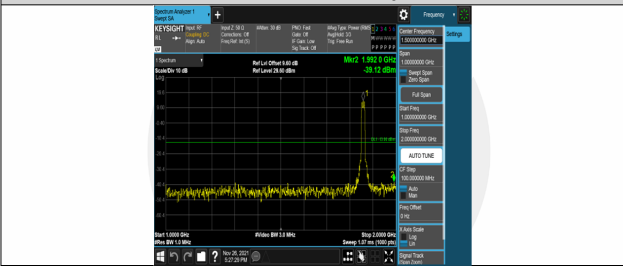
Band25-15MHz-16QAM-26115-75RB#0-Range2:1000~2000MHz
