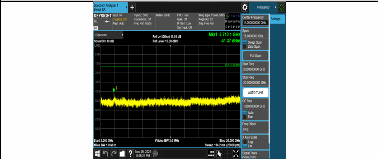
Band25-10MHz-QPSK-26090-50RB#0-Range3:2000~20000MHz
