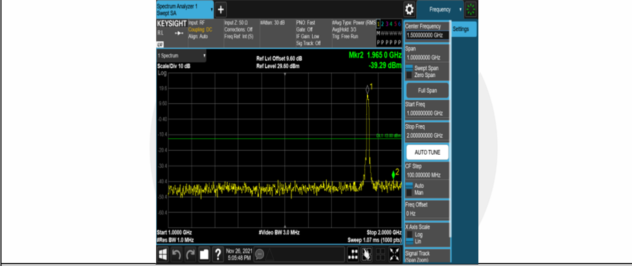
Band25-10MHz-16QAM-26090-50RB#0-Range2:1000~2000MHz
