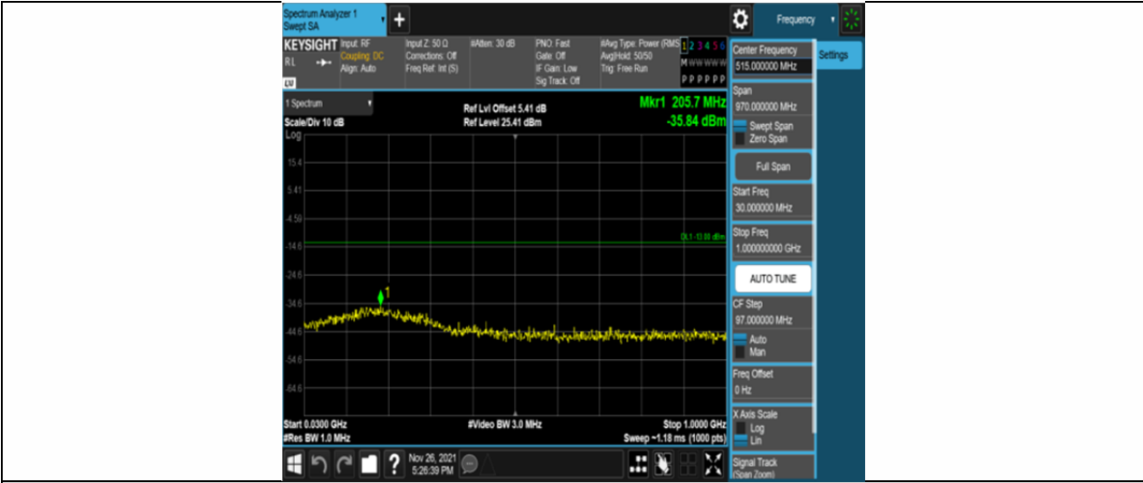
Band25-15MHz-QPSK-26115-75RB#0-Range1:30~1000MHz
