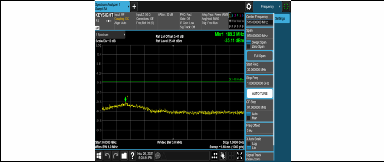
Band25-15MHz-16QAM-26365-75RB#0-Range1:30~1000MHz
