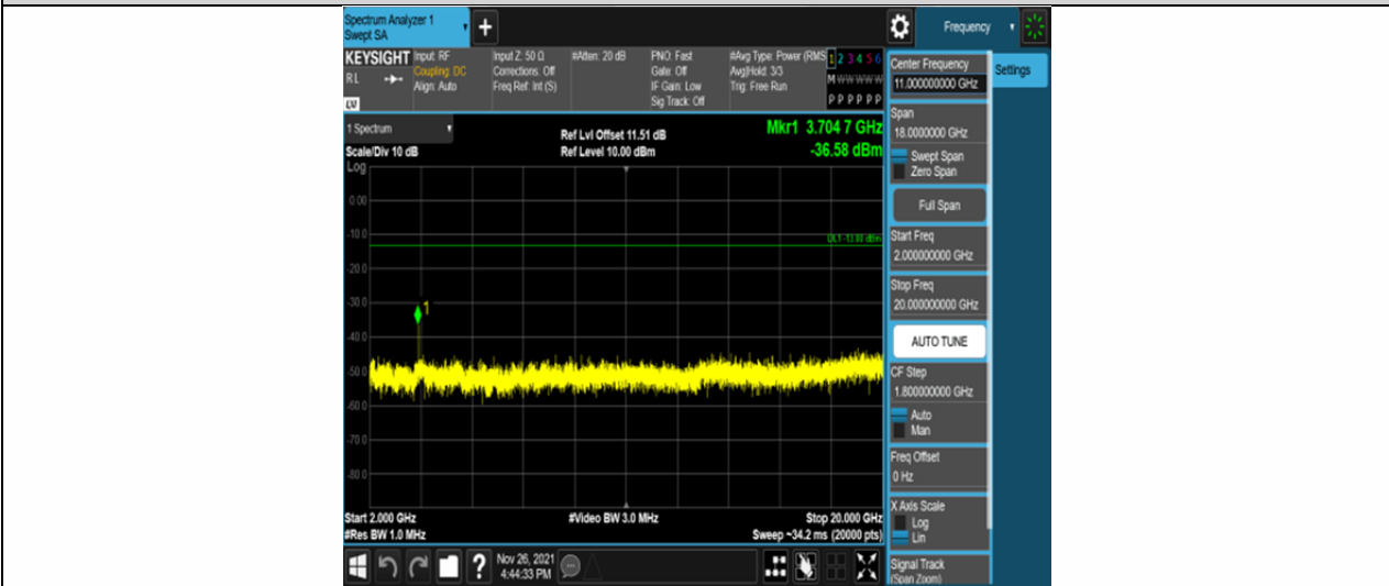
Band25-5MHz-16QAM-26065-25RB#0-Range3:2000~20000MHz
