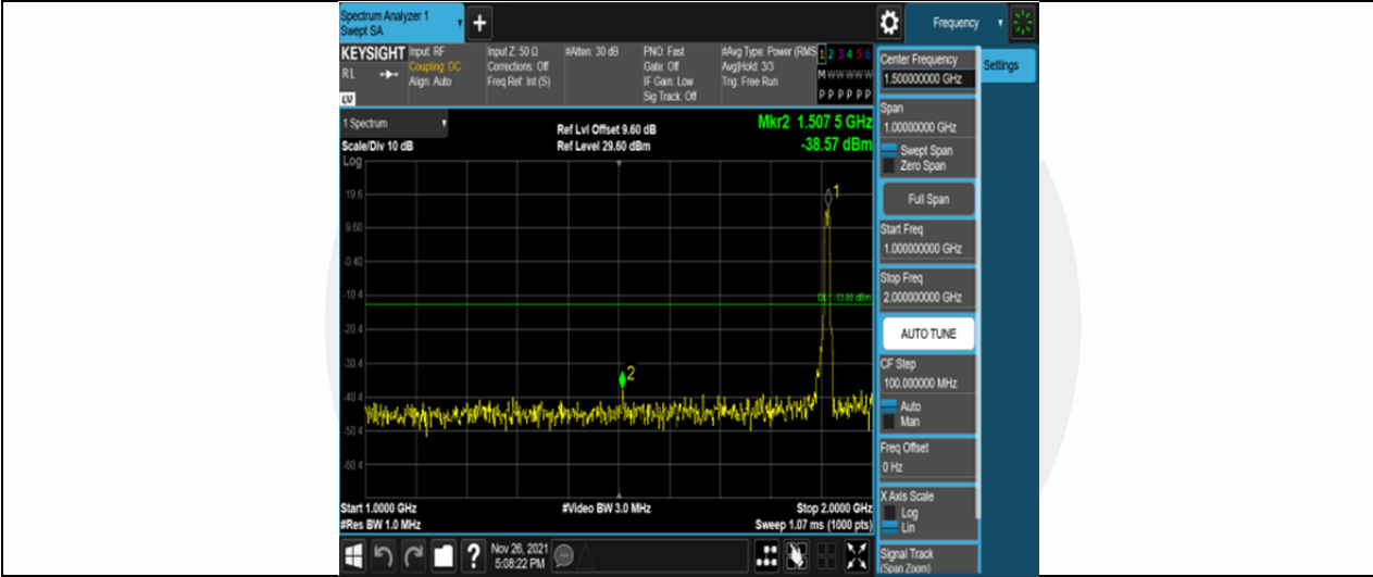
Band25-10MHz-16QAM-26640-50RB#0-Range2:1000~2000MHz
