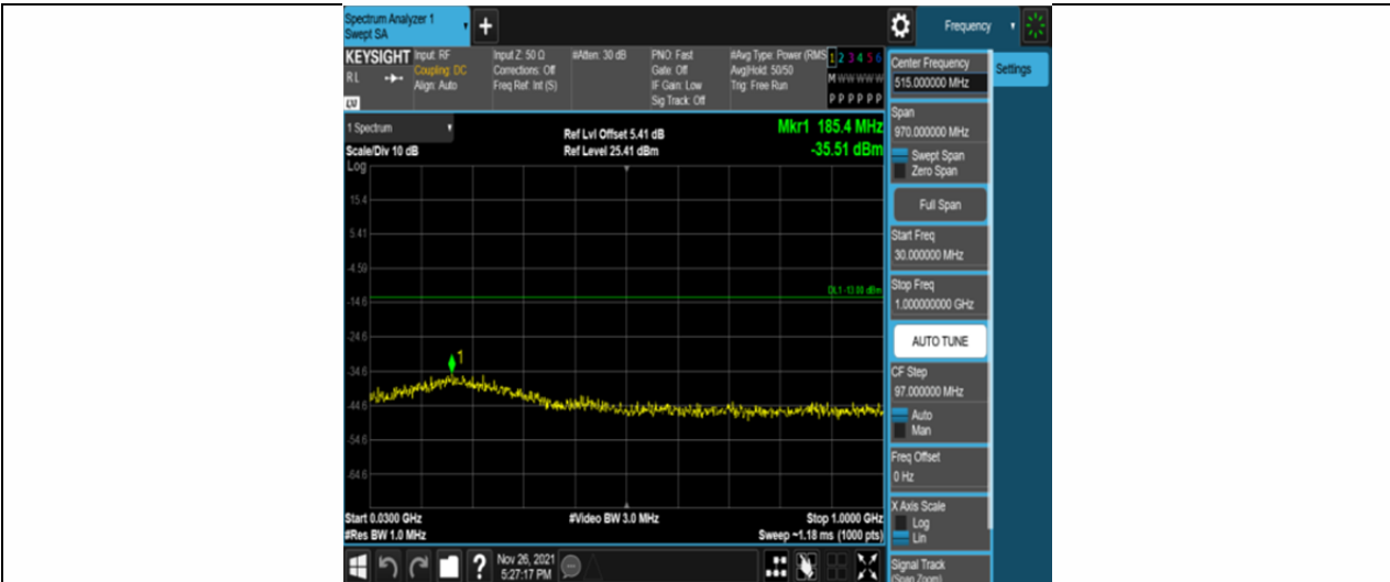
Band25-15MHz-16QAM-26115-75RB#0-Range1:30~1000MHz
