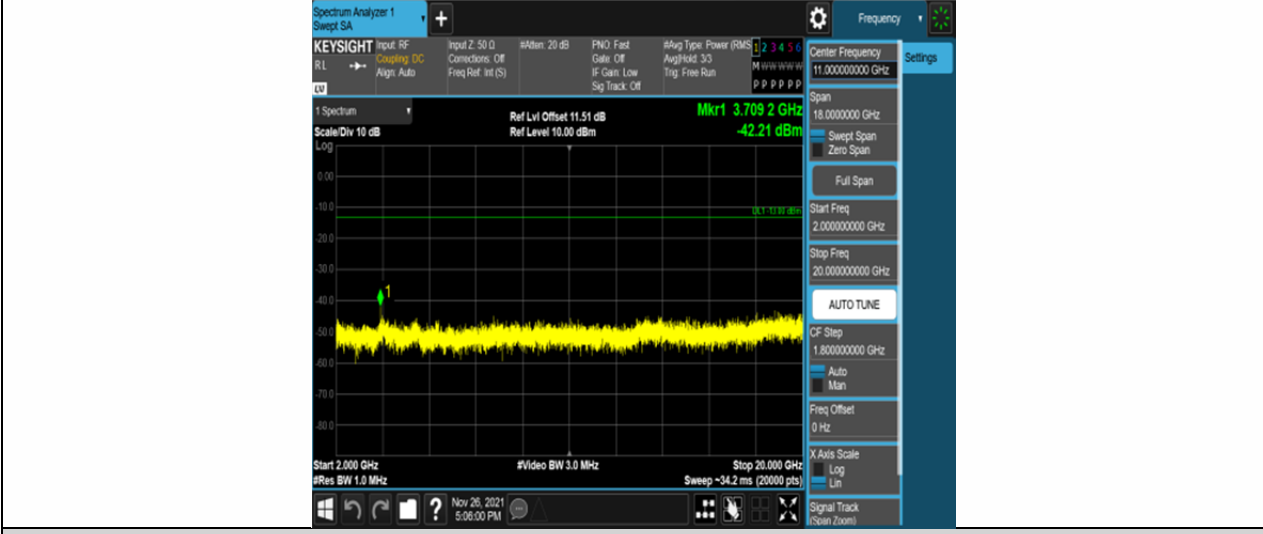
Band25-10MHz-16QAM-26090-50RB#0-Range3:2000~20000MHz
