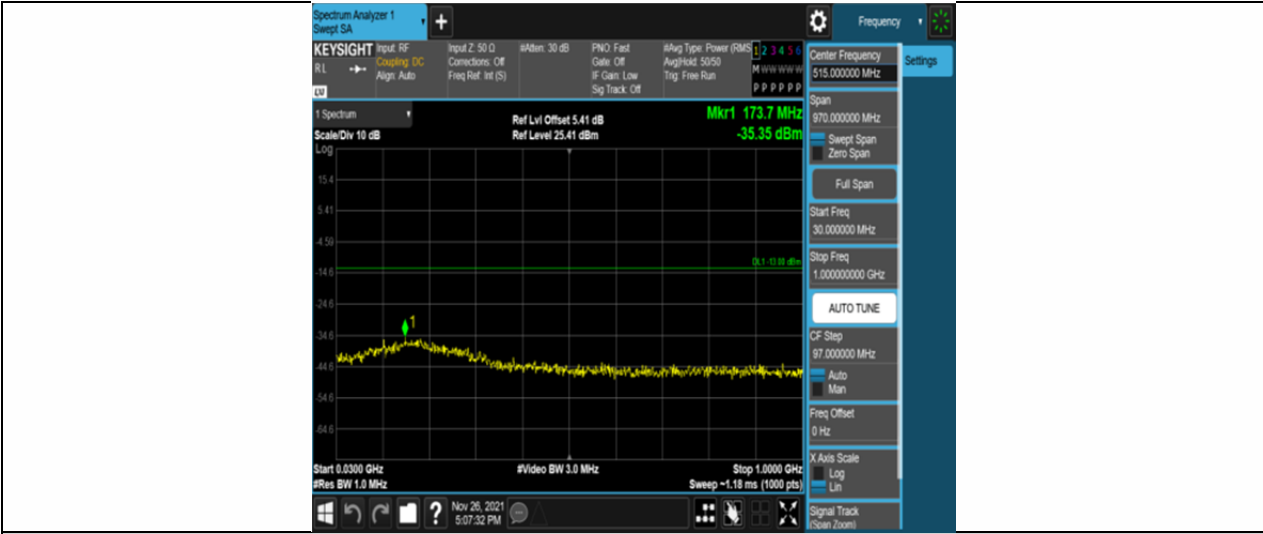
Band25-10MHz-QPSK-26640-50RB#0-Range1:30~1000MHz
