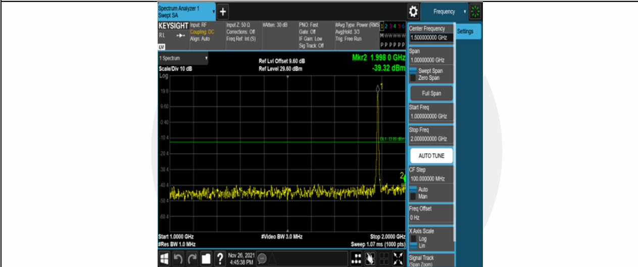
Band25-5MHz-16QAM-26365-25RB#0-Range2:1000~2000MHz
