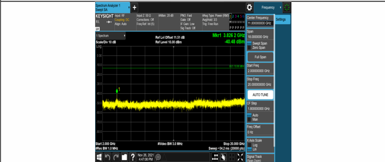
Band25-5MHz-16QAM-26665-25RB#0-Range3:2000~20000MHz
