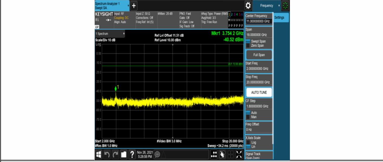
Band25-15MHz-16QAM-26365-75RB#0-Range3:2000~20000MHz
