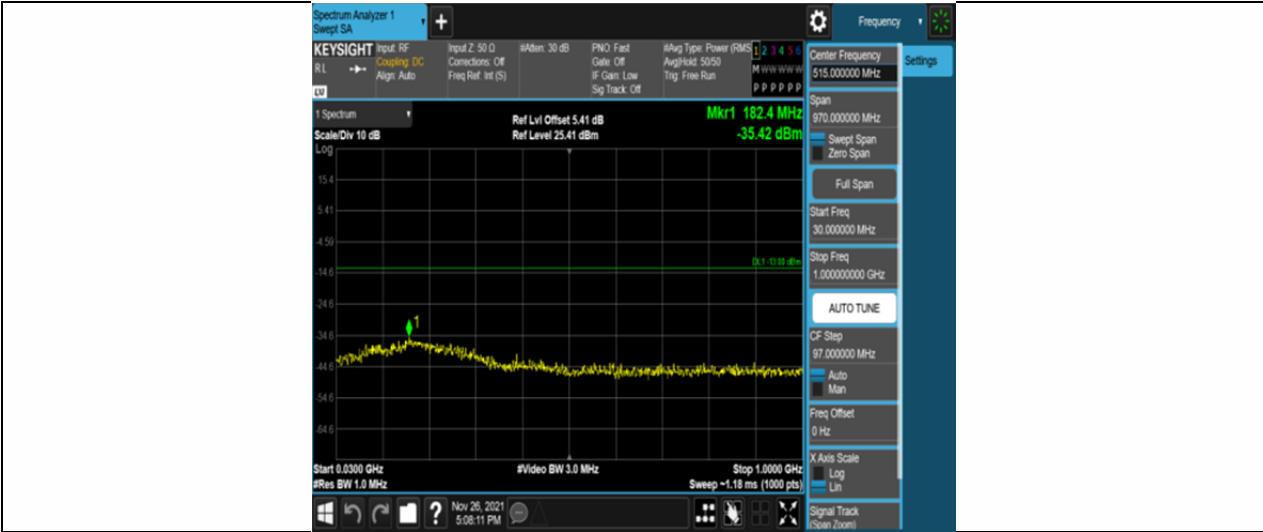
Band25-10MHz-16QAM-26640-50RB#0-Range1:30~1000MHz
