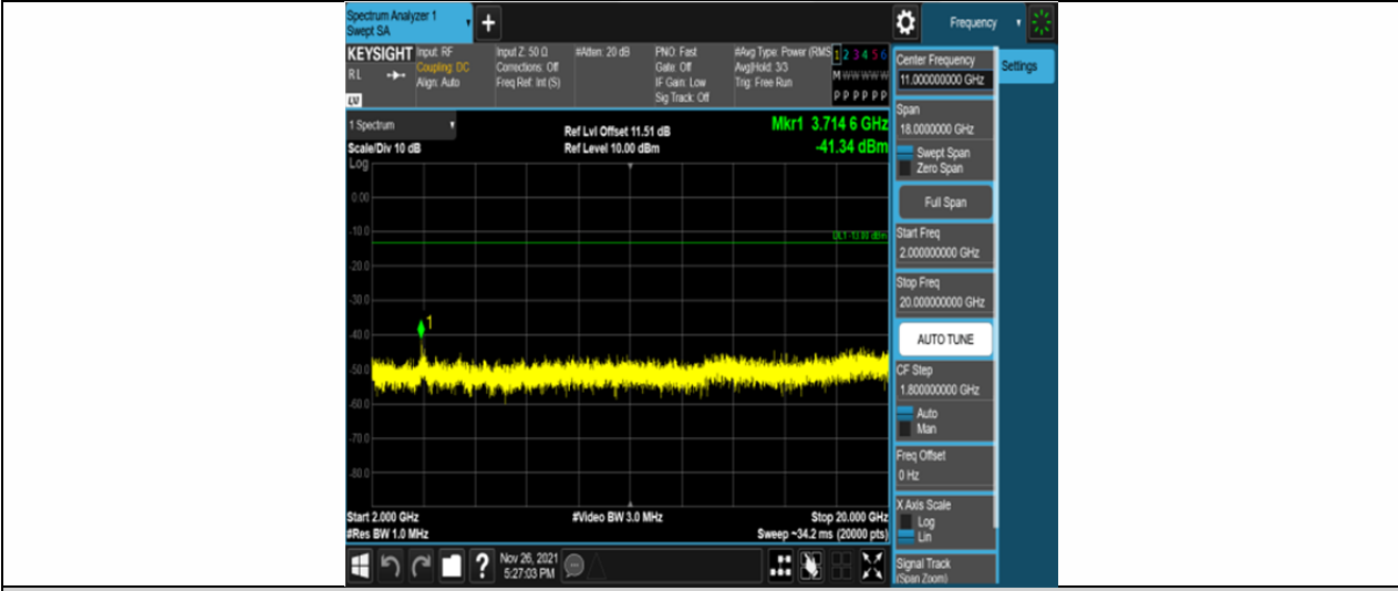
Band25-15MHz-QPSK-26115-75RB#0-Range3:2000~20000MHz
