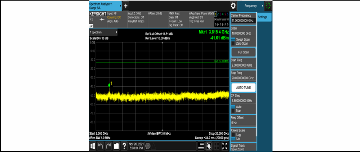
Band25-10MHz-16QAM-26640-50RB#0-Range3:2000~20000MHz
