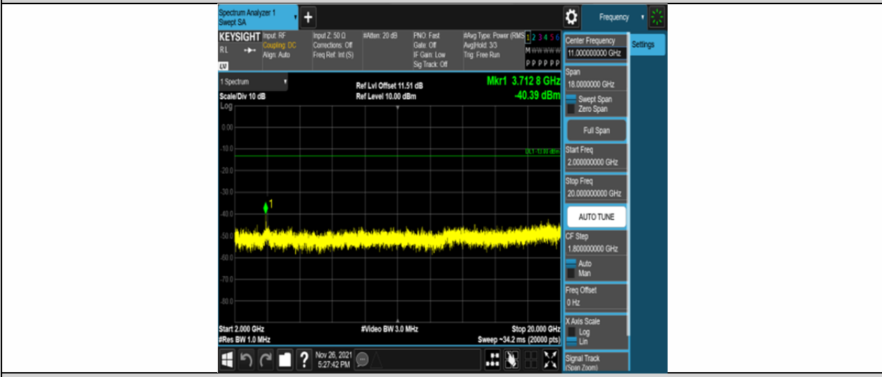
Band25-15MHz-16QAM-26115-75RB#0-Range3:2000~20000MHz
