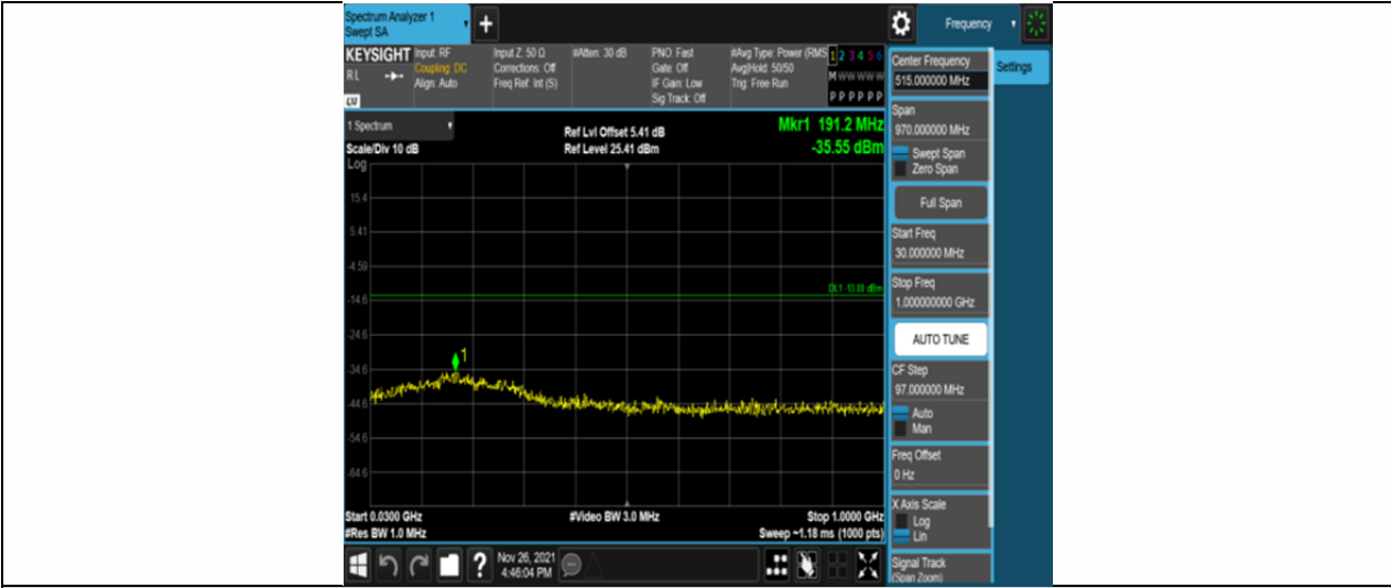
Band25-5MHz-QPSK-26665-25RB#0-Range1:30~1000MHz
