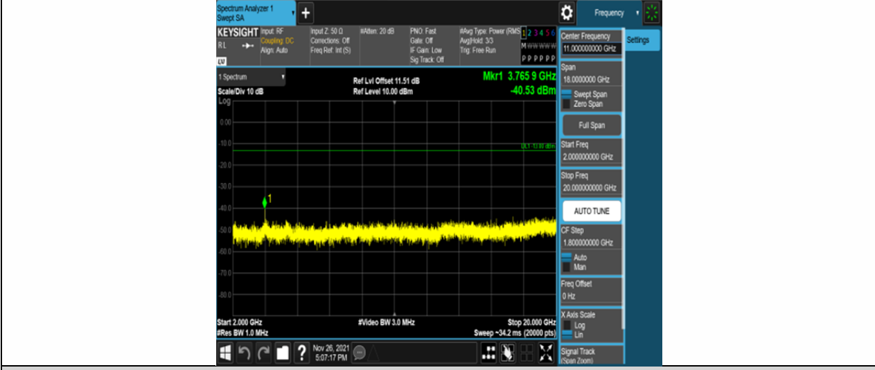
Band25-10MHz-16QAM-26365-50RB#0-Range3:2000~20000MHz
