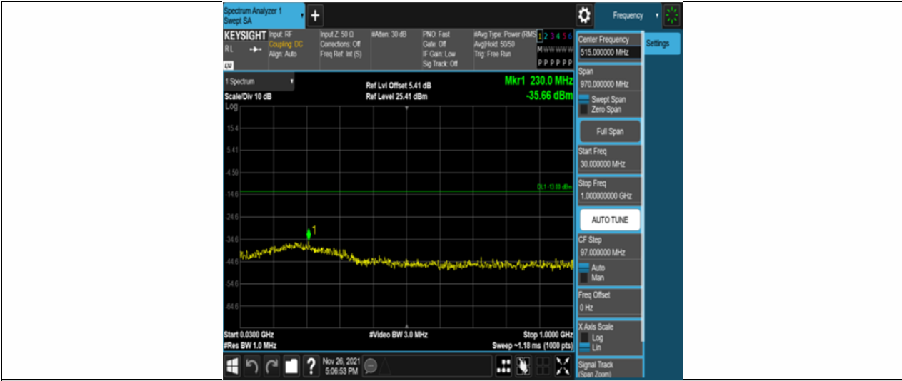
Band25-10MHz-16QAM-26365-50RB#0-Range1:30~1000MHz
