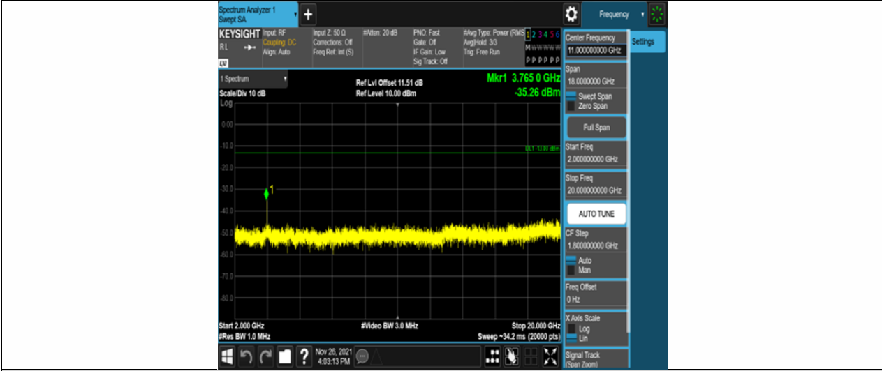
Band25-1.4MHz-16QAM-26365-6RB#0-Range3:2000~20000MHz
