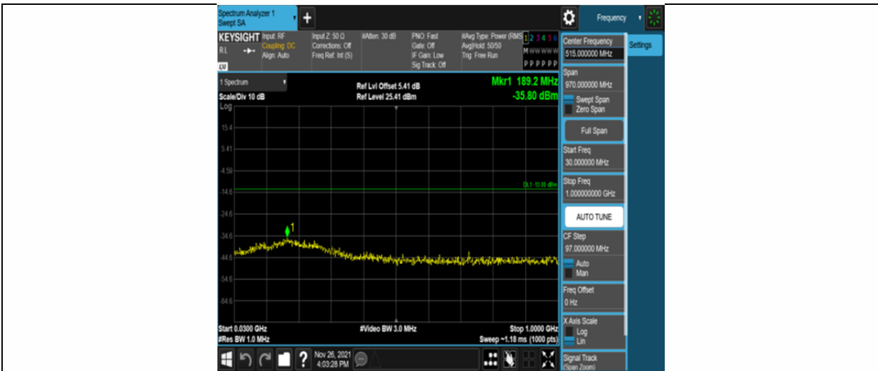
Band25-1.4MHz-QPSK-26683-6RB#0-Range1:30~1000MHz
