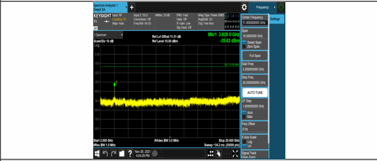
Band25-1.4MHz-16QAM-26683-6RB#0-Range3:2000~20000MHz
