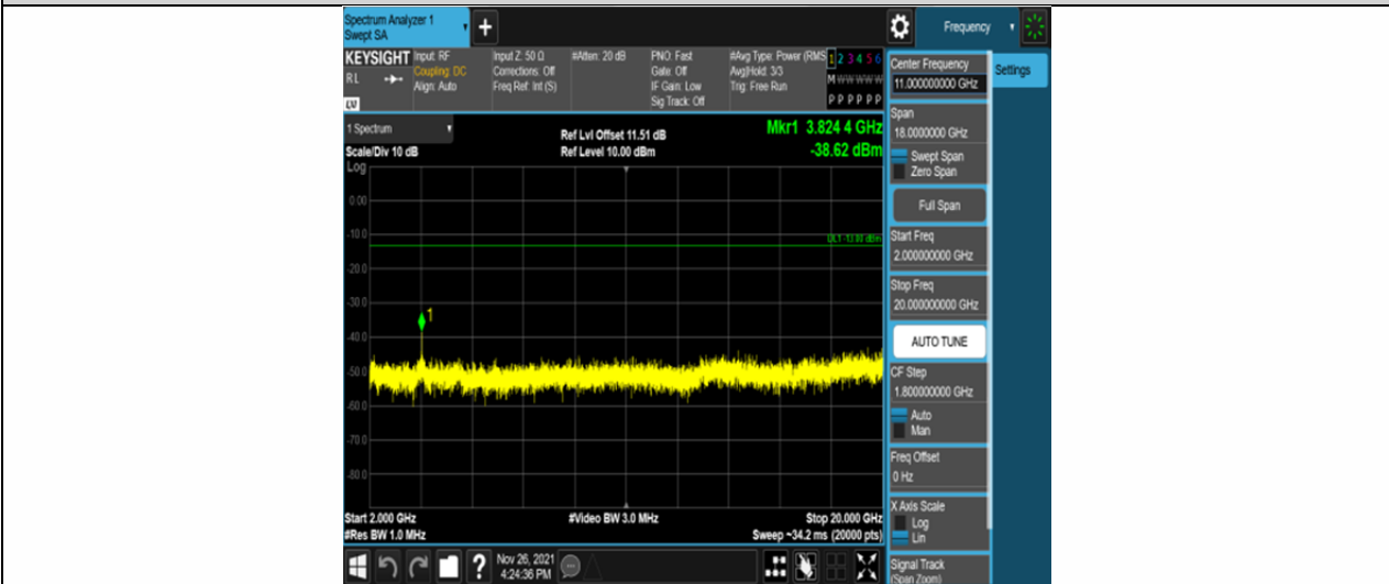
Band25-3MHz-QPSK-26675-1RB#0-Range3:2000~20000MHz
