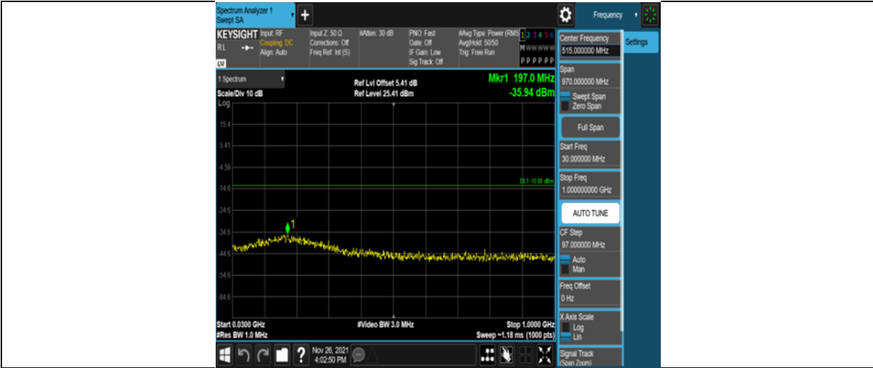
Band25-1.4MHz-16QAM-26365-6RB#0-Range1:30~1000MHz
