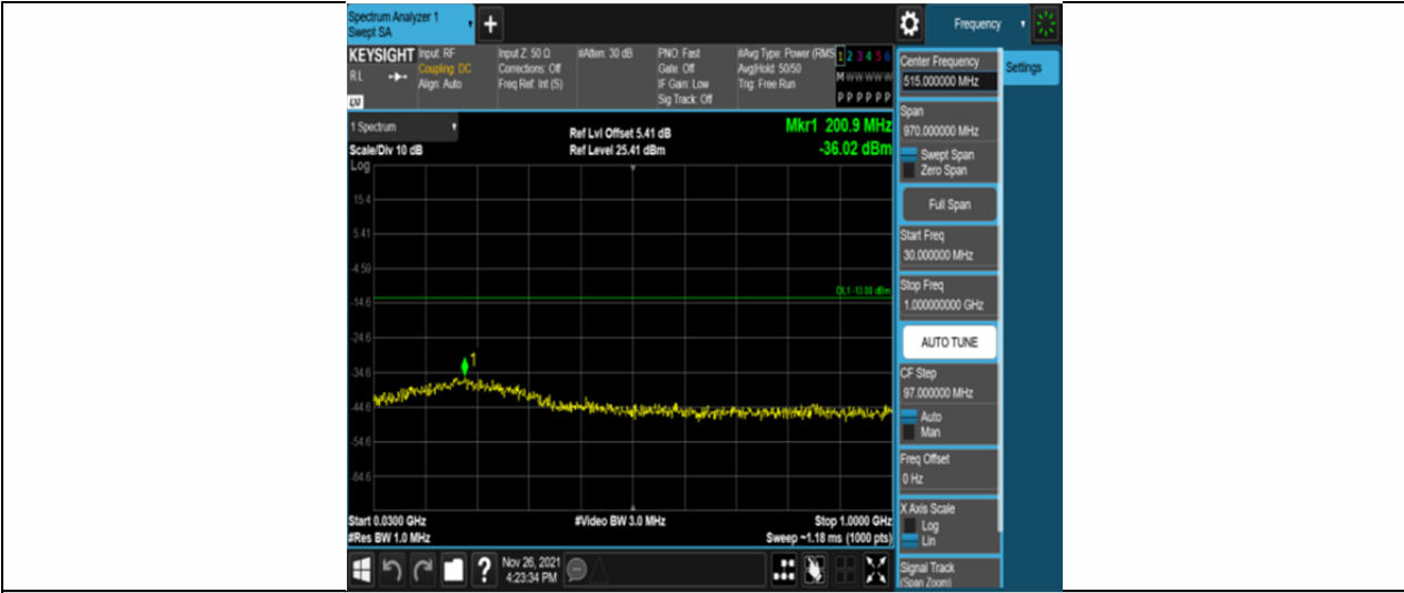
Band25-3MHz-16QAM-26365-1RB#0-Range1:30~1000MHz
