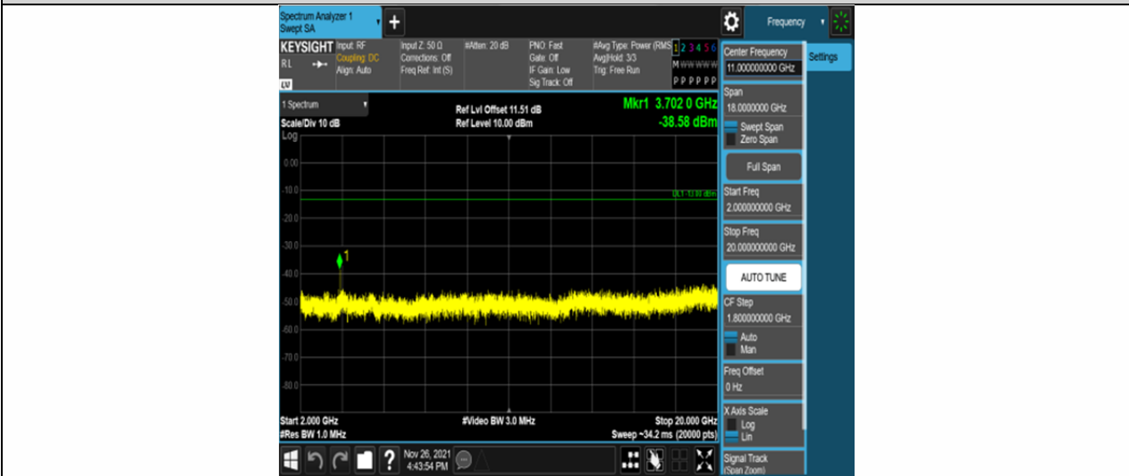
Band25-5MHz-QPSK-26065-25RB#0-Range3:2000~20000MHz
