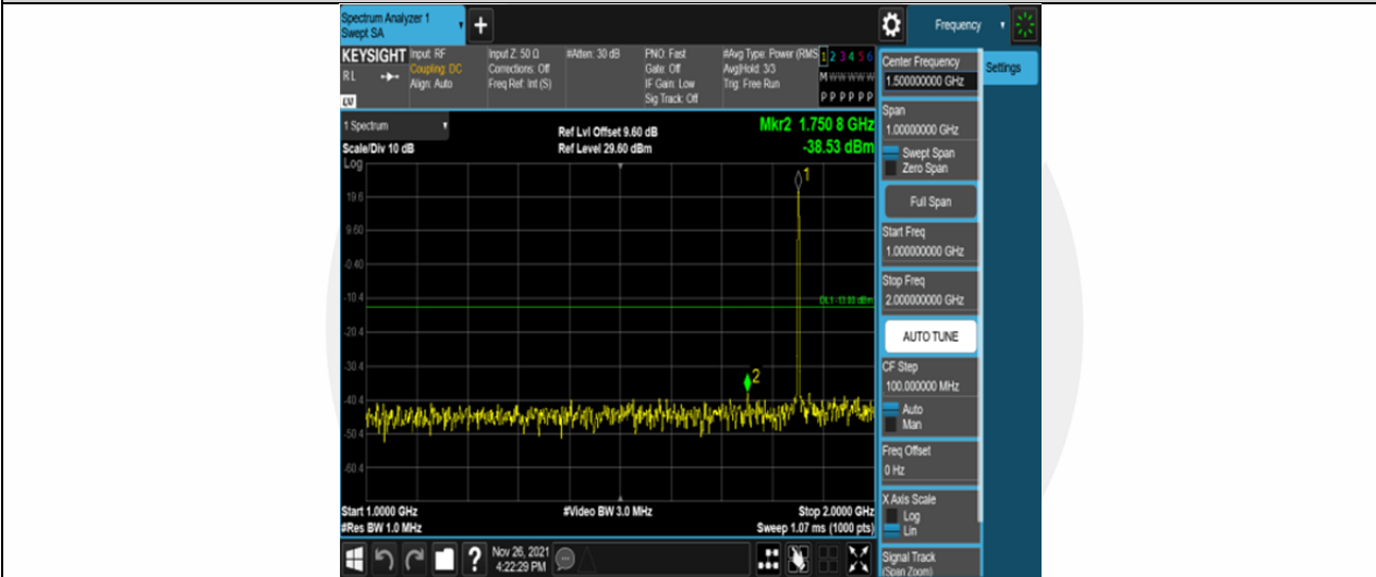
Band25-3MHz-16QAM-26055-1RB#0-Range2:1000~2000MHz
