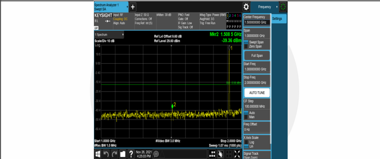
Band25-3MHz-16QAM-26675-1RB#0-Range2:1000~2000MHz
