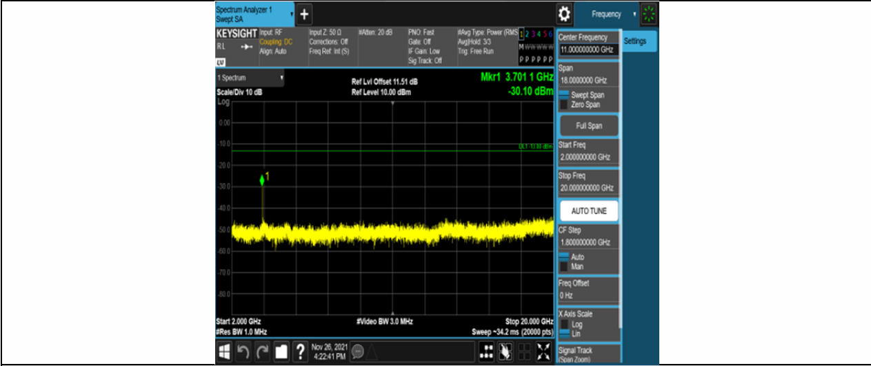
Band25-3MHz-16QAM-26055-1RB#0-Range3:2000~20000MHz
