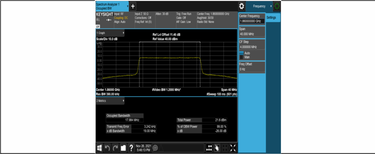
Band25-20MHz-16QAM-26140-100RB#0
