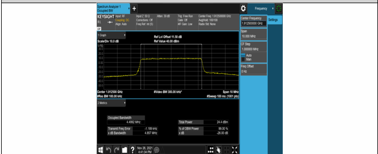
Band25-5MHz-QPSK-26665-25RB#0
