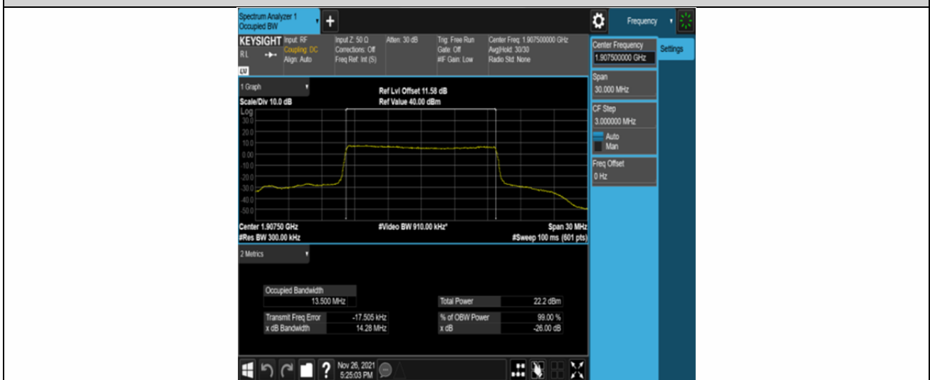
Band25-15MHz-16QAM-26615-75RB#0
