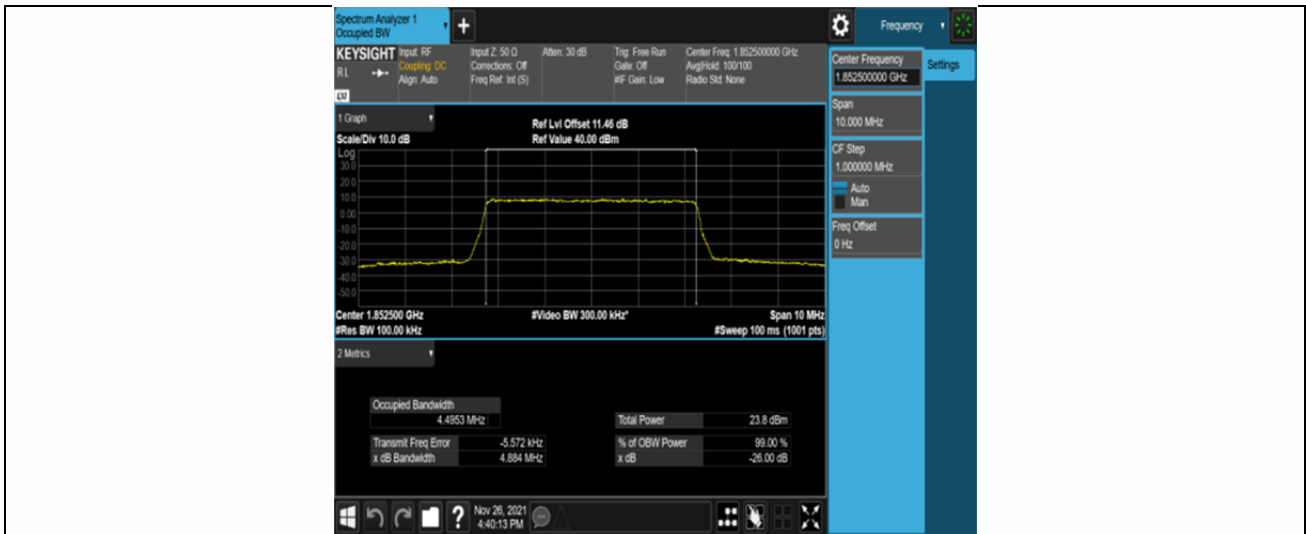
Band25-5MHz-QPSK-26065-25RB#0
