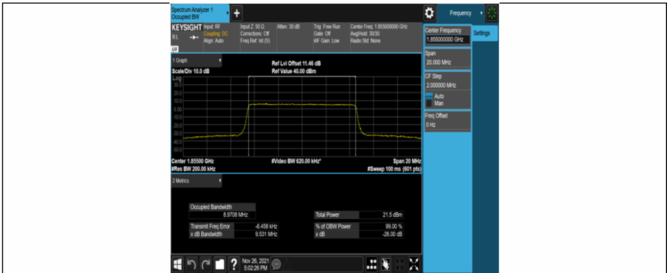
Band 25-10MHz-16QAM-26090-50RB#0
