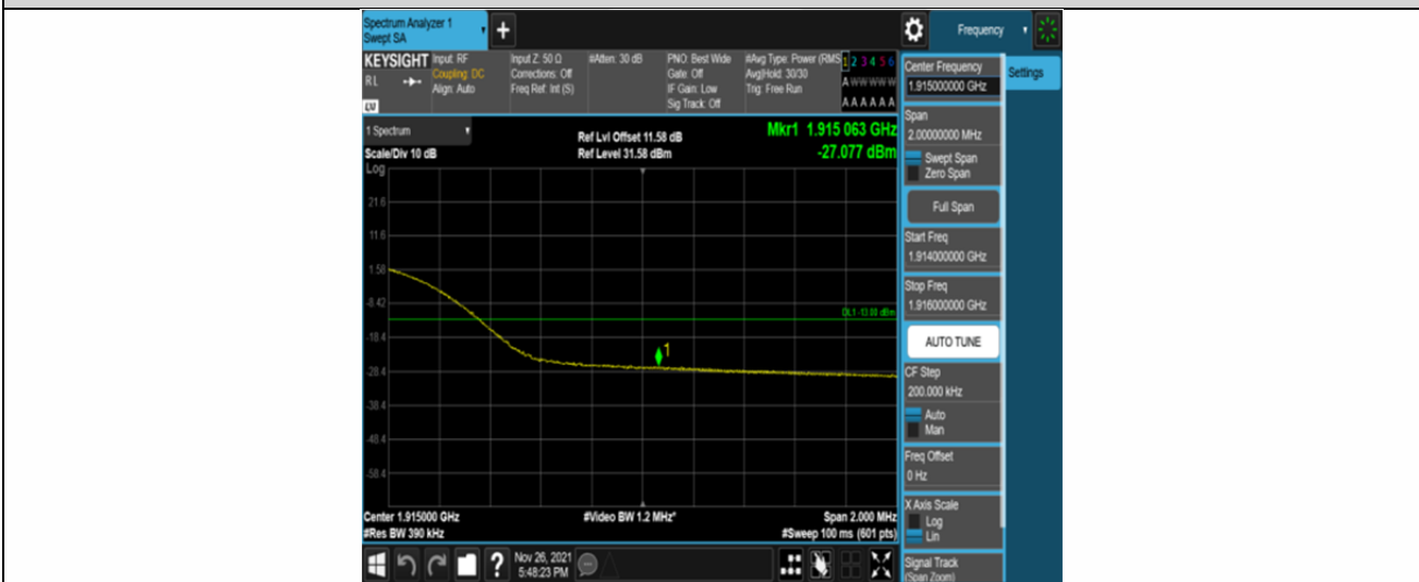
Band25-20MHz-16QAM-26590-100RB#0
