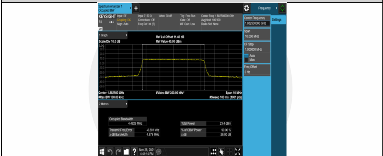
Band25-5MHz-16QAM-26365-25RB#0
