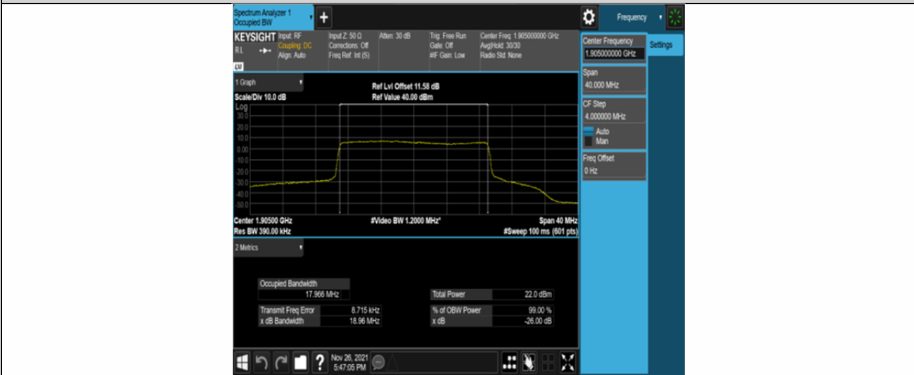
Band25-20MHz-16QAM-26590-100RB#0
