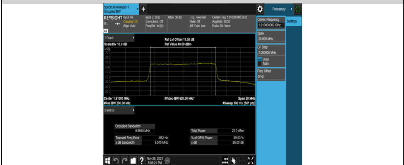
Band 25-10MHz-16QAM-26640-50RB#0
