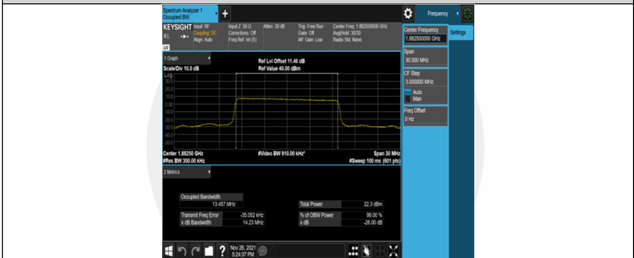
Band25-15MHz-16QAM-26365-75RB#0
