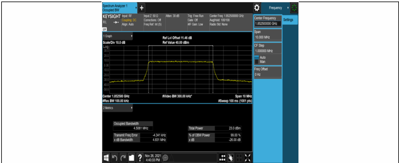
Band25-5MHz-16QAM-26065-25RB#0
