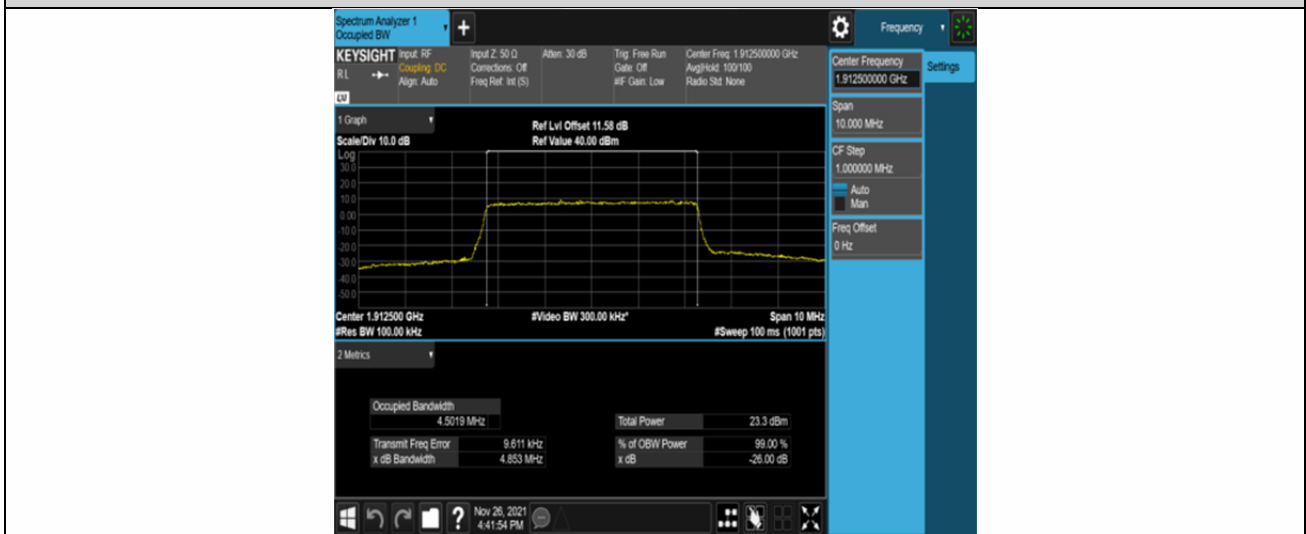
Band25-5MHz-16QAM-26665-25RB#0
