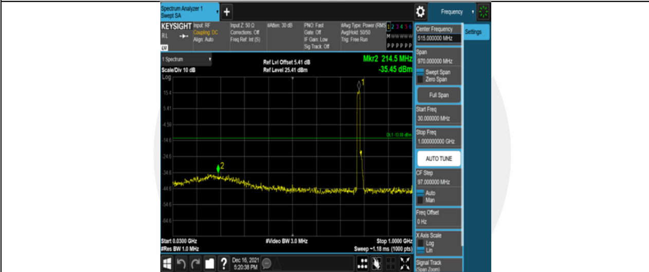
Band13-5MHz-QPSK-23255-25RB#0-Range1:30~1000MHz
