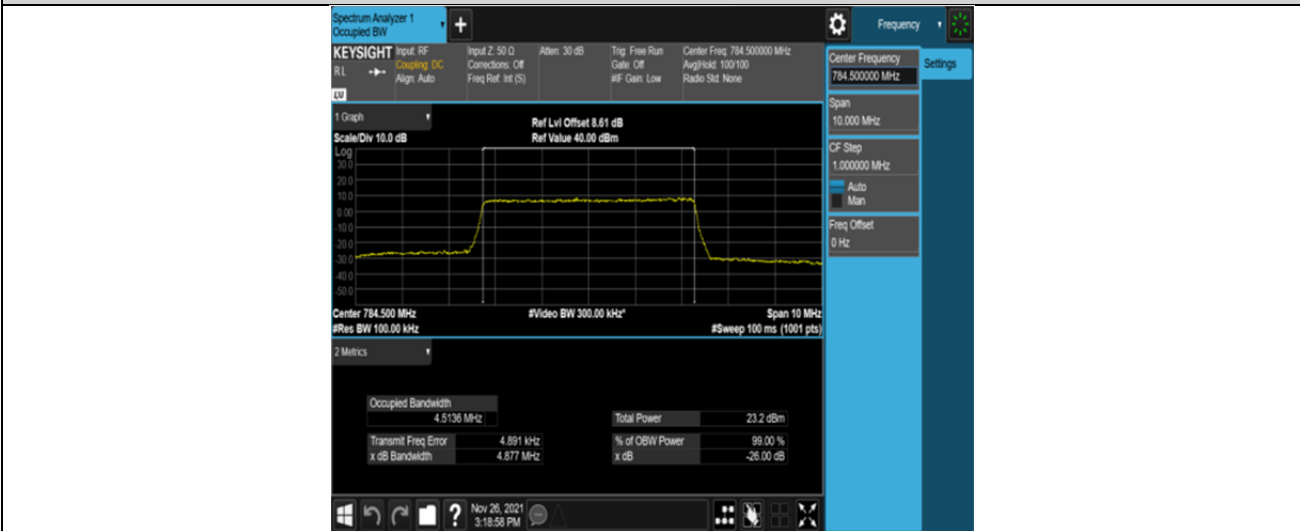
Band13-5MHz-16QAM-23255-25RB#0
