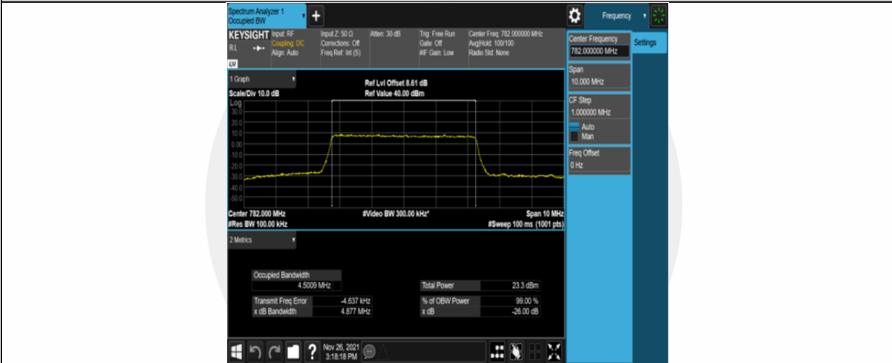
Band13-5MHz-16QAM-23230-25RB#0
