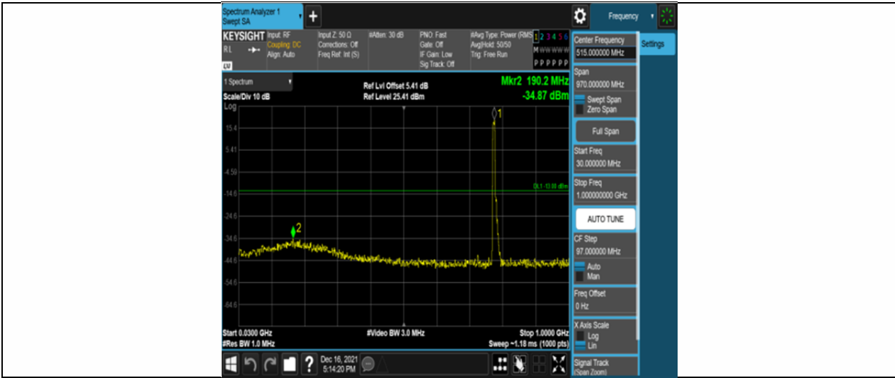
Band13-5MHz-QPSK-23205-25RB#0-Range1:30~1000MHz
