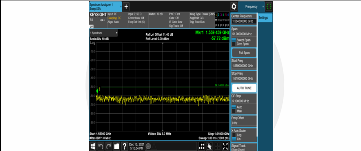
Band13-5MHz-16QAM-23205-25RB#0-Range5:1559~1610MHz
