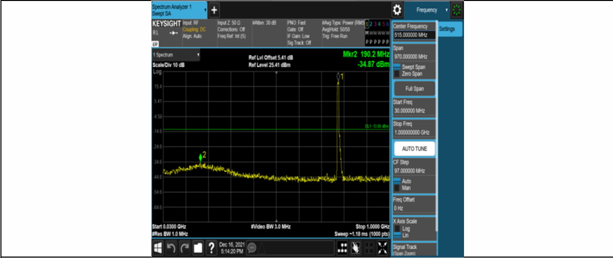
Band13-5MHz-16QAM-23230-25RB#0-Range1:30~1000MHz
