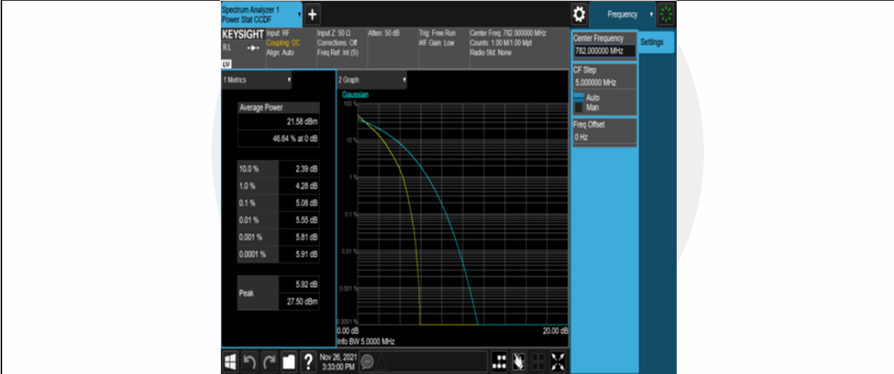
Band13-5MHz-QPSK-23230-25RB#0
