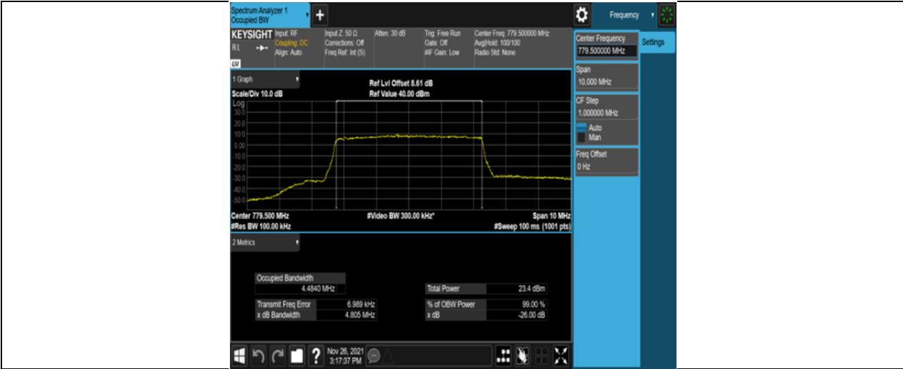
Band13-5MHz-16QAM-23205-25RB#0
