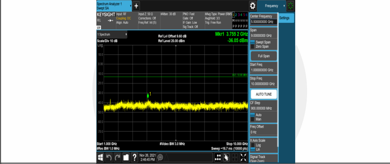
Band12-10MHz-16QAM-23060-50RB#0-Range2:1000~10000MHz
