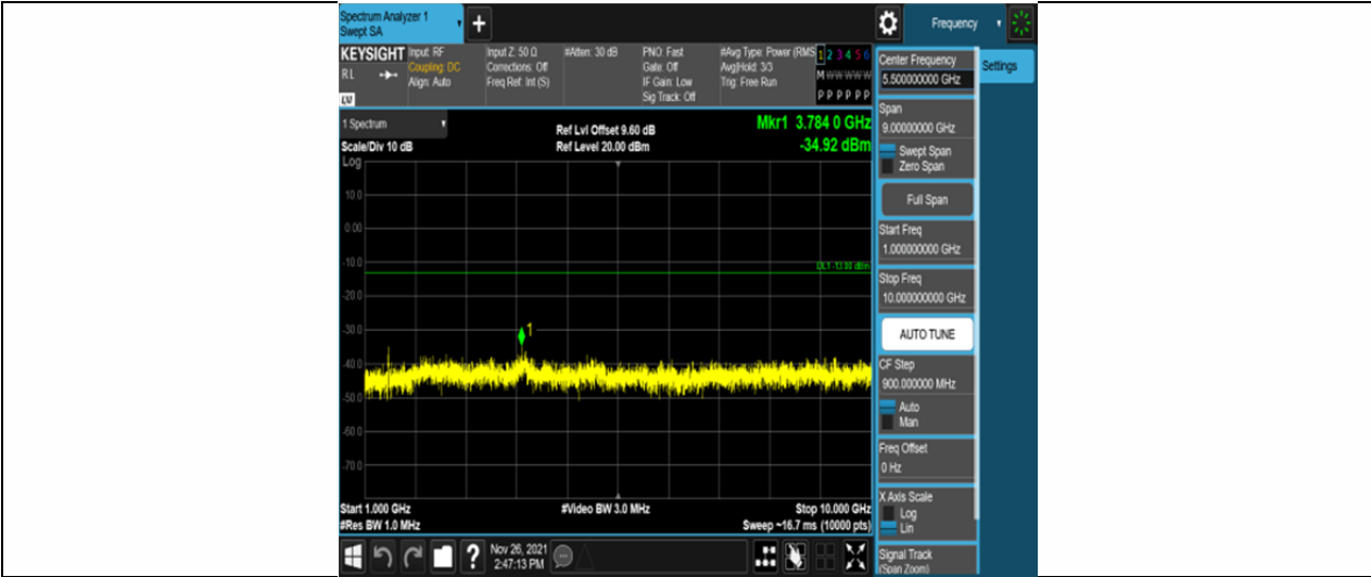
Band12-10MHz-QPSK-23095-50RB#0-Range2:1000~10000MHz
