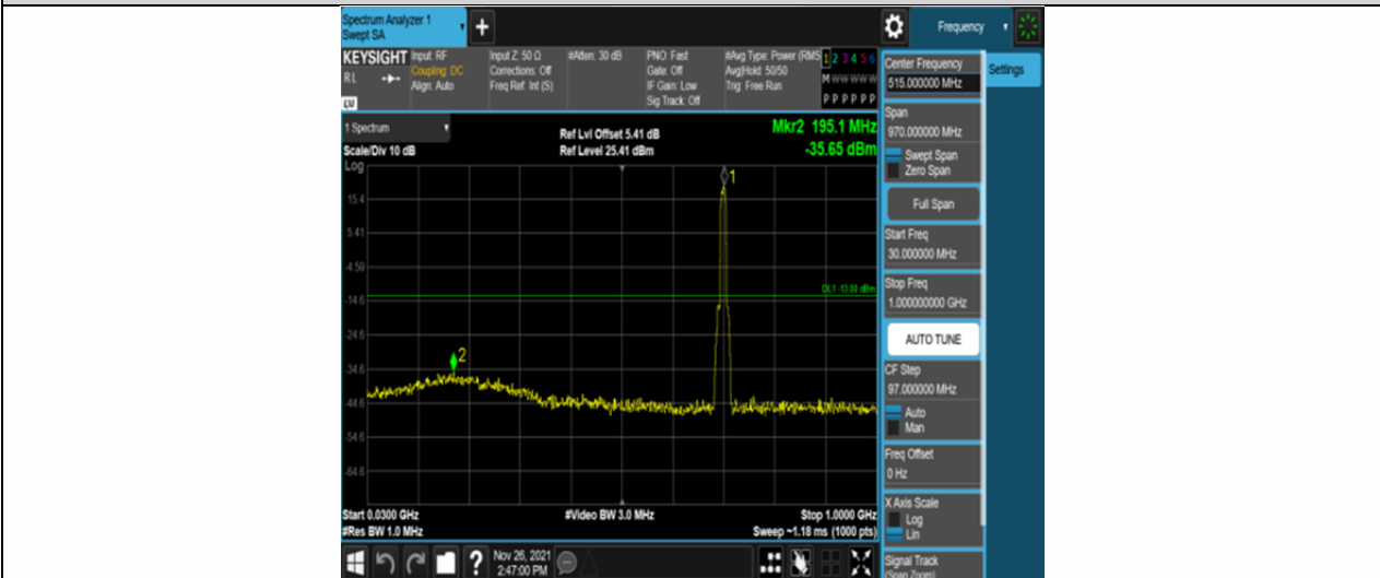
Band12-10MHz-QPSK-23095-50RB#0-Range1:30~1000MHz
