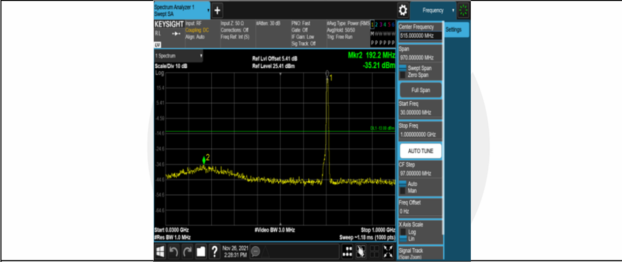
Band12-5MHz-16QAM-23155-25RB#0-Range1:30~1000MHz
