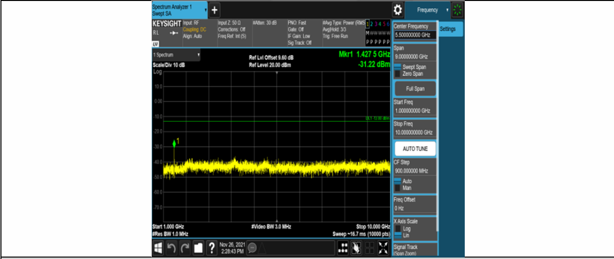
Band12-5MHz-16QAM-23155-25RB#0-Range2:1000~10000MHz
