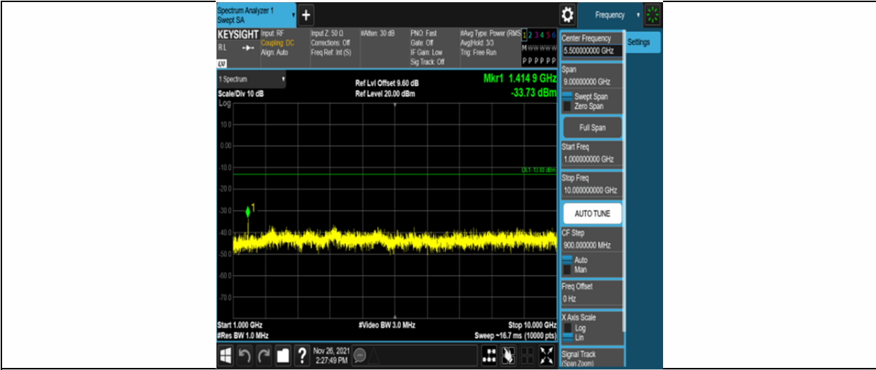
Band12-5MHz-16QAM-23095-25RB#0-Range2:1000~10000MHz
