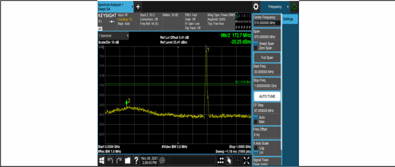
Band12-5MHz-16QAM-23035-25RB#0-Range1:30~1000MHz
