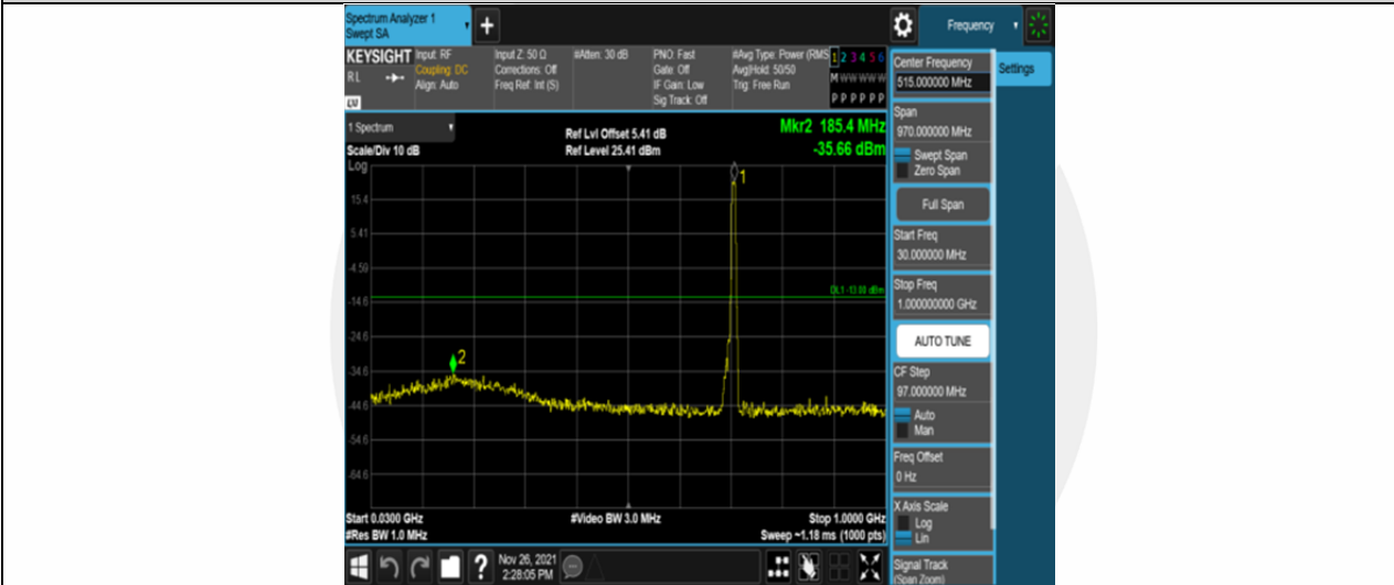
Band12-5MHz-QPSK-23155-25RB#0-Range1:30~1000MHz
