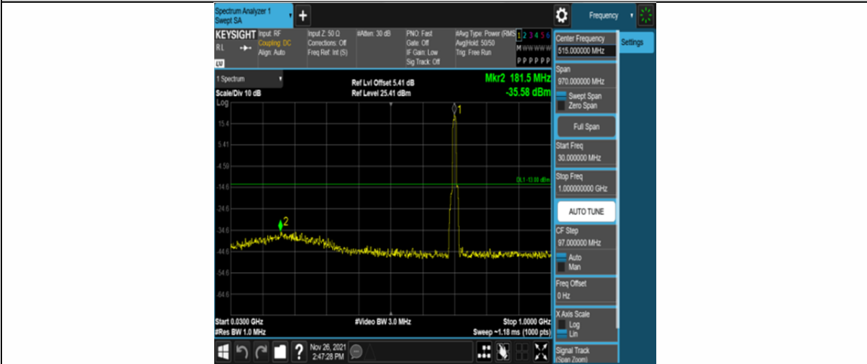
Band12-10MHz-16QAM-23095-50RB#0-Range1:30~1000MHz
