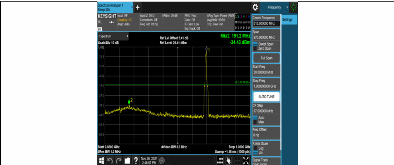
Band12-10MHz-QPSK-23060-50RB#0-Range1:30~1000MHz
