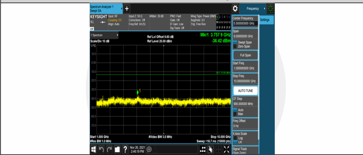
Band12-10MHz-QPSK-23060-50RB#0-Range2:1000~10000MHz
