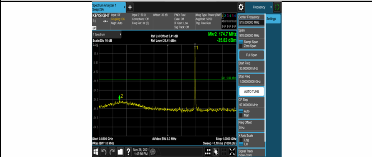
Band12-1.4MHz-16QAM-23095-6RB#0-Range1:30~1000MHz
