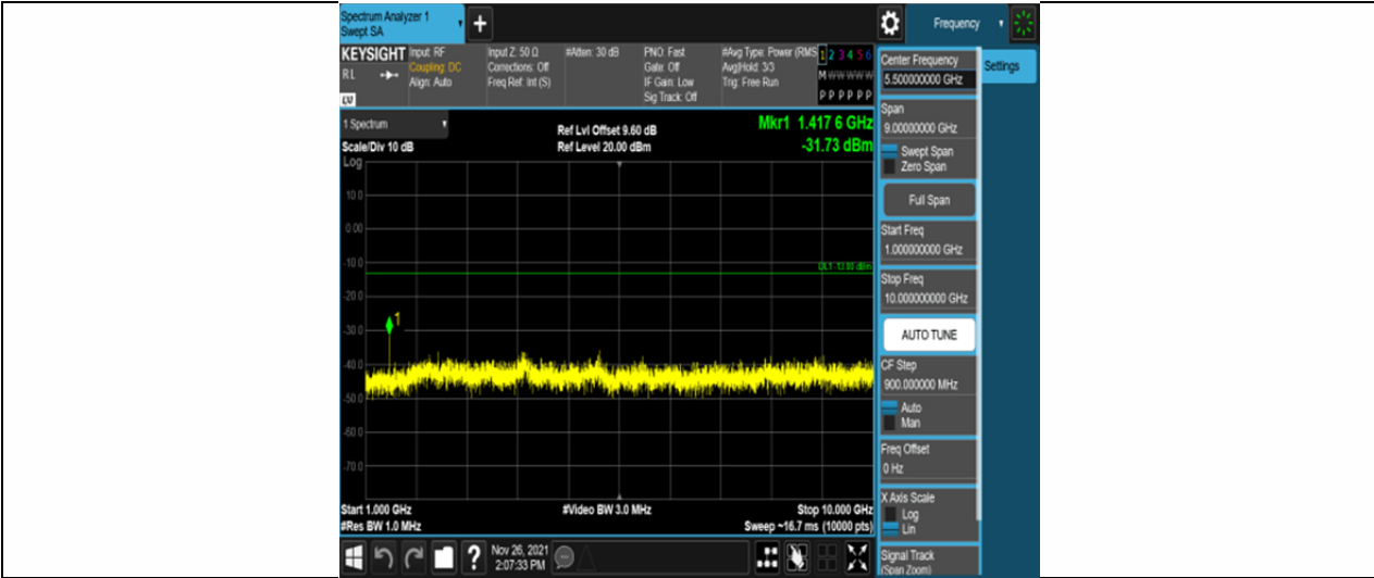
Band12-3MHz-16QAM-23095-15RB#0-Range2:1000~10000MHz
