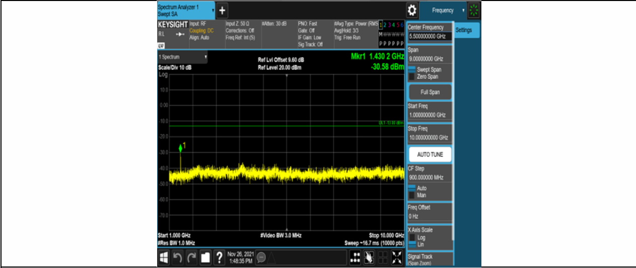
Band12-1.4MHz-QPSK-23173-6RB#0-Range2:1000~10000MHz
