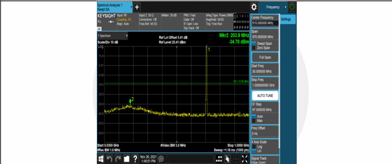
Band12-1.4MHz-16QAM-23173-6RB#0-Range1:30~1000MHz
