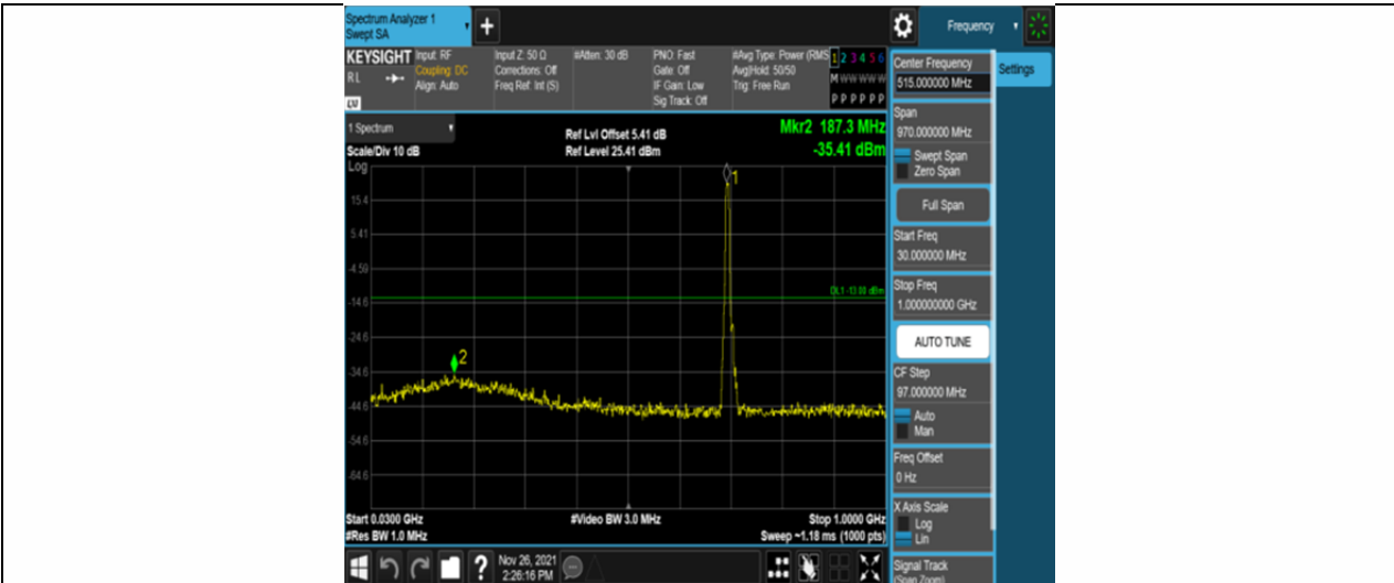
Band12-5MHz-QPSK-23035-25RB#0-Range1:30~1000MHz
