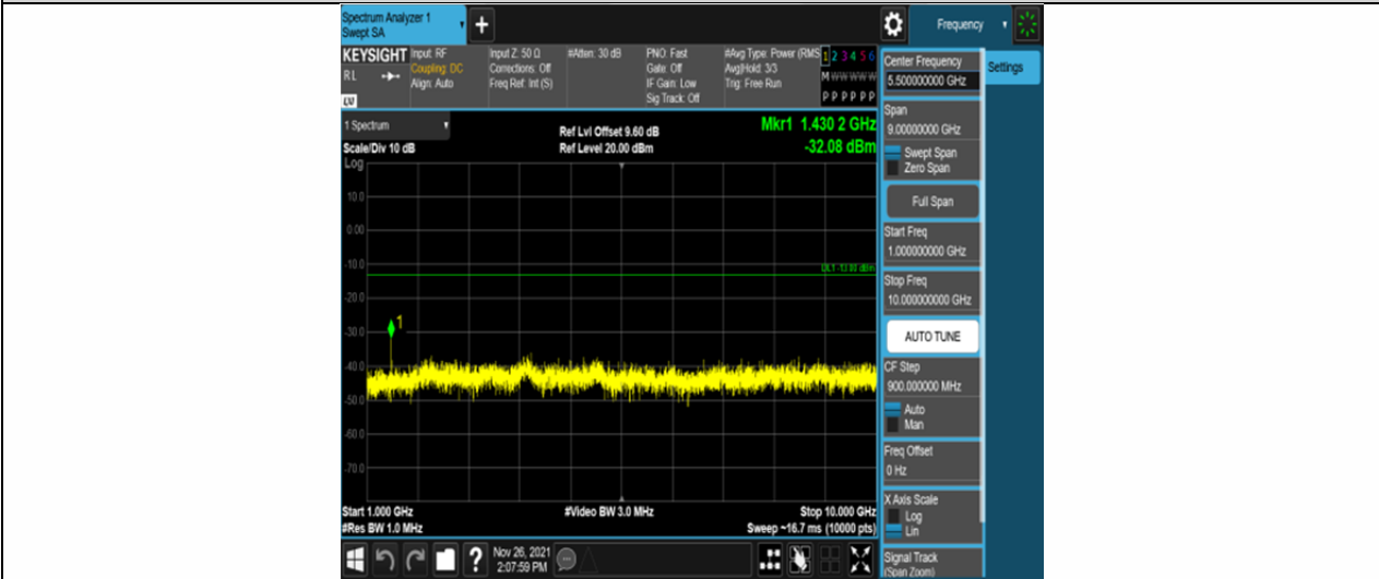
Band12-3MHz-QPSK-23165-15RB#0-Range2:1000~10000MHz
