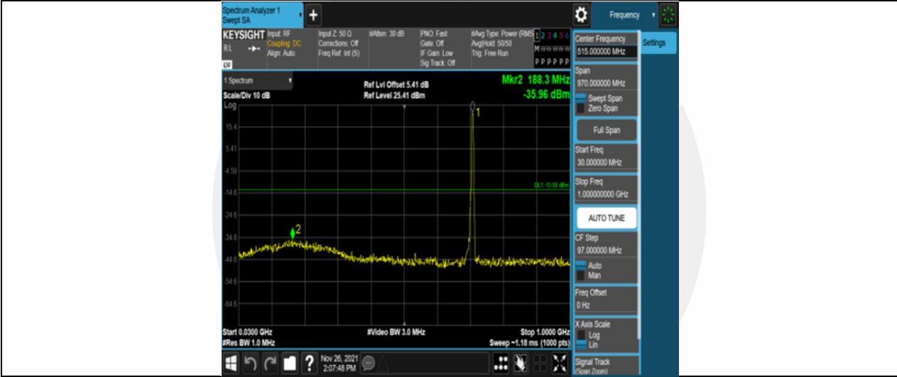
Band12-3MHz-QPSK-23165-15RB#0-Range1:30~1000MHz
