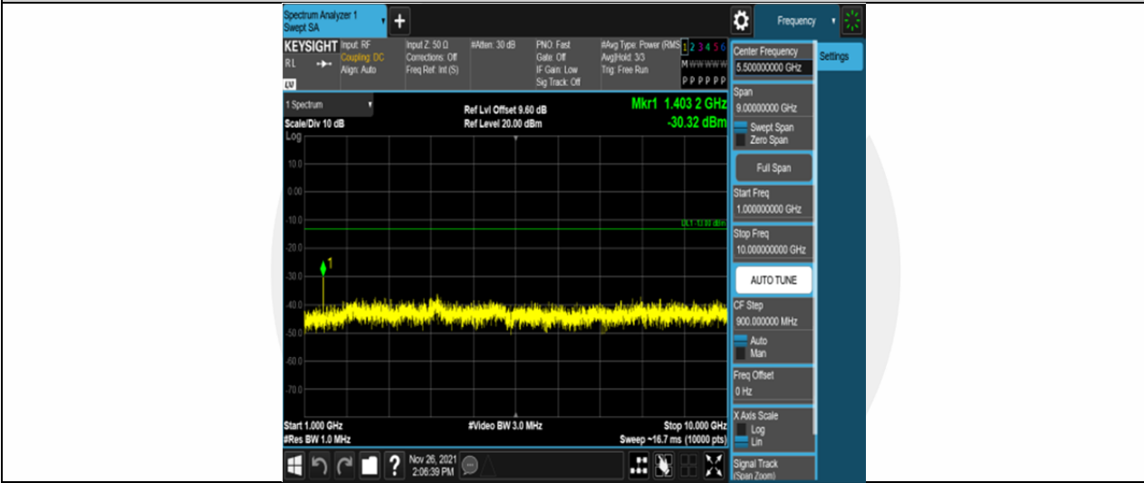
Band12-3MHz-16QAM-23025-15RB#0-Range2:1000~10000MHz
