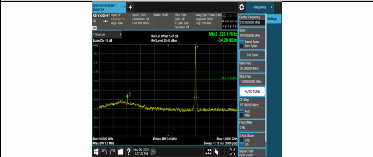
Band12-3MHz-16QAM-23095-15RB#0-Range1:30~1000MHz
