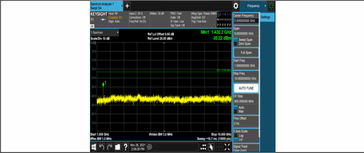
Band12-3MHz-16QAM-23165-15RB#0-Range2:1000~10000MHz
