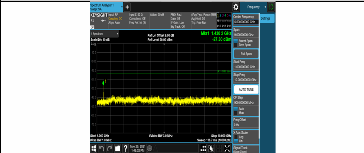
Band12-1.4MHz-16QAM-23173-6RB#0-Range2:1000~10000MHz
