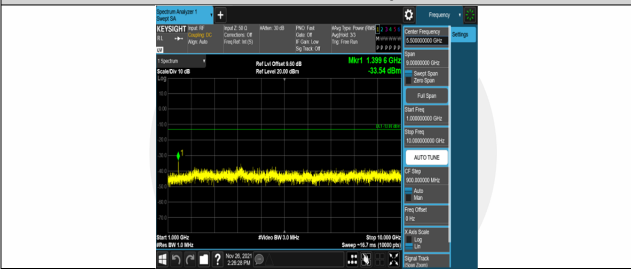
Band12-5MHz-QPSK-23035-25RB#0-Range2:1000~10000MHz
