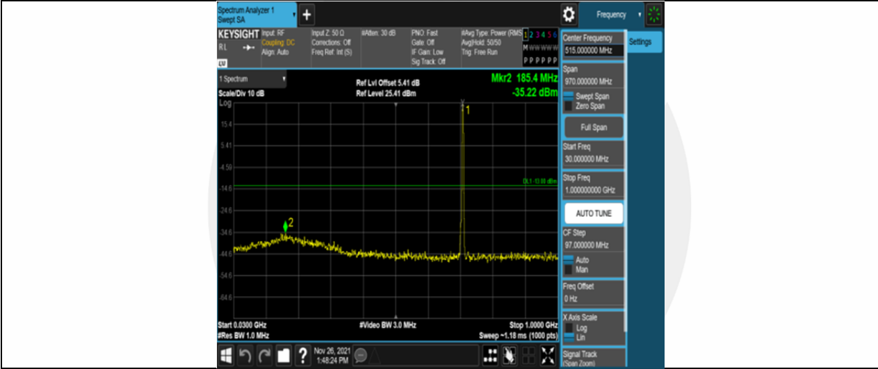
Band12-1.4MHz-QPSK-23173-6RB#0-Range1:30~1000MHz
