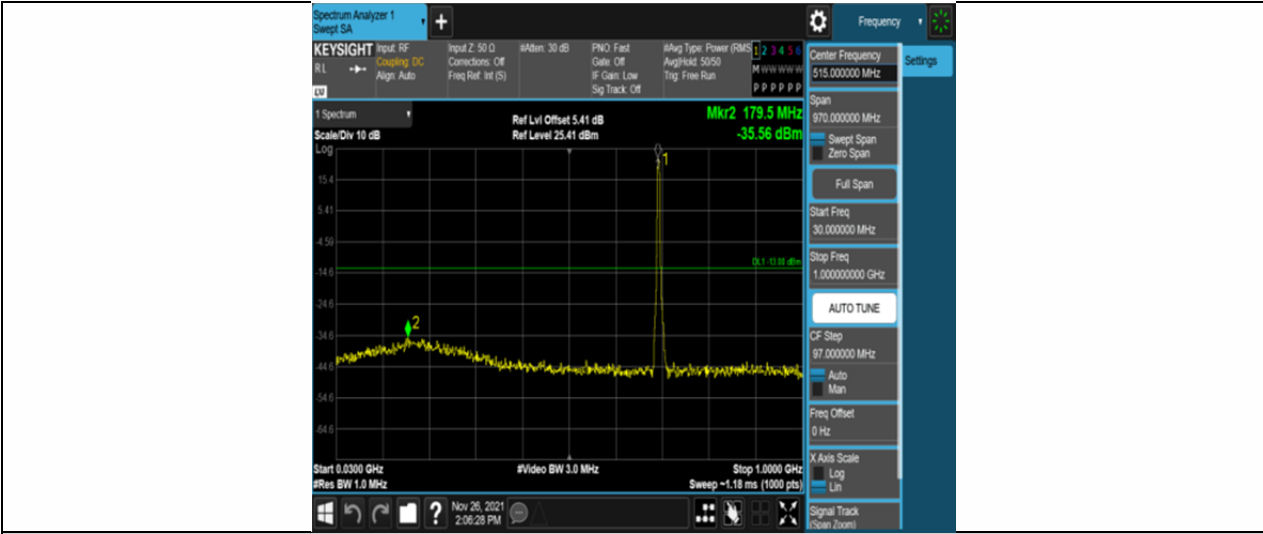
Band12-3MHz-16QAM-23025-15RB#0-Range1:30~1000MHz
