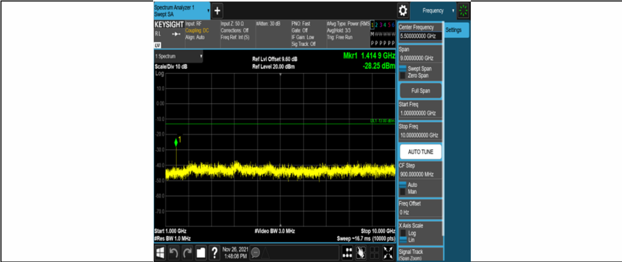
Band12-1.4MHz-16QAM-23095-6RB#0-Range2:1000~10000MHz
