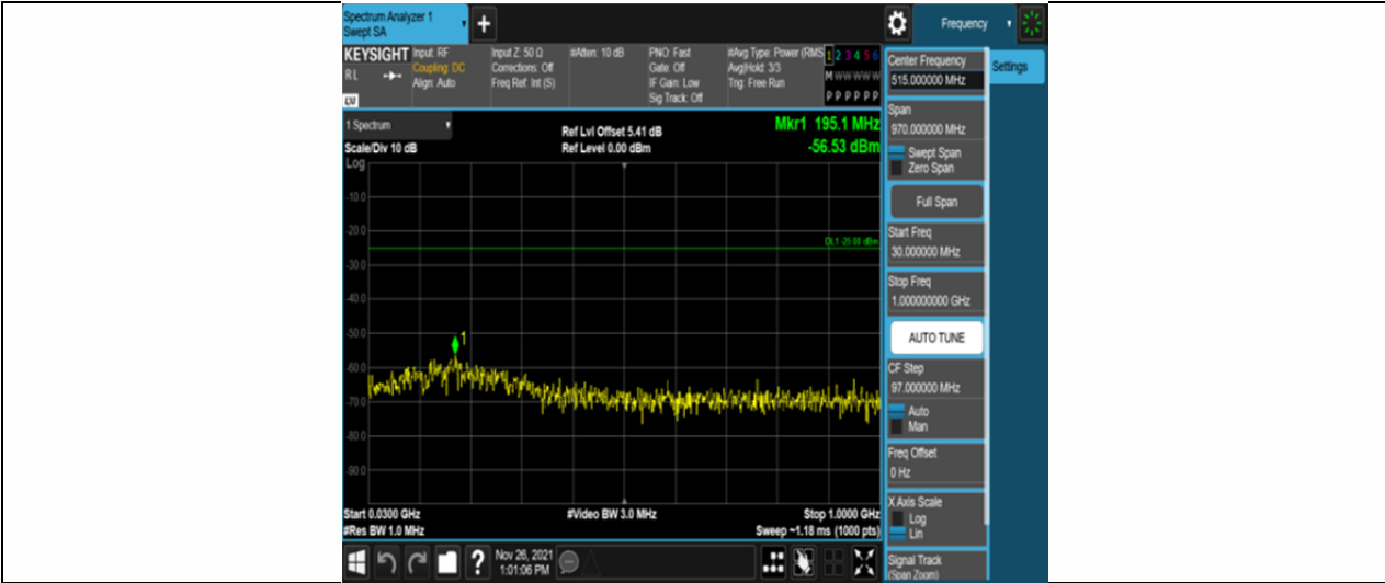
Band7-15MHz-16QAM-20825-75RB#0-Range1:30~1000MHz
