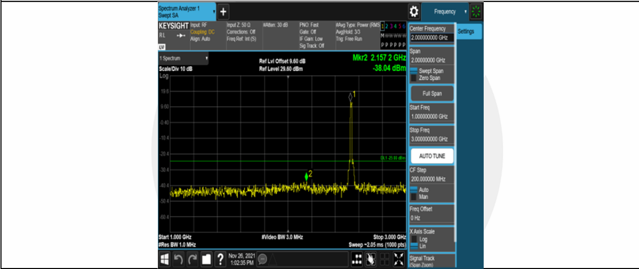
Band7-15MHz-16QAM-21100-75RB#0-Range2:1000~3000MHz
