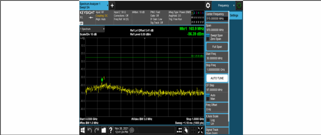
Band7-10MHz-16QAM-21100-50RB#0-Range1:30~1000MHz
