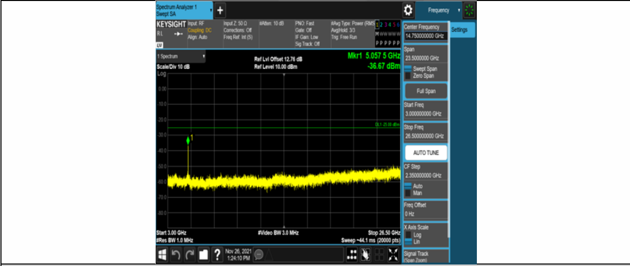
Band7-20MHz-16QAM-21100-100RB#0-Range3:3000~26500MHz
