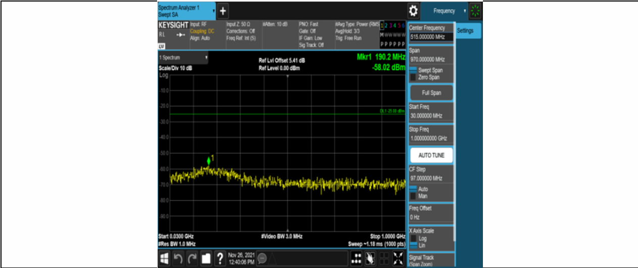
Band7-10MHz-16QAM-20800-50RB#0-Range1:30~1000MHz
