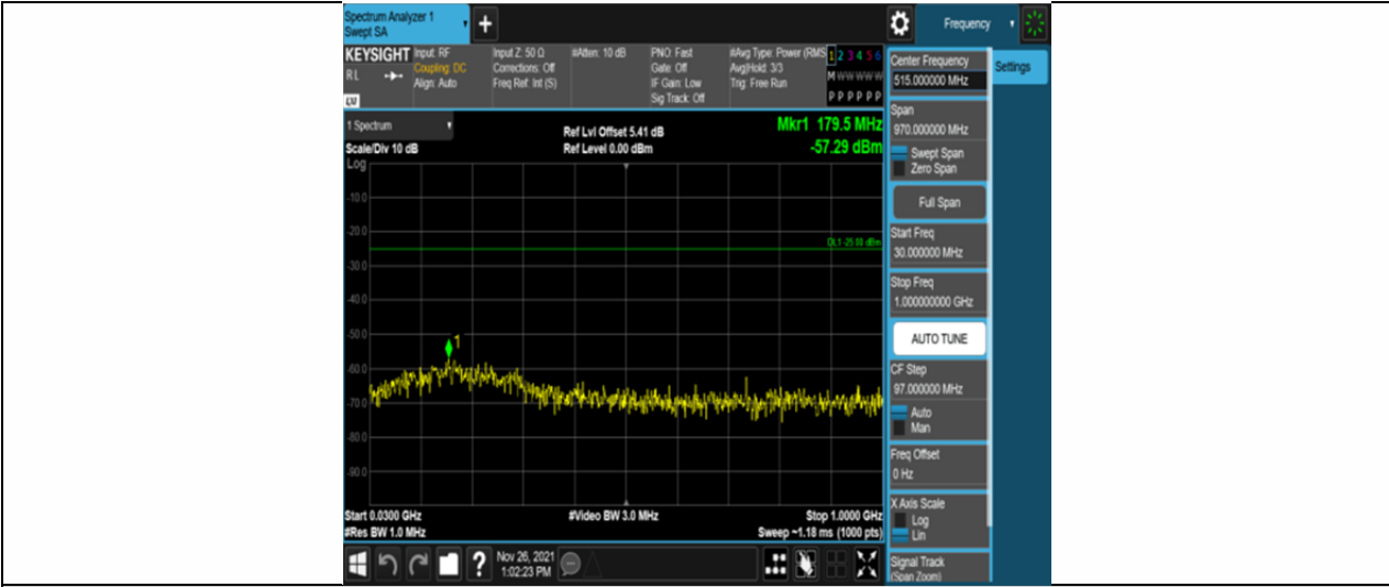
Band7-15MHz-16QAM-21100-75RB#0-Range1:30~1000MHz
