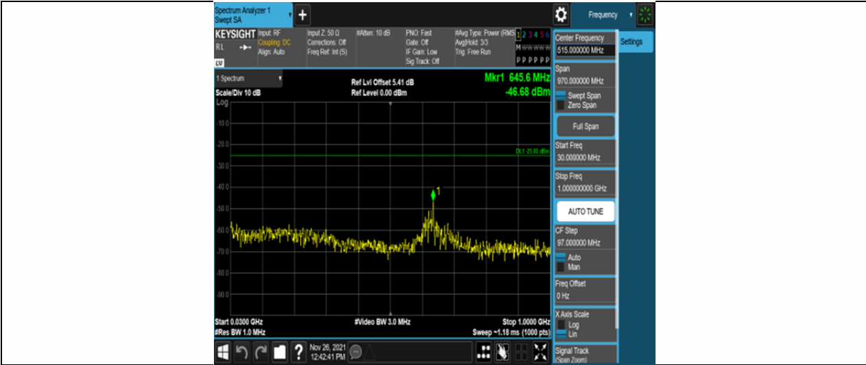
Band7-10MHz-16QAM-21400-50RB#0-Range1:30~1000MHz
