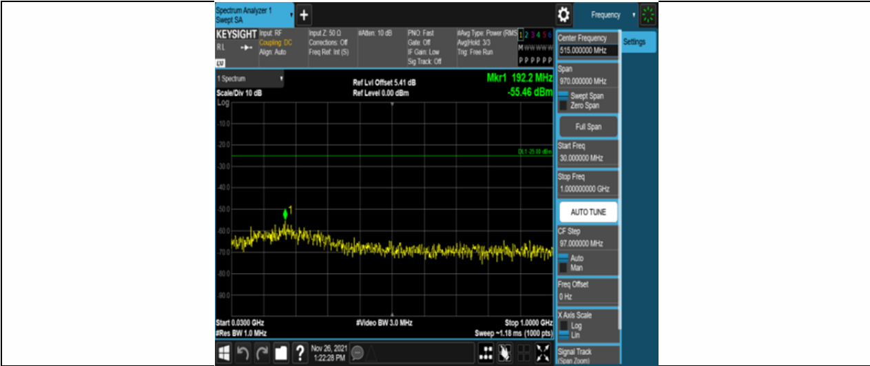
Band7-20MHz-16QAM-20850-100RB#0-Range1:30~1000MHz
