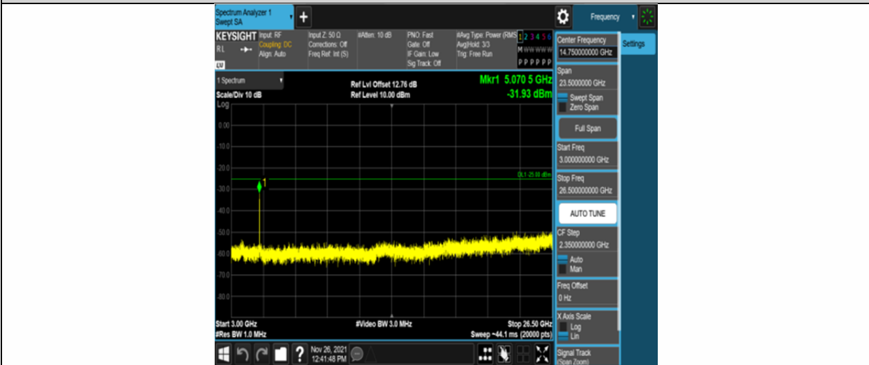
Band7-10MHz-16QAM-21100-50RB#0-Range3:3000~26500MHz
