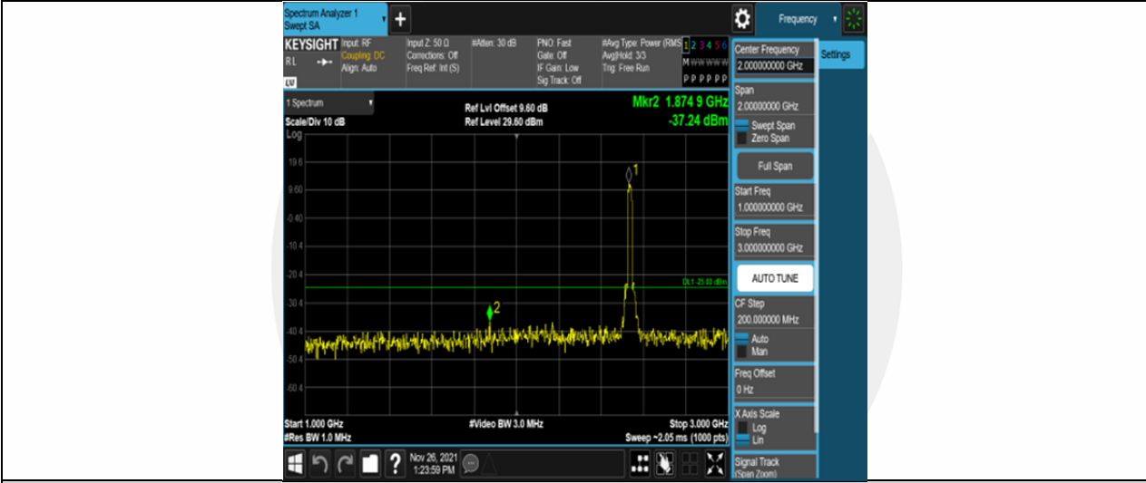
Band7-20MHz-16QAM-21100-100RB#0-Range2:1000~3000MHz
