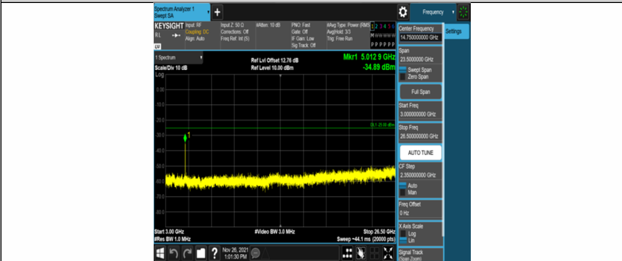
Band7-15MHz-16QAM-20825-75RB#0-Range3:3000~26500MHz
