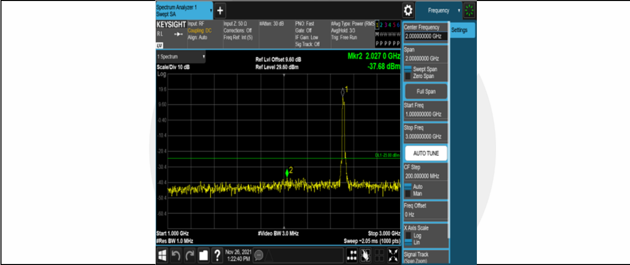
Band7-20MHz-16QAM-20850-100RB#0-Range2:1000~3000MHz
