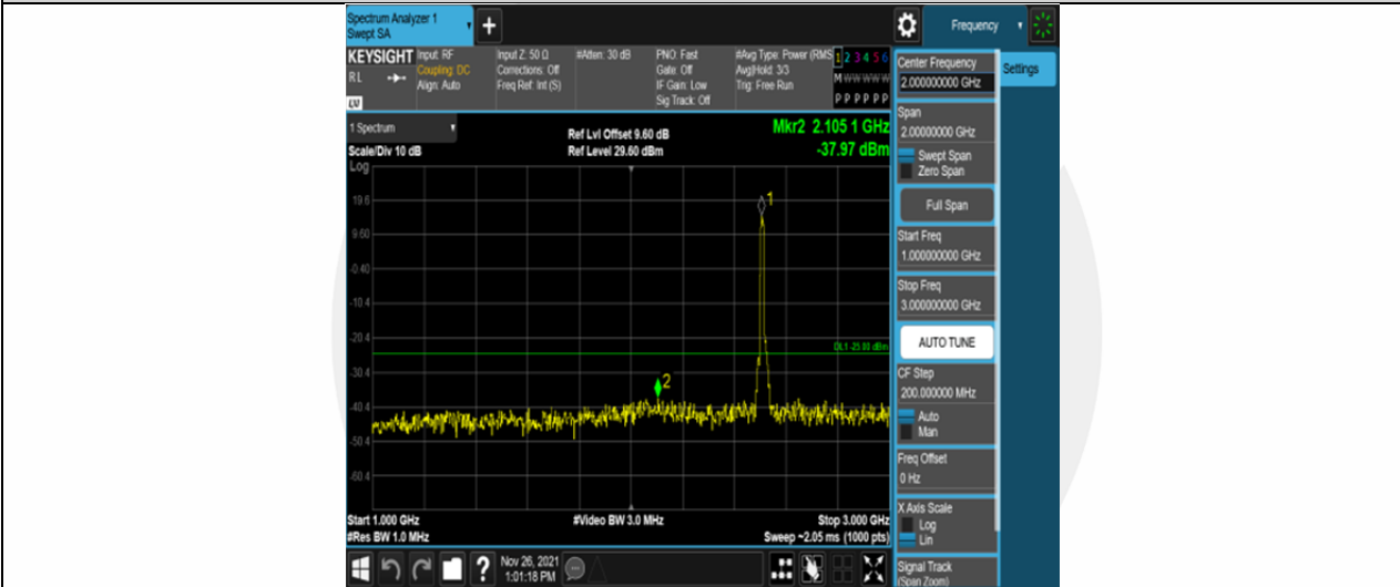
Band7-15MHz-16QAM-20825-75RB#0-Range2:1000~3000MHz
