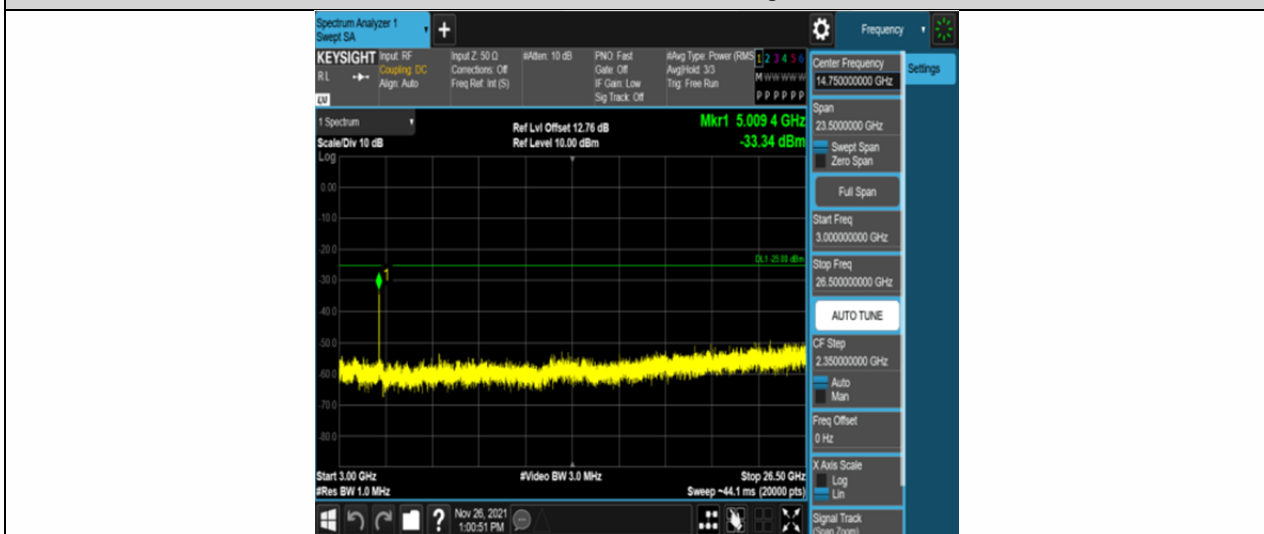
Band7-15MHz-QPSK-20825-75RB#0-Range3:3000~26500MHz
