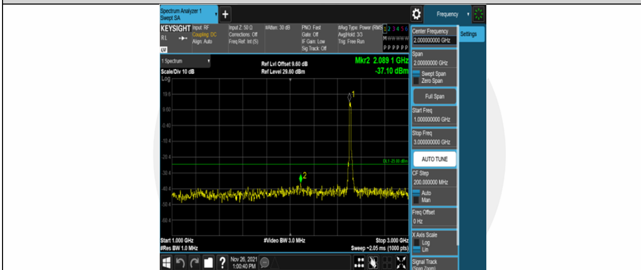
Band7-15MHz-QPSK-20825-75RB#0-Range2:1000~3000MHz
