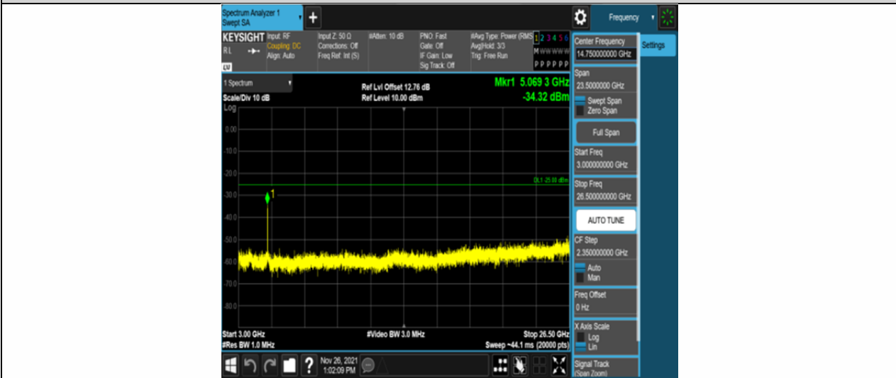
Band7-15MHz-QPSK-21100-75RB#0-Range3:3000~26500MHz
