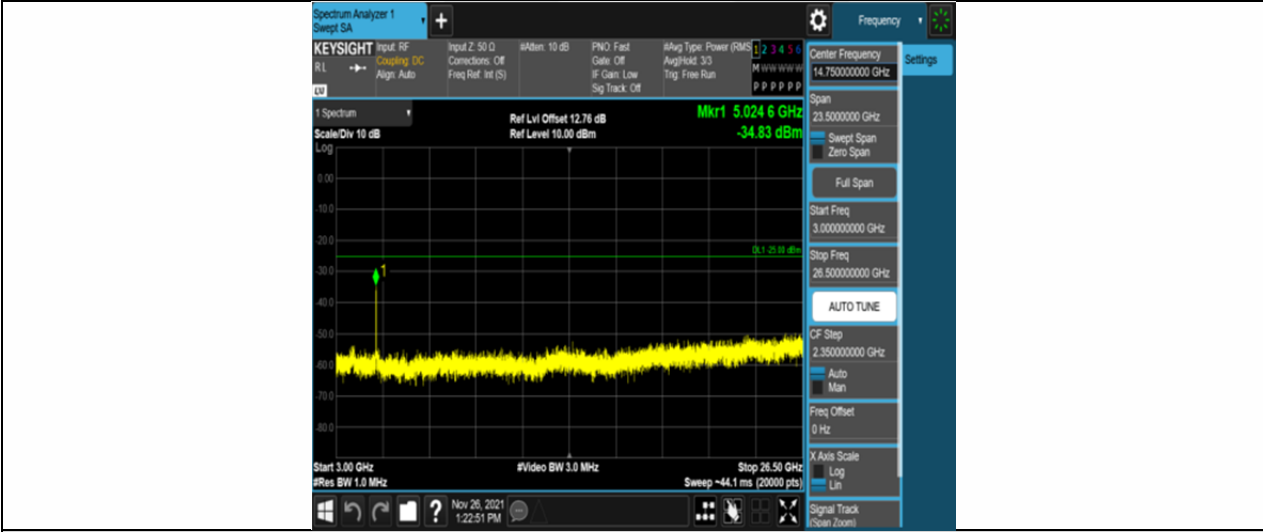
Band7-20MHz-16QAM-20850-100RB#0-Range3:3000~26500MHz
