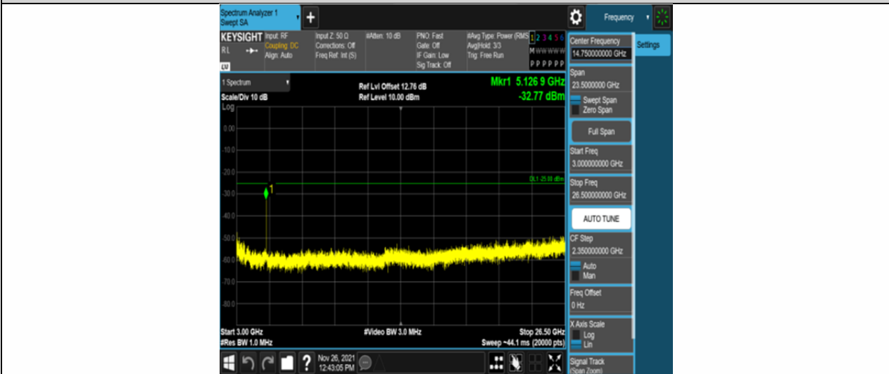
Band7-10MHz-16QAM-21400-50RB#0-Range3:3000~26500MHz
