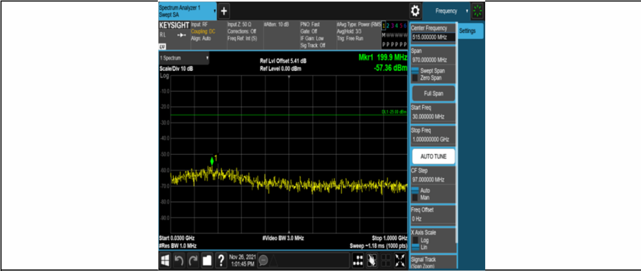
Band7-15MHz-QPSK-21100-75RB#0-Range1:30~1000MHz
