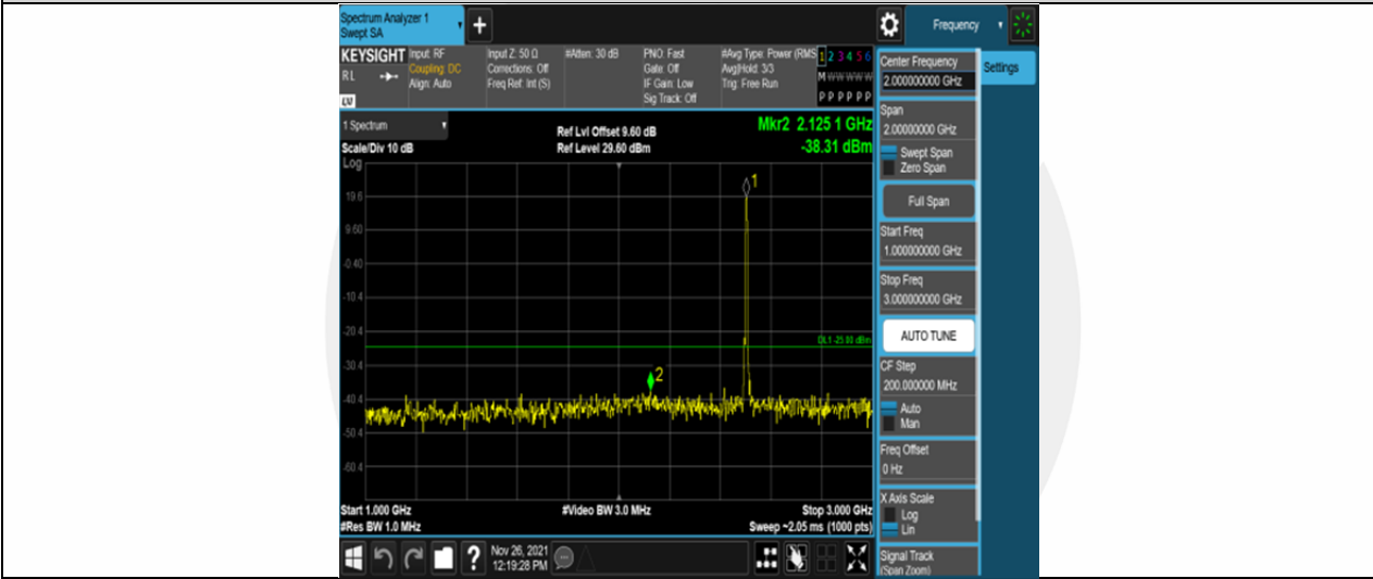
Band7-5MHz-16QAM-20775-25RB#0-Range2:1000~3000MHz
