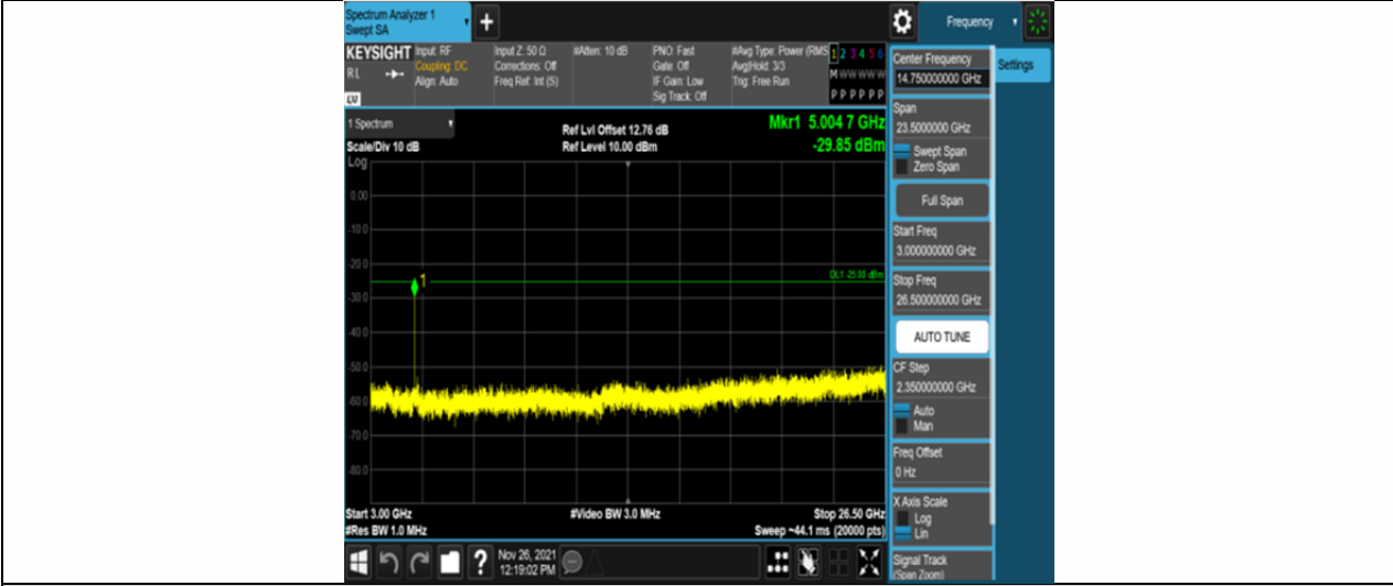
Band7-5MHz-QPSK-20775-25RB#0-Range3:3000~26500MHz
