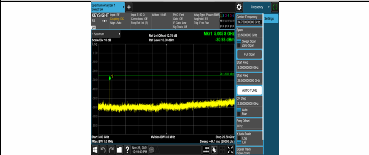
Band7-5MHz-16QAM-20775-25RB#0-Range3:3000~26500MHz
