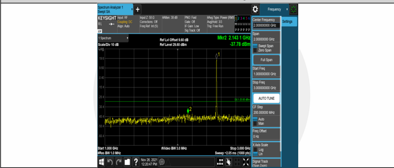
Band7-5MHz-16QAM-21100-25RB#0-Range2:1000~3000MHz
