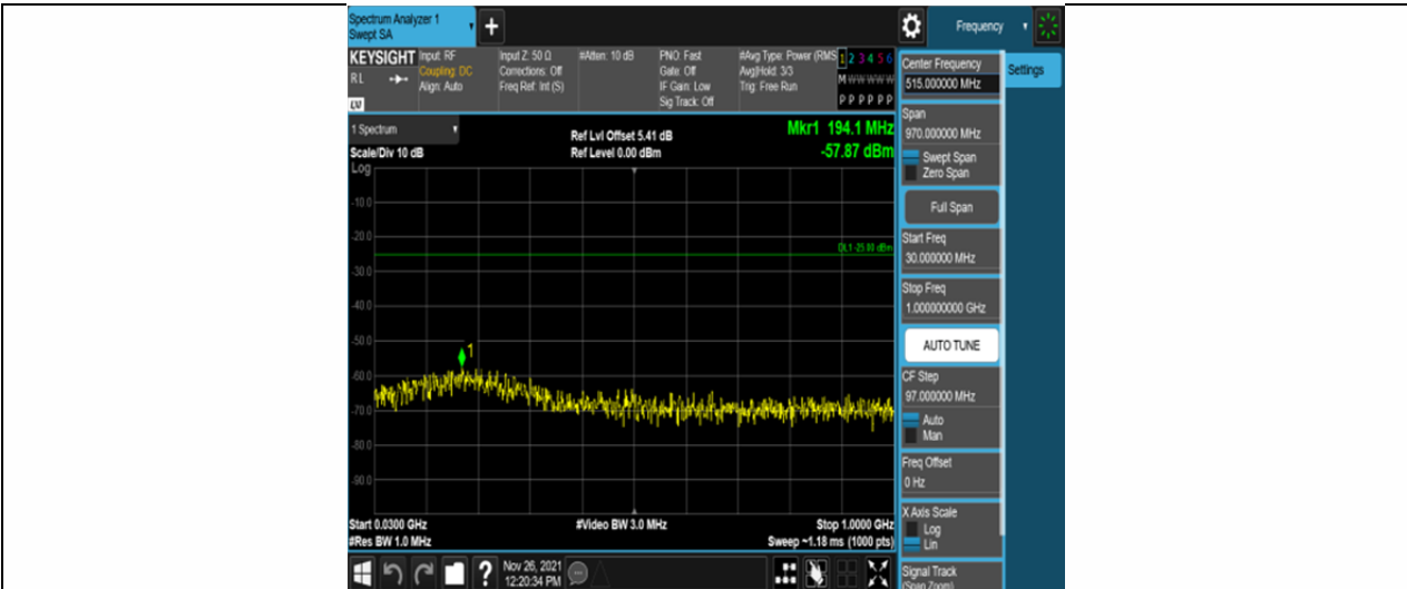
Band7-5MHz-16QAM-21100-25RB#0-Range1:30~1000MHz
