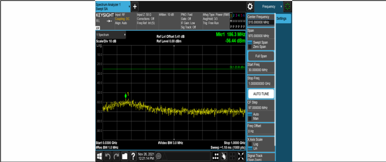
Band7-5MHz-QPSK-21425-25RB#0-Range1:30~1000MHz
