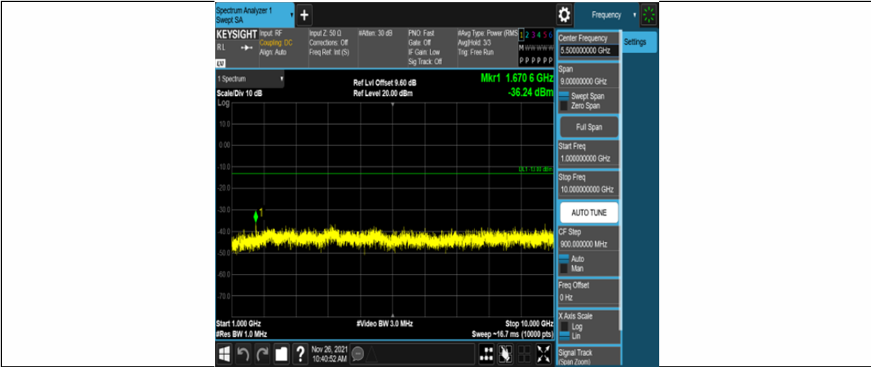
Band5-5MHz-QPSK-20525-25RB#0-Range2:1000~10000MHz
