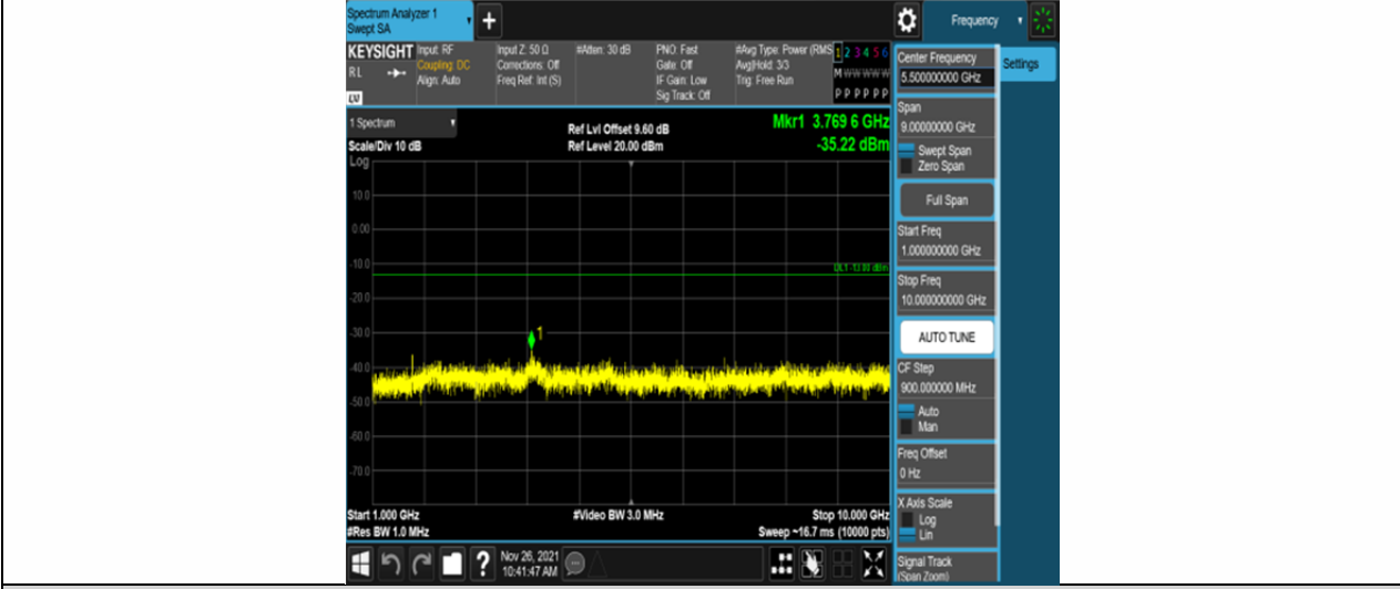
Band5-5MHz-QPSK-20625-25RB#0-Range2:1000~10000MHz
