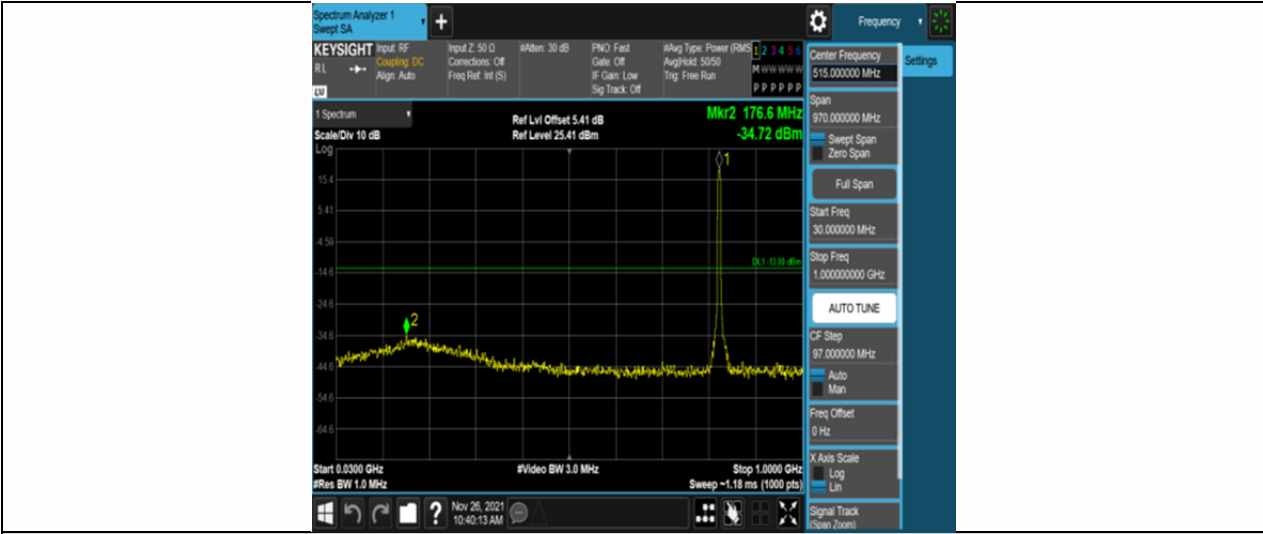
Band5-5MHz-16QAM-20425-25RB#0-Range1:30~1000MHz
