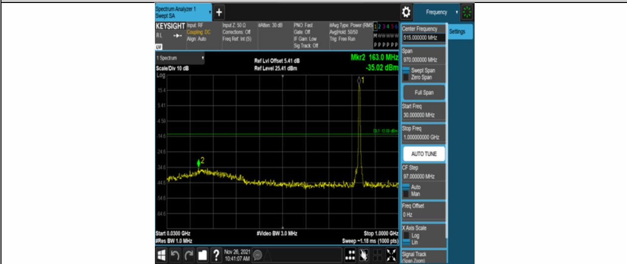
Band5-5MHz-16QAM-20525-25RB#0-Range1:30~1000MHz
