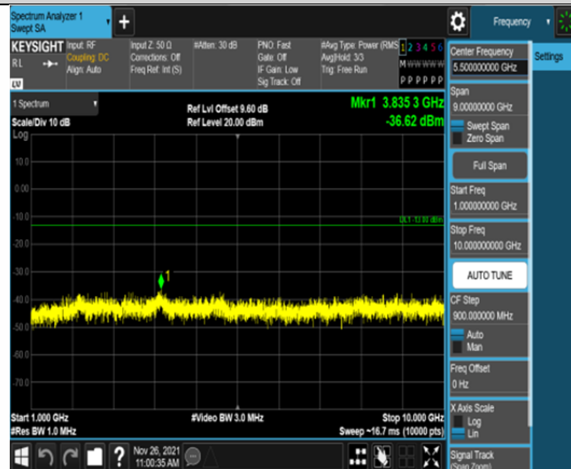
Band5-10MHz-16QAM-20600-50RB#0-Range2:1000~10000MHz
