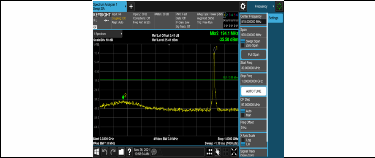
Band5-10MHz-16QAM-20450-50RB#0-Range1:30~1000MHz
