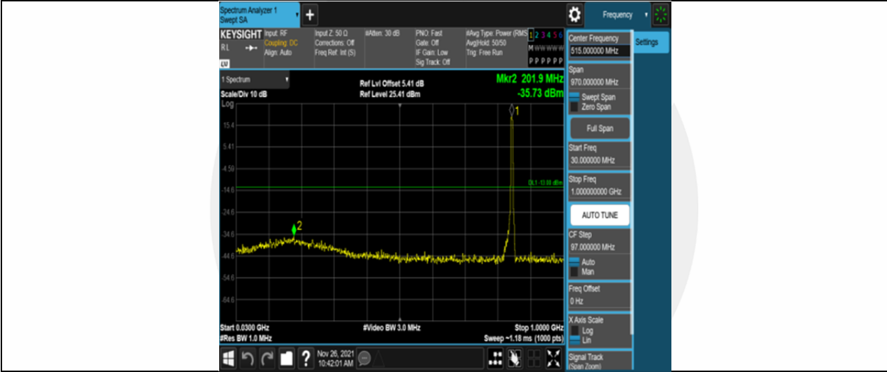
Band5-5MHz-16QAM-20625-25RB#0-Range1:30~1000MHz
