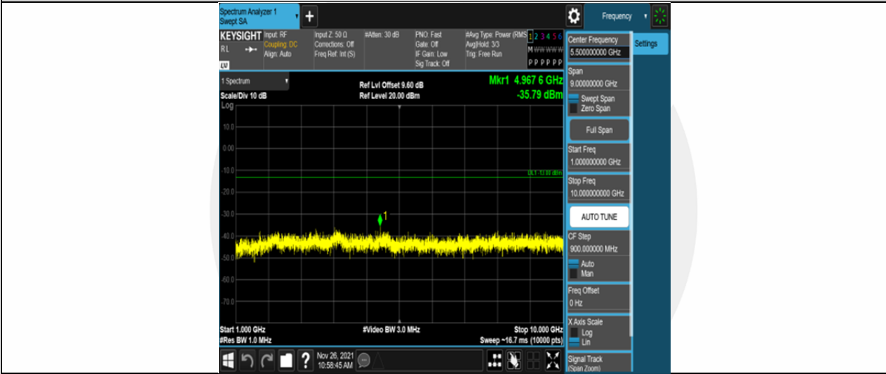
Band5-10MHz-16QAM-20450-50RB#0-Range2:1000~10000MHz
