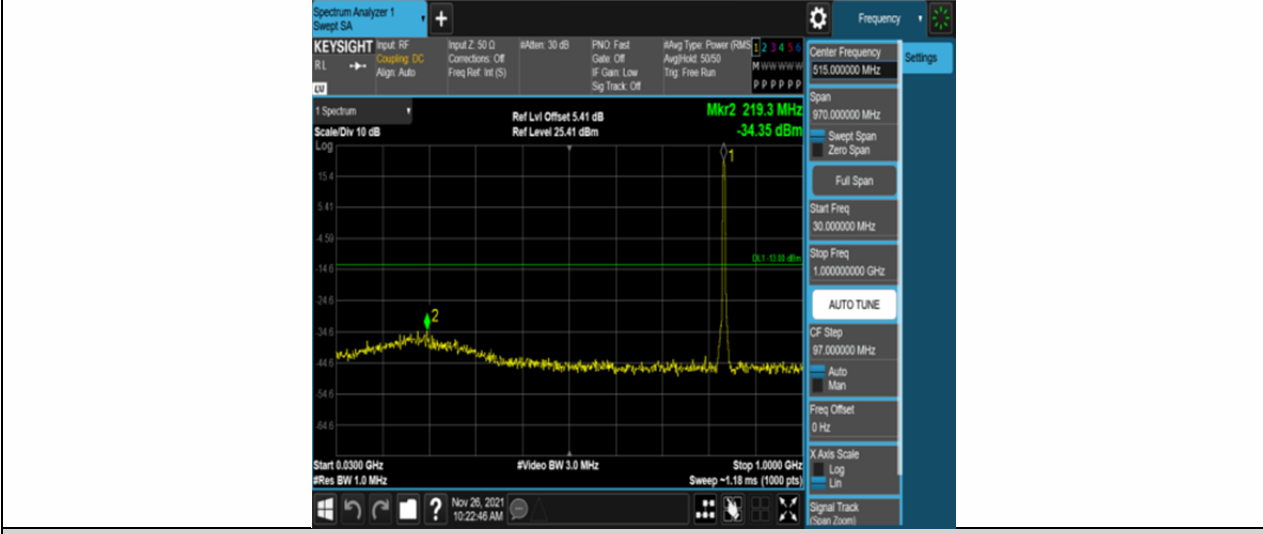
Band5-3MHz-16QAM-20525-15RB#0-Range1:30~1000MHz
