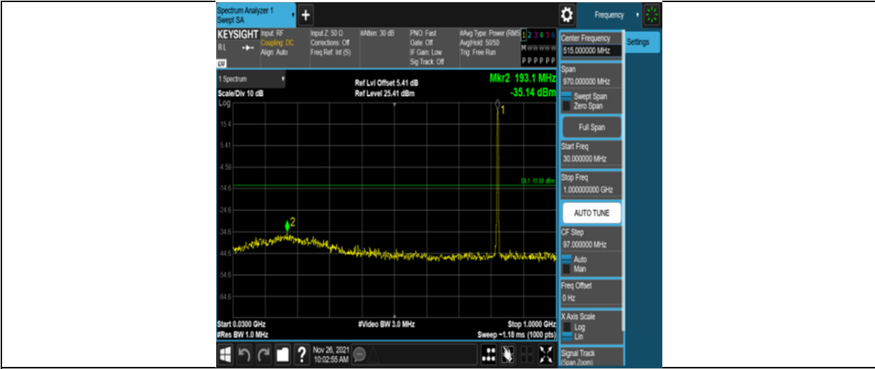
Band5-1.4MHz-16QAM-20407-6RB#0-Range1:30~1000MHz
