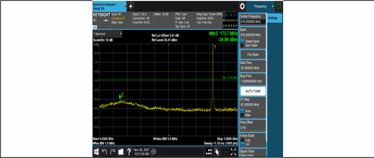
Band5-3MHz-16QAM-20415-15RB#0-Range1:30~1000MHz
