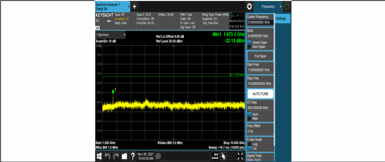
Band5-1.4MHz-16QAM-20525-6RB#0-Range2:1000~10000MHz
