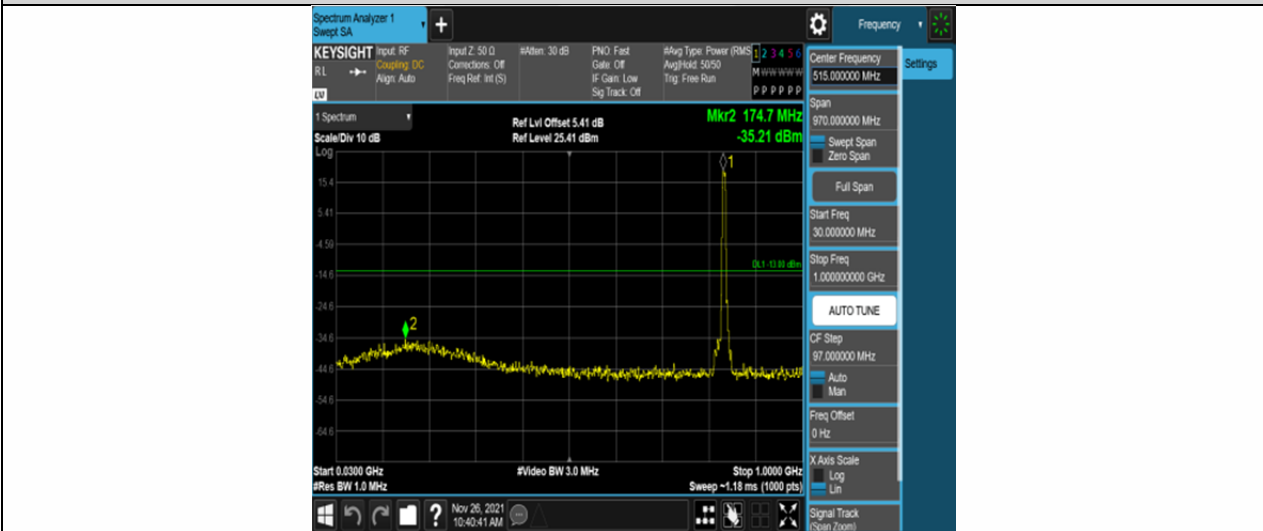
Band5-5MHz-QPSK-20525-25RB#0-Range1:30~1000MHz
