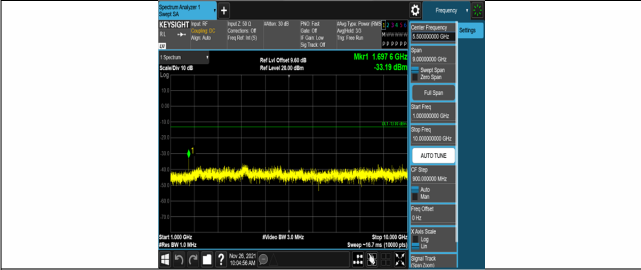
Band5-1.4MHz-16QAM-20643-6RB#0-Range2:1000~10000MHz
