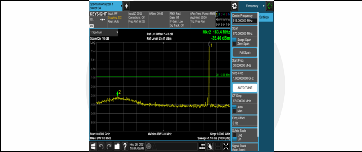
Band5-1.4MHz-16QAM-20643-6RB#0-Range1:30~1000MHz
