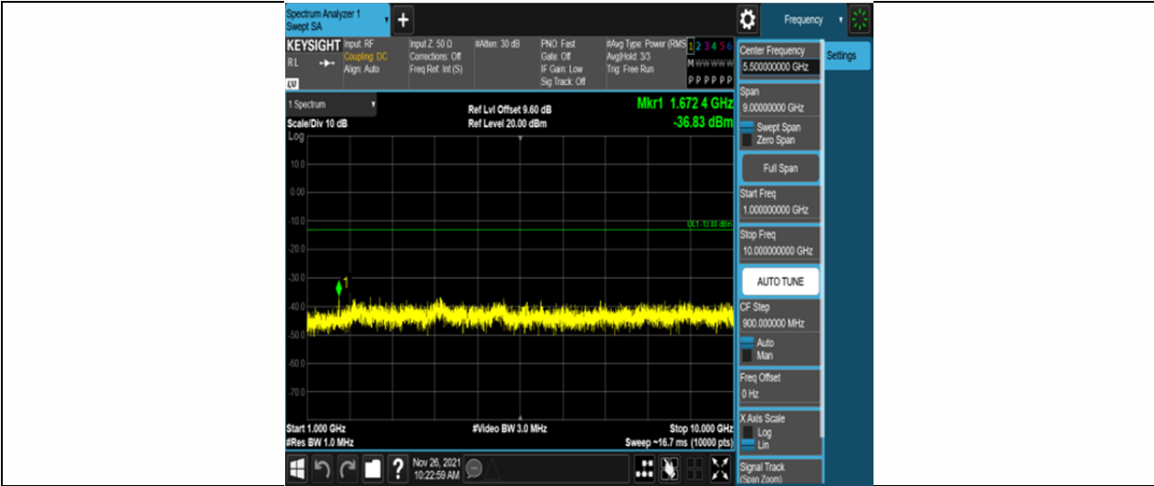
Band5-3MHz-16QAM-20525-15RB#0-Range2:1000~10000MHz
