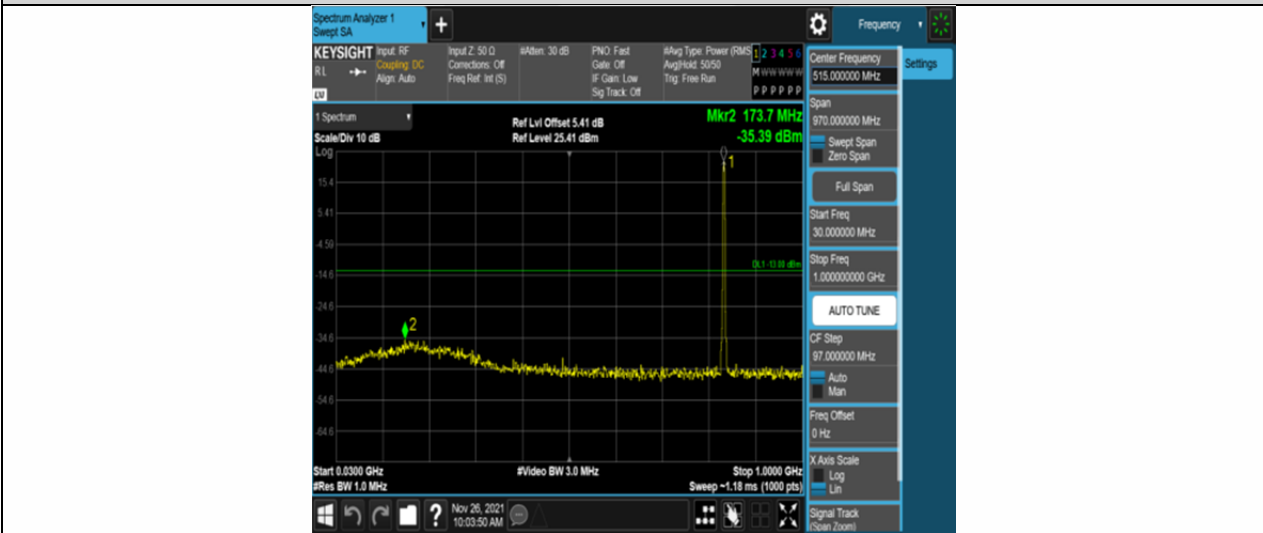
Band5-1.4MHz-16QAM-20525-6RB#0-Range1:30~1000MHz
