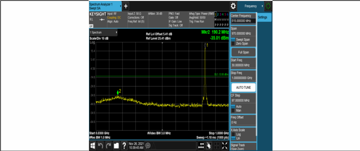
Band5-5MHz-QPSK-20425-25RB#0-Range1:30~1000MHz
