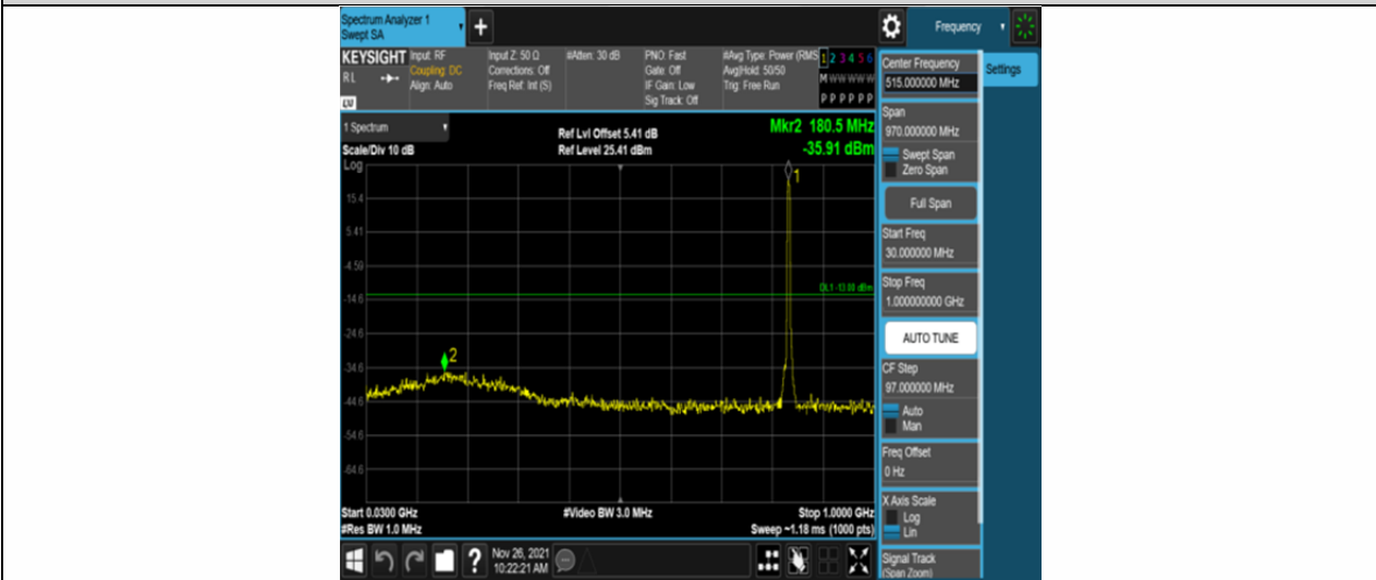
Band5-3MHz-QPSK-20525-15RB#0-Range1:30~1000MHz
