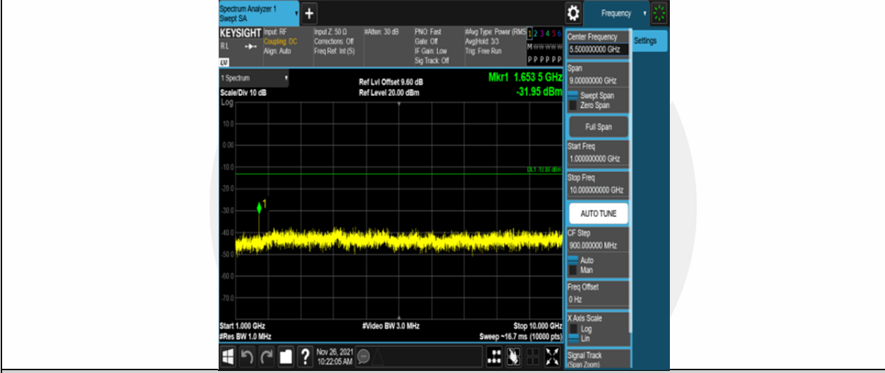
Band5-3MHz-16QAM-20415-15RB#0-Range2:1000~10000MHz
