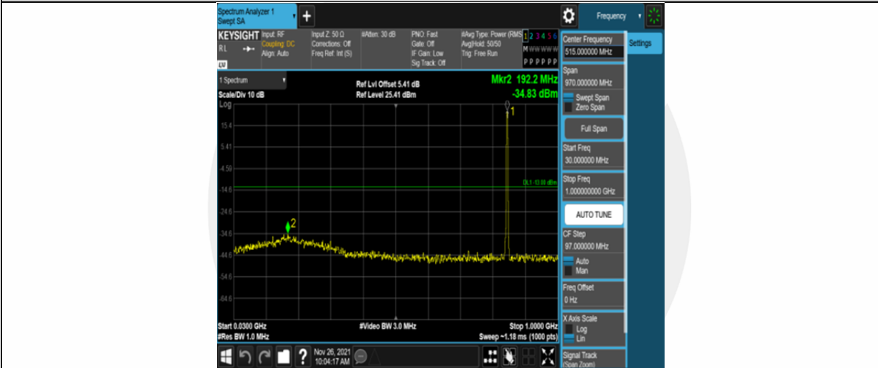
Band5-1.4MHz-QPSK-20643-6RB#0-Range1:30~1000MHz
