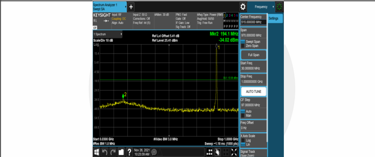
Band5-3MHz-16QAM-20635-15RB#0-Range1:30~1000MHz
