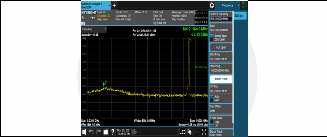
Band5-3MHz-QPSK-20635-15RB#0-Range1:30~1000MHz
