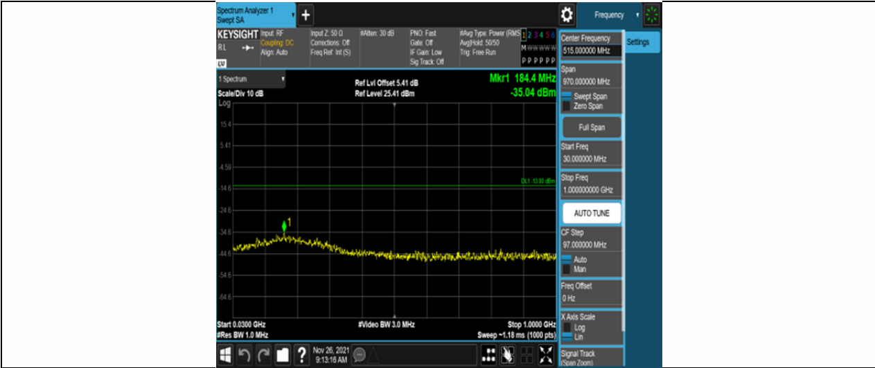
Band4-15MHz-QPSK-20025-75RB#0-Range1:30~1000MHz
