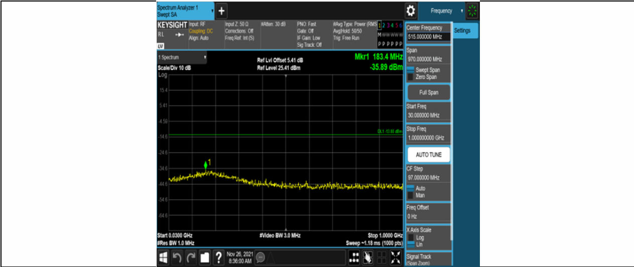
Band4-5MHz-16QAM-20375-25RB#0-Range1:30~1000MHz
