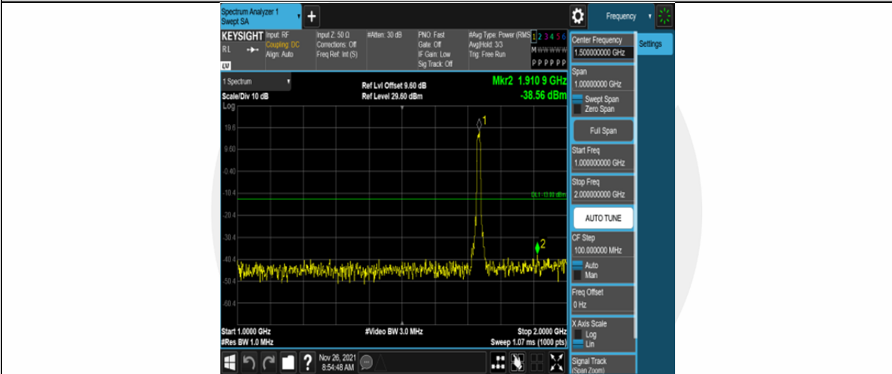
Band4-10MHz-16QAM-20175-50RB#0-Range2:1000~2000MHz
