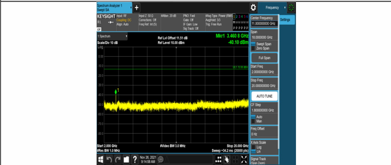
Band4-15MHz-QPSK-20175-75RB#0-Range3:2000~20000MHz
