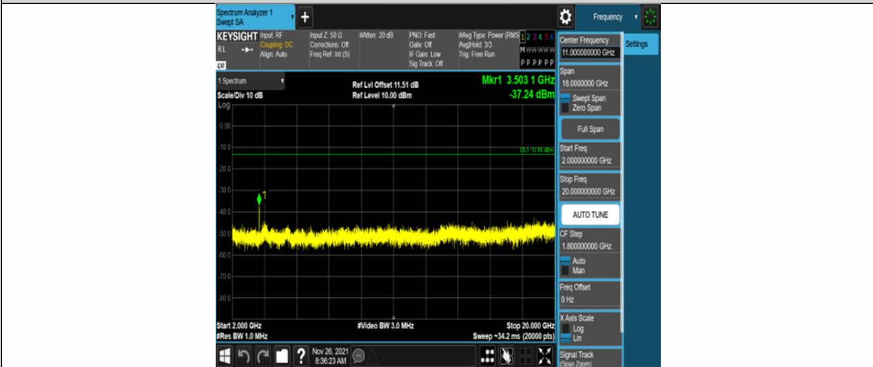
Band4-5MHz-16QAM-20375-25RB#0-Range3:2000~20000MHz
