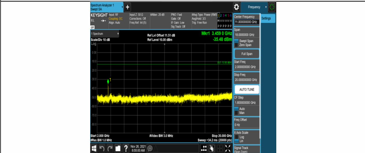
Band4-10MHz-16QAM-20175-50RB#0-Range3:2000~20000MHz
