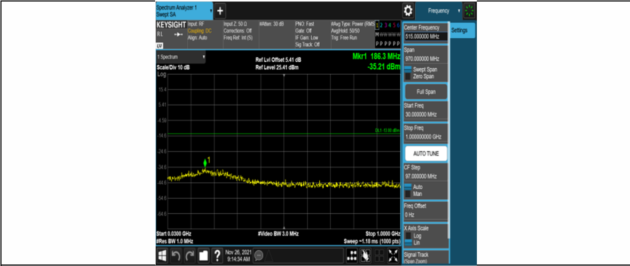
Band4-15MHz-QPSK-20175-75RB#0-Range1:30~1000MHz
