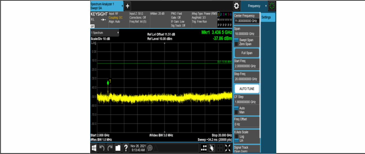
Band4-15MHz-QPSK-20025-75RB#0-Range3:2000~20000MHz
