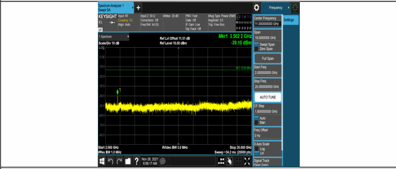
Band4-10MHz-16QAM-20350-50RB#0-Range3:2000~20000MHz
