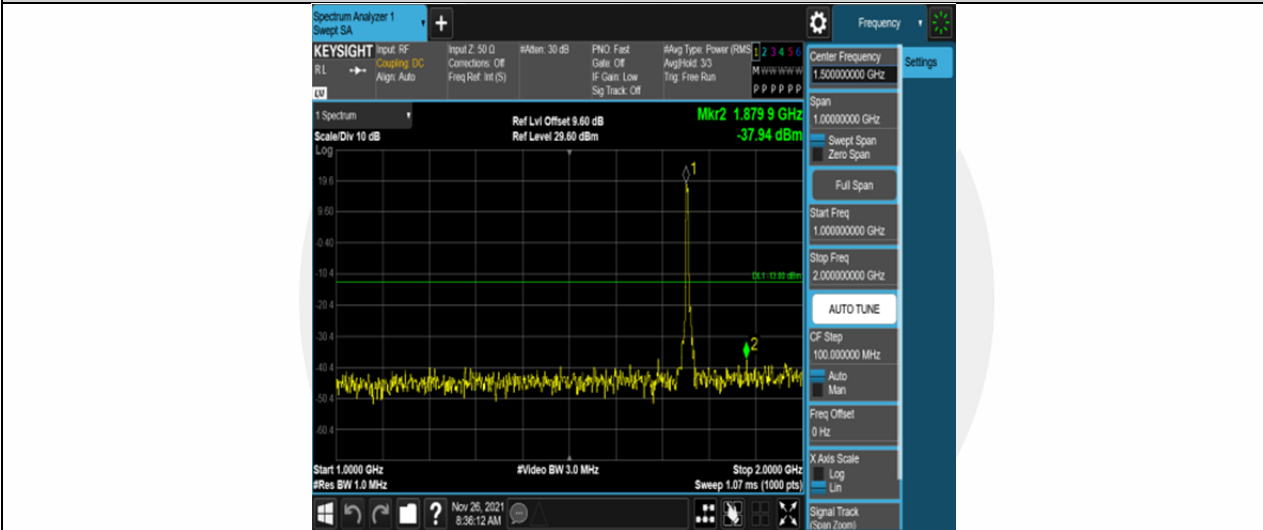
Band4-5MHz-16QAM-20375-25RB#0-Range2:1000~2000MHz
