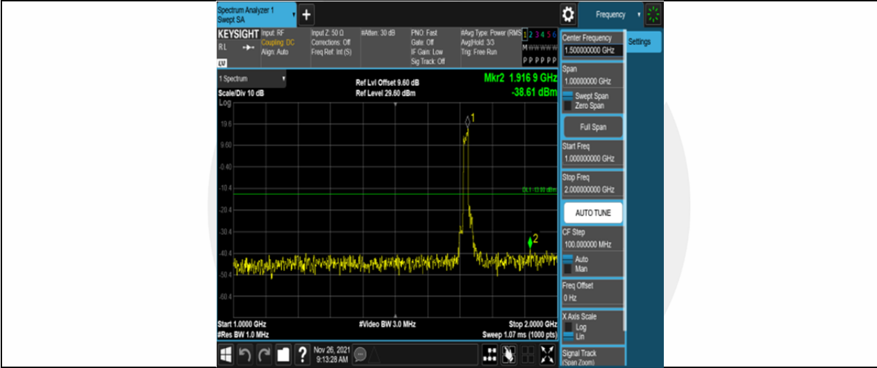
Band4-15MHz-QPSK-20025-75RB#0-Range2:1000~2000MHz
