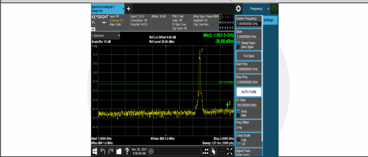
Band4-10MHz-16QAM-20350-50RB#0-Range2:1000~2000MHz
