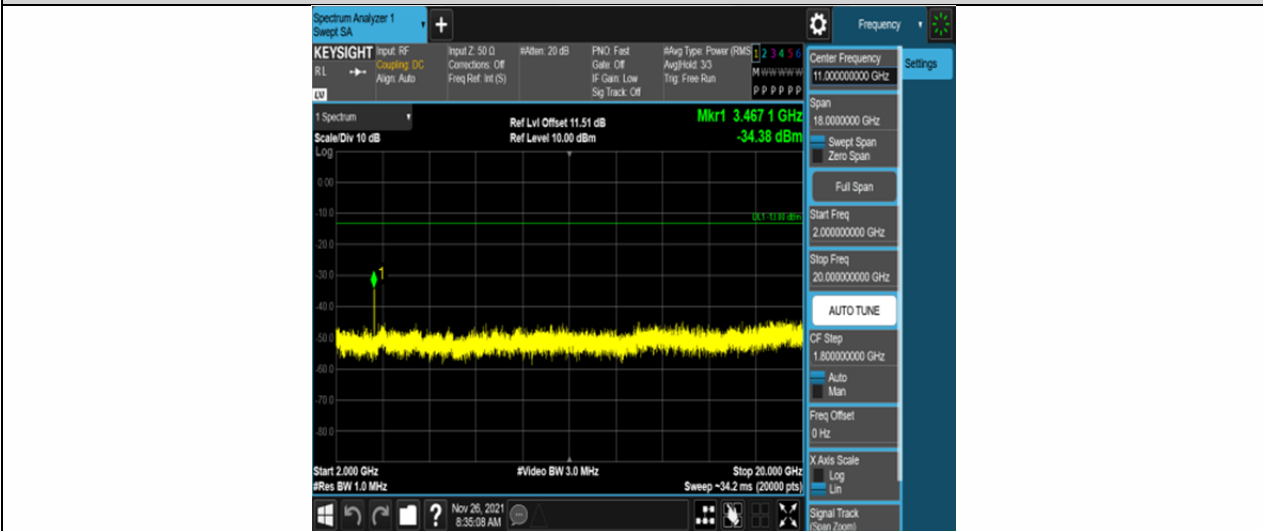
Band4-5MHz-16QAM-20175-25RB#0-Range3:2000~20000MHz
