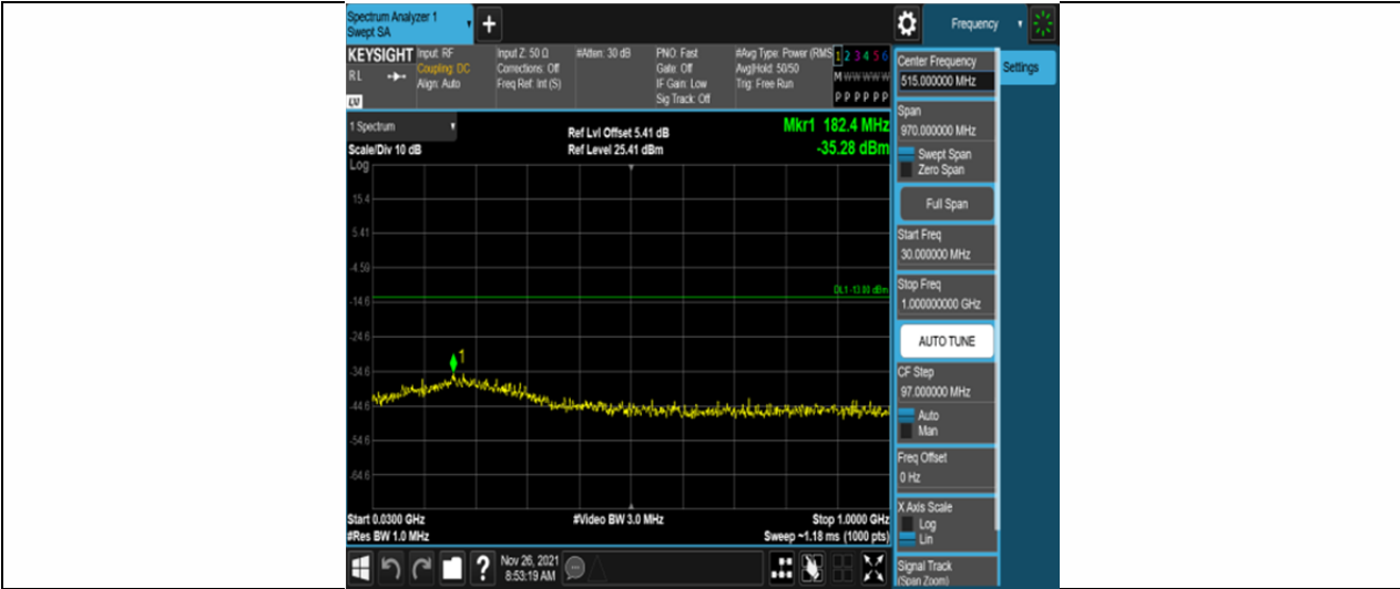
Band4-10MHz-16QAM-20000-50RB#0-Range1:30~1000MHz
