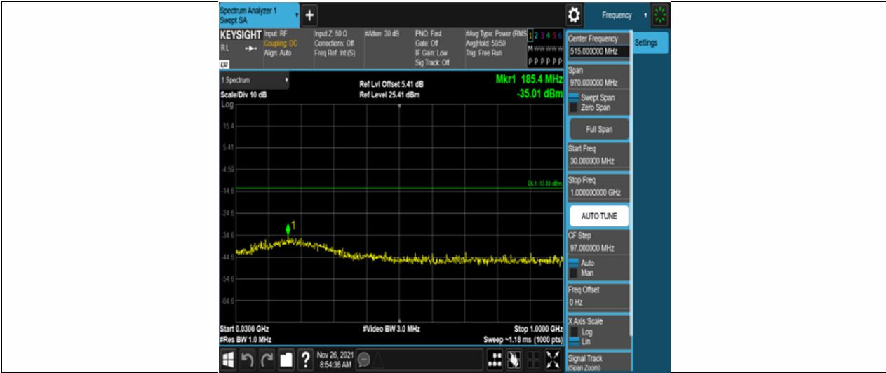
Band4-10MHz-16QAM-20175-50RB#0-Range1:30~1000MHz
