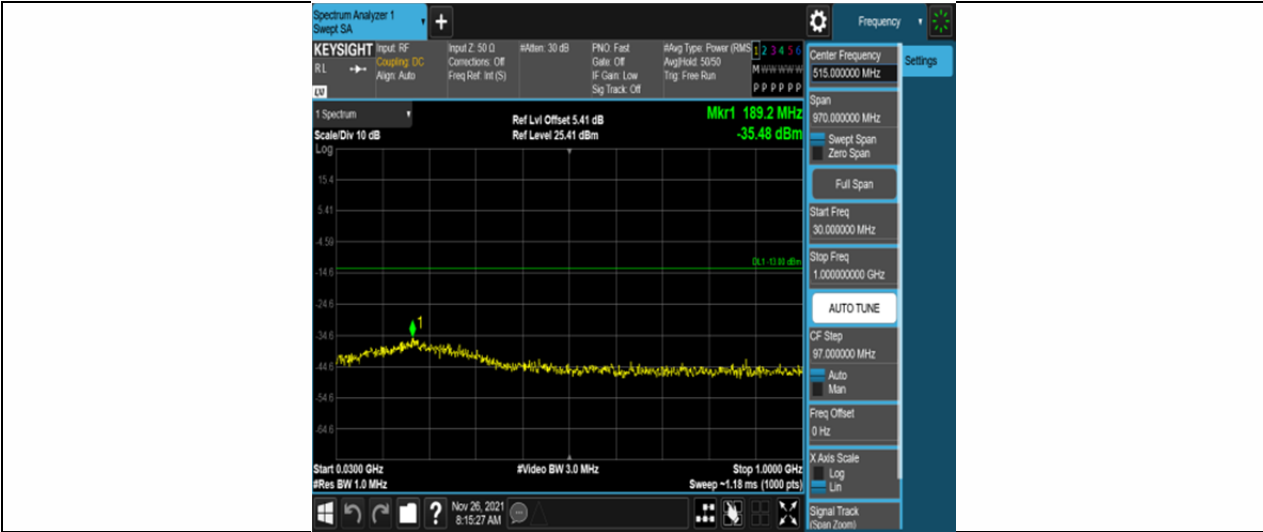
Band4-3MHz-16QAM-20385-6RB#0-Range1:30~1000MHz
