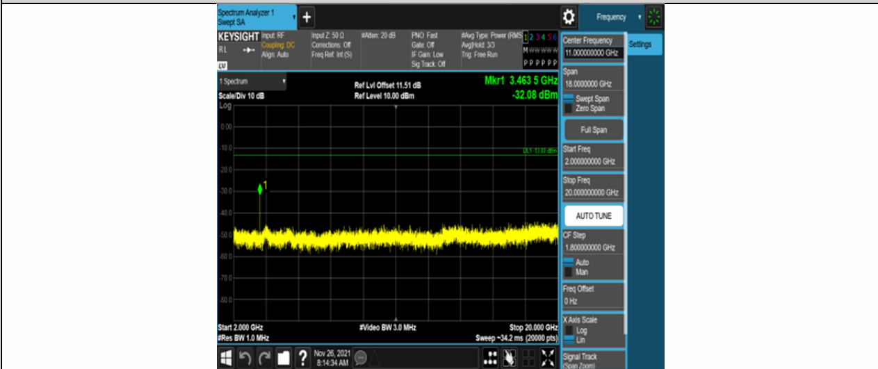
Band4-3MHz-16QAM-20175-6RB#0-Range3:2000~20000MHz
