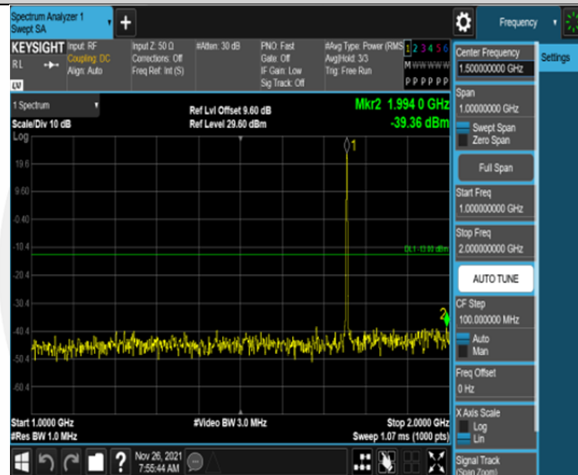
Band4-1.4MHz-16QAM-20393-6RB#0-Range2:1000~2000MHz
