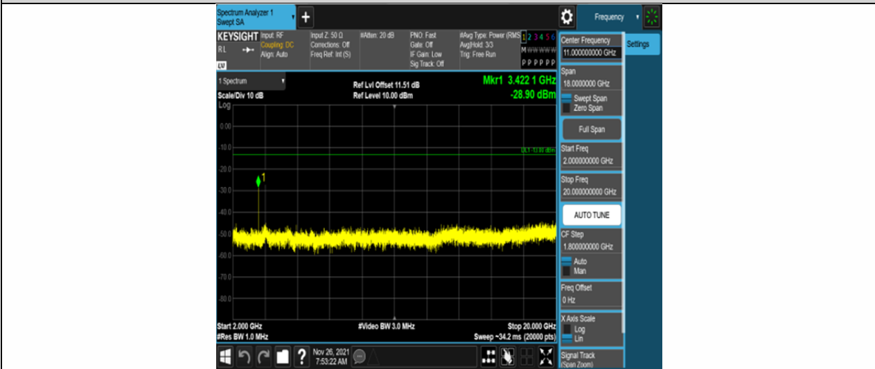
Band4-1.4MHz-16QAM-19957-6RB#0-Range3:2000~20000MHz
