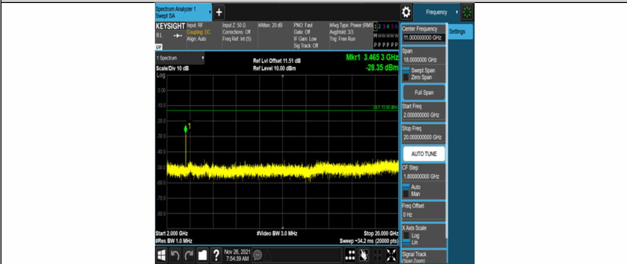
Band4-1.4MHz-16QAM-20175-6RB#0-Range3:2000~20000MHz
