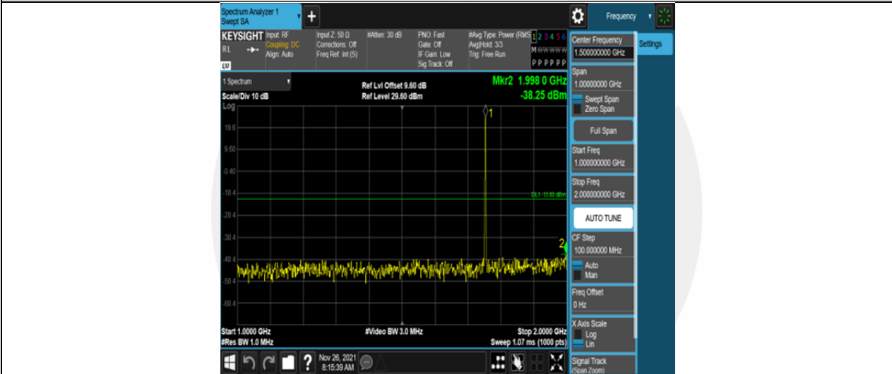
Band4-3MHz-16QAM-20385-6RB#0-Range2:1000~2000MHz
