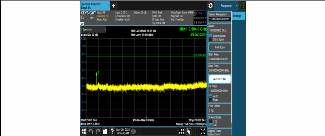
Band4-5MHz-QPSK-20375-25RB#0-Range3:2000~20000MHz
