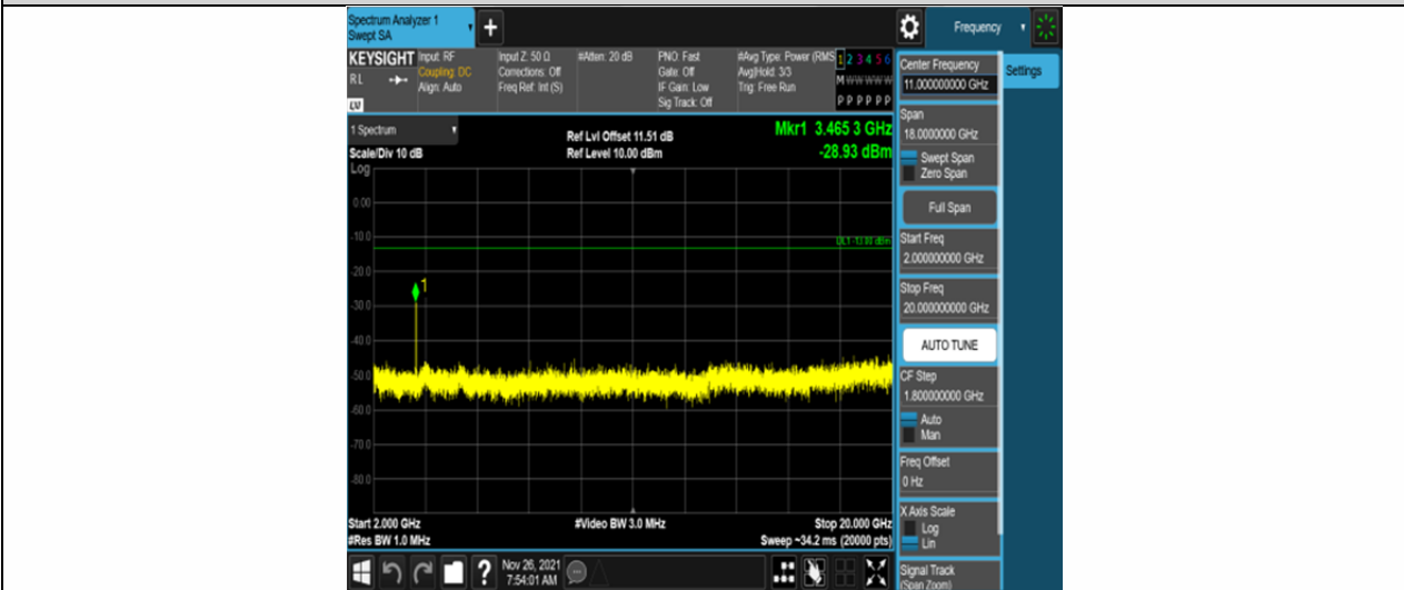
Band4-1.4MHz-QPSK-20175-6RB#0-Range3:2000~20000MHz
