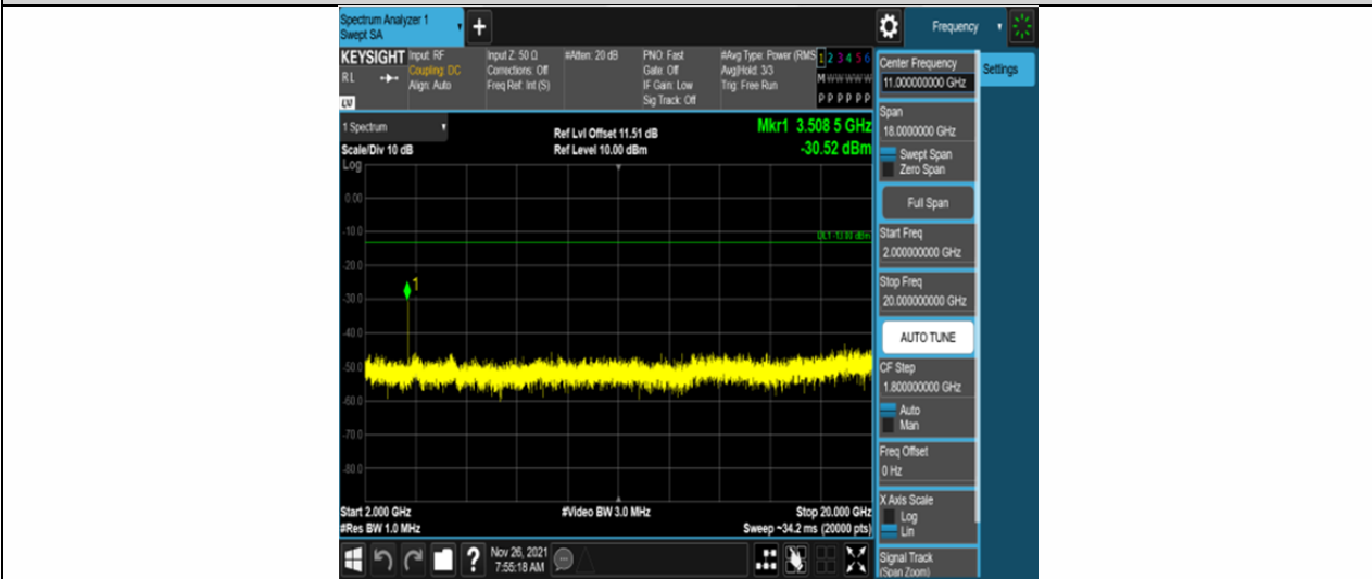
Band4-1.4MHz-QPSK-20393-6RB#0-Range3:2000~20000MHz
