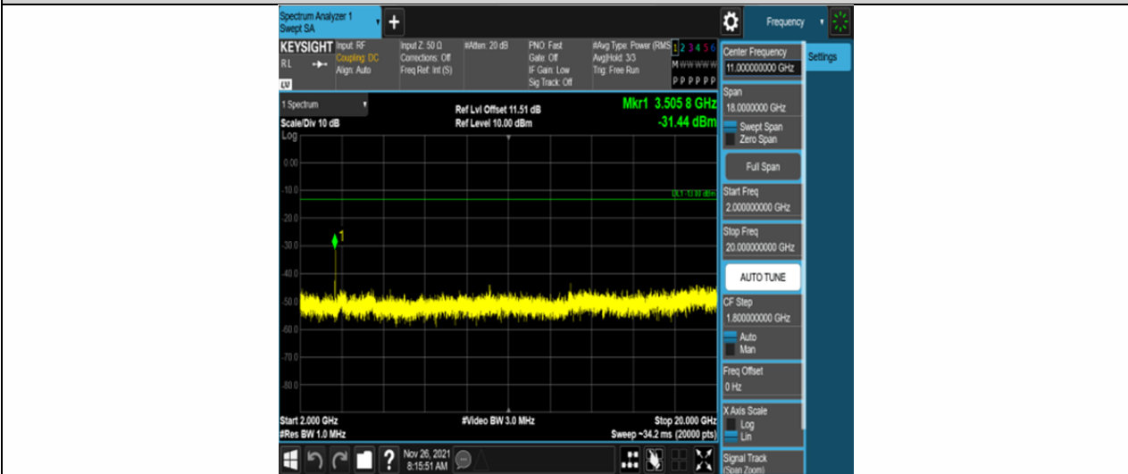
Band4-3MHz-16QAM-20385-6RB#0-Range3:2000~20000MHz
