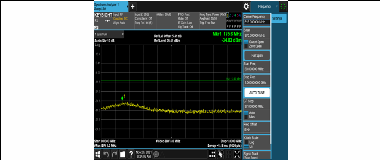
Band4-5MHz-QPSK-20175-25RB#0-Range1:30~1000MHz
