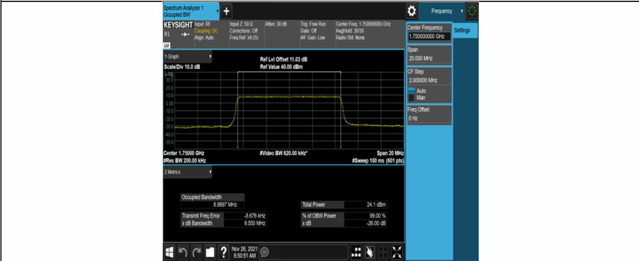
Band4-10MHz-QPSK-20350-50RB#0
