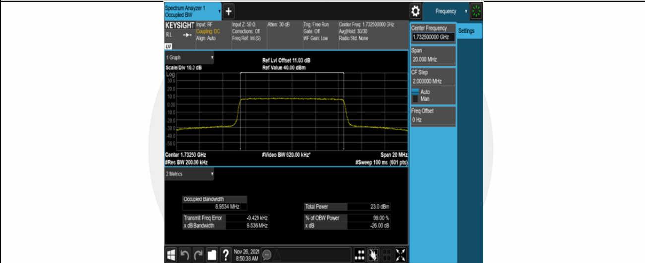
Band4-10MHz-16QAM-20175-50RB#0
