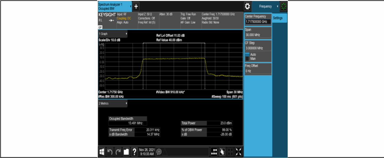
Band4-15MHz-QPSK-20025-75RB#0
