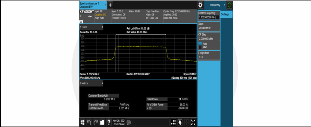
Band4-10MHz-QPSK-20175-50RB#0
