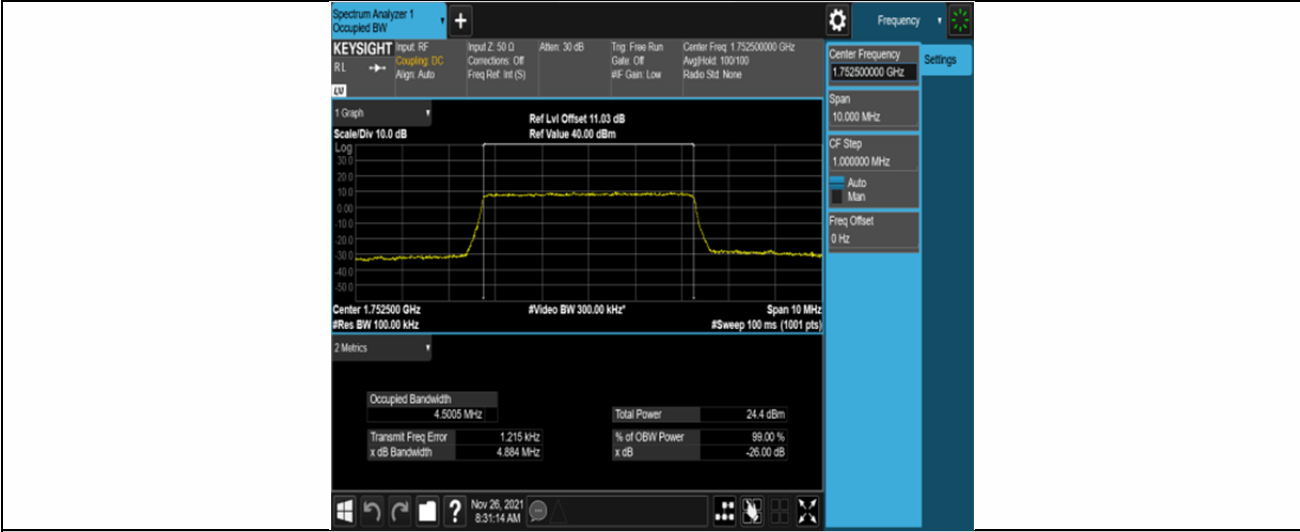
Band4-5MHz-16QAM-20375-25RB#0
