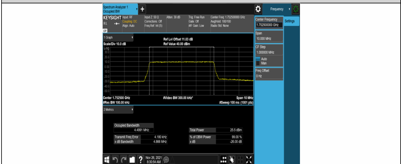
Band4-5MHz-QPSK-20375-25RB#0
