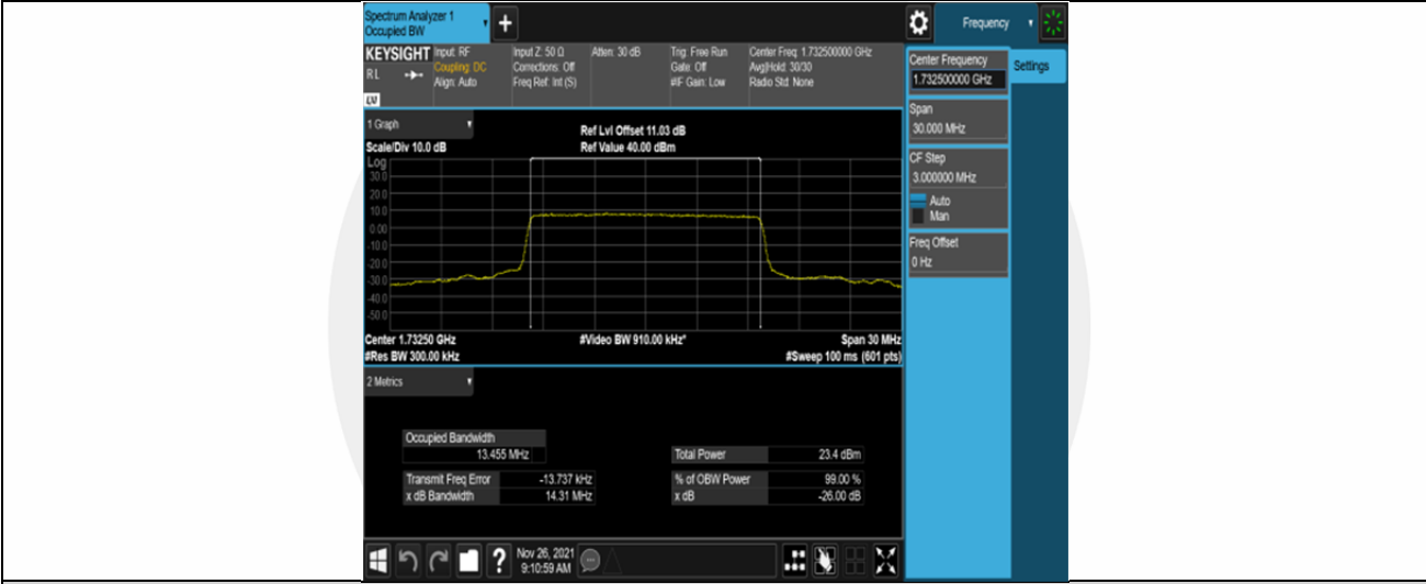
Band4-15MHz-QPSK-20175-75RB#0
