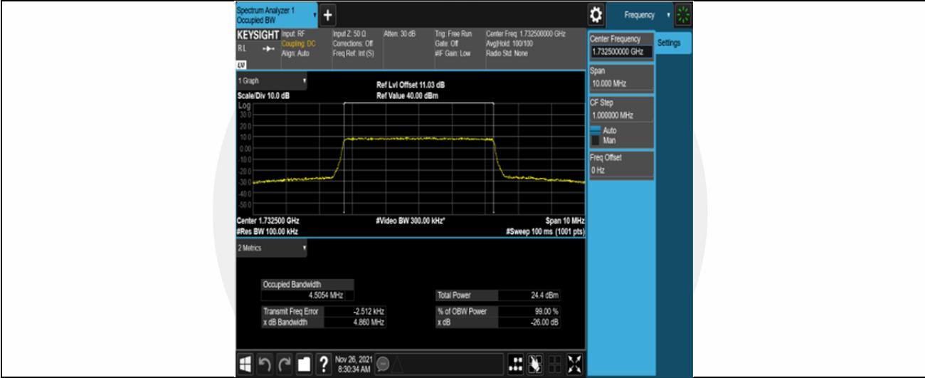
Band4-5MHz-16QAM-20175-25RB#0
