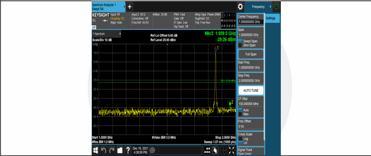
Band2-5MHz-16QAM-18625-25RB#0-Range2:1000~2000MHz
