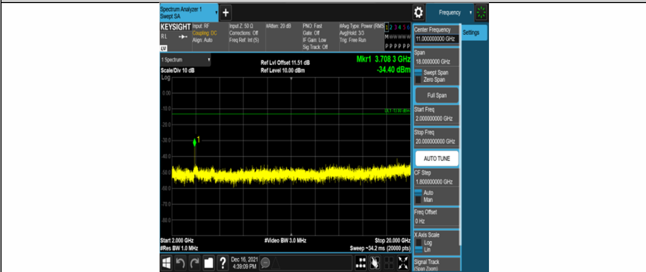
Band2-5MHz-16QAM-18625-25RB#0-Range3:2000~20000MHz
