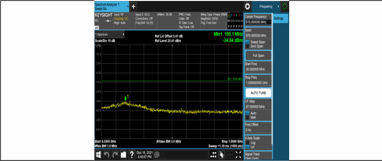
Band2-10MHz-QPSK-18900-50RB#0-Range1:30~1000MHz
