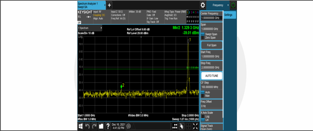
Band2-5MHz-16QAM-19175-25RB#0-Range2:1000~2000MHz
