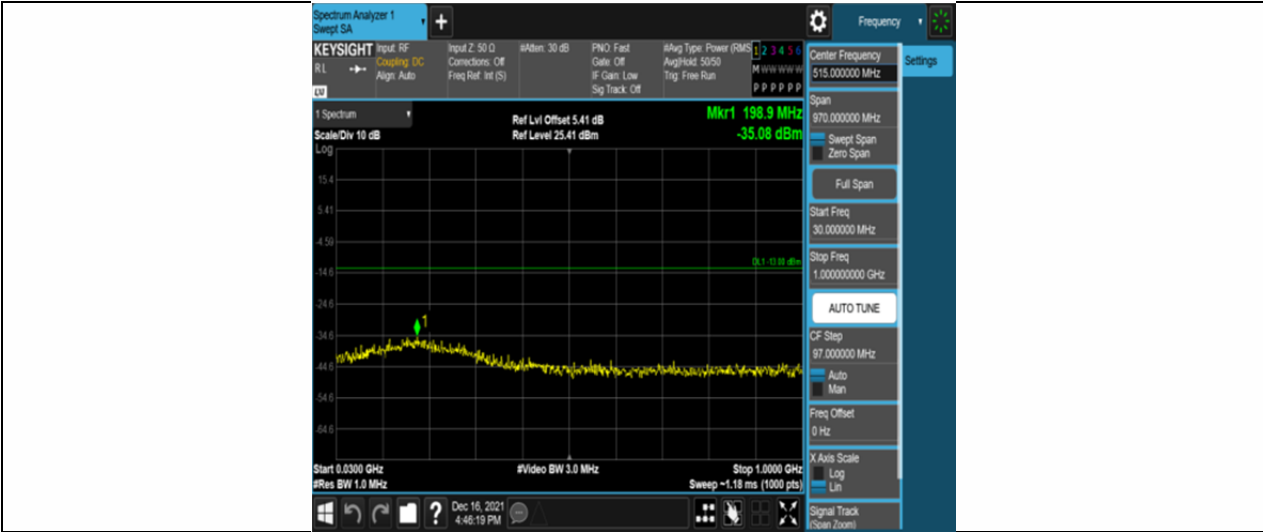
Band2-10MHz-16QAM-18650-50RB#0-Range1:30~1000MHz
