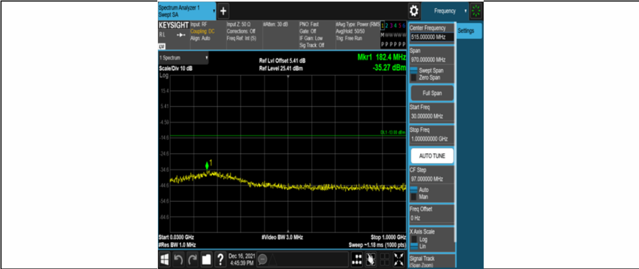
Band2-10MHz-QPSK-18650-50RB#0-Range1:30~1000MHz
