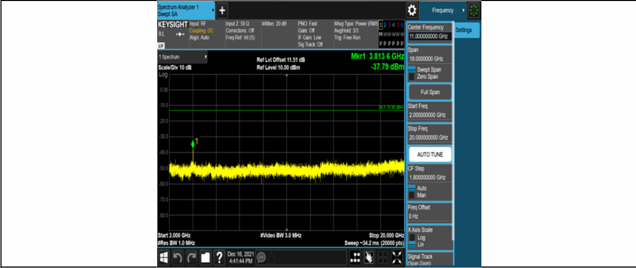
Band2-5MHz-16QAM-19175-25RB#0-Range3:2000~20000MHz
