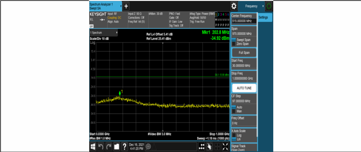
Band2-5MHz-16QAM-19175-25RB#0-Range1:30~1000MHz
