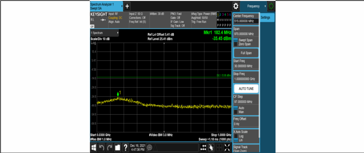
Band2-10MHz-16QAM-18900-50RB#0-Range1:30~1000MHz
