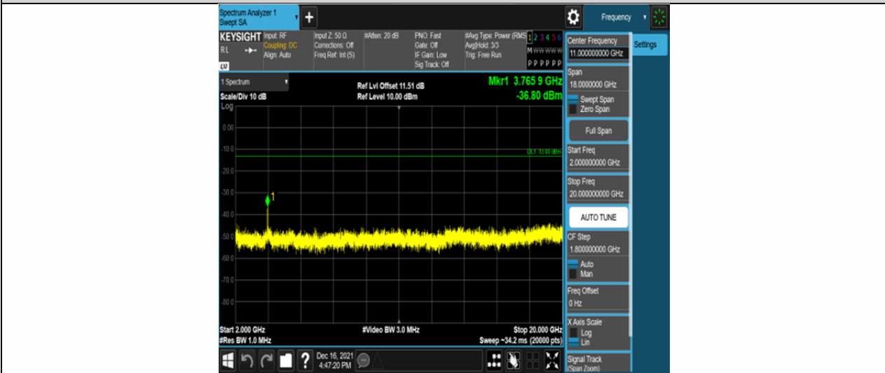
Band2-10MHz-QPSK-18900-50RB#0-Range3:2000~20000MHz
