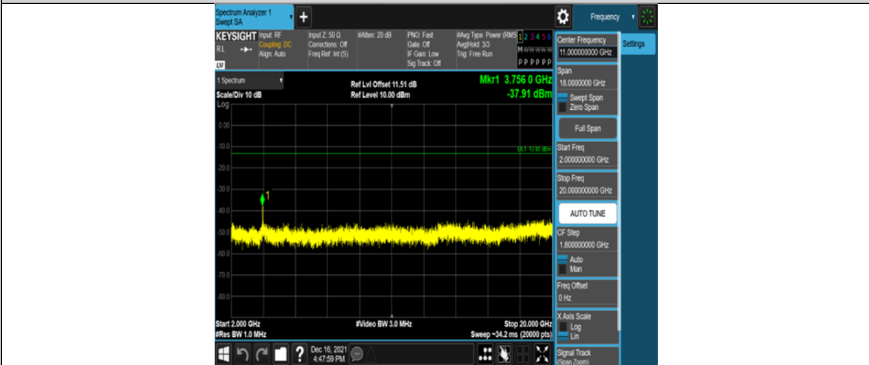
Band2-10MHz-16QAM-18900-50RB#0-Range3:2000~20000MHz
