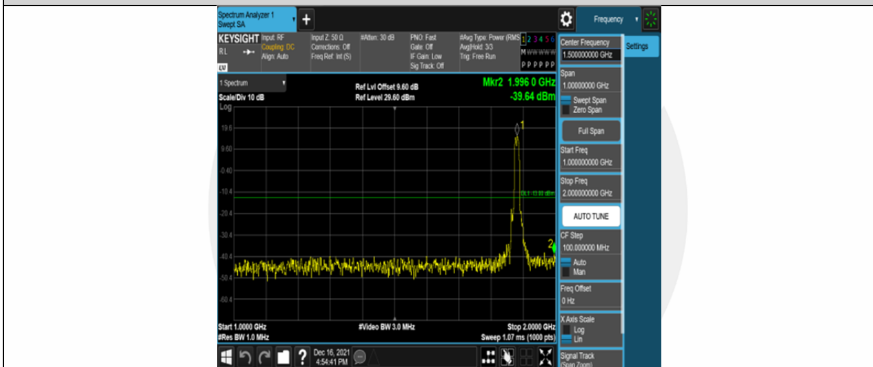
Band2-15MHz-QPSK-18900-75RB#0-Range2:1000~2000MHz
