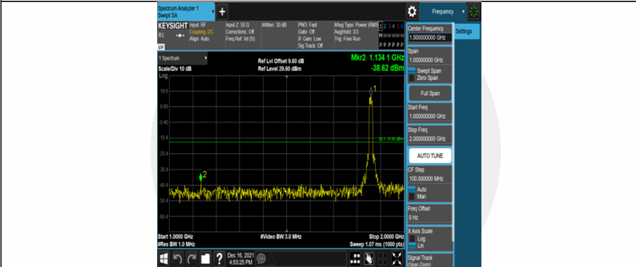
Band2-15MHz-QPSK-18675-75RB#0-Range2:1000~2000MHz
