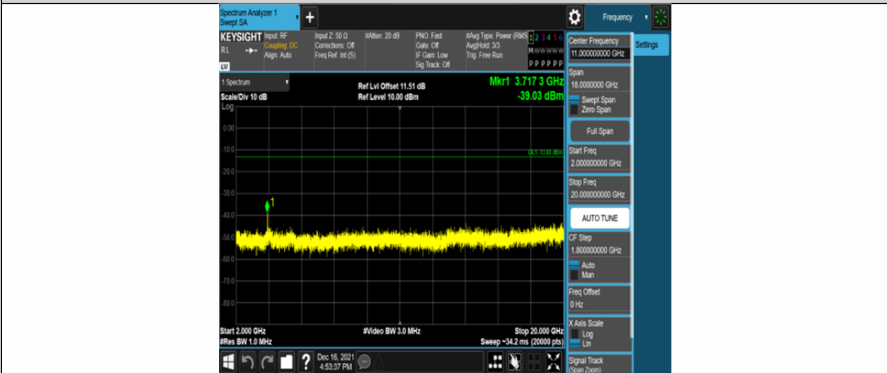
Band2-15MHz-QPSK-18675-75RB#0-Range3:2000~20000MHz
