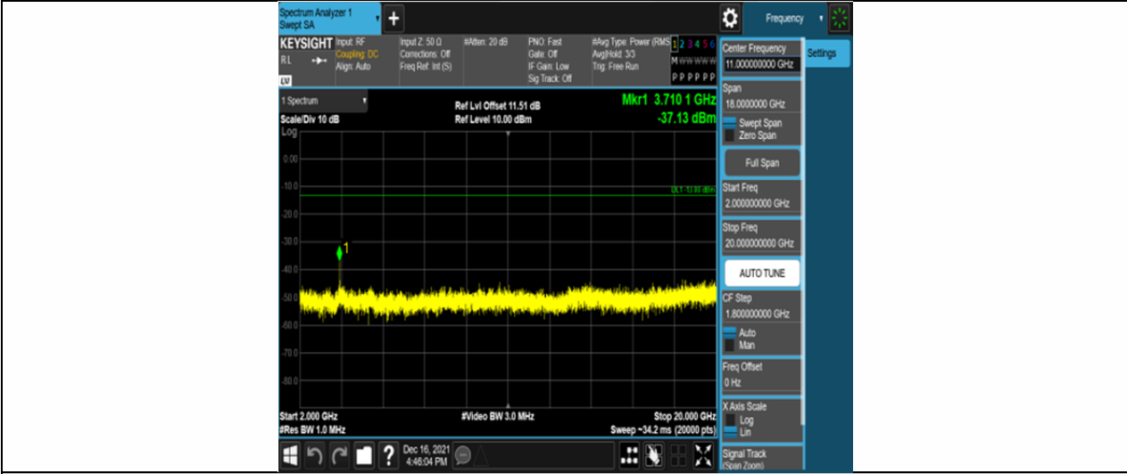
Band2-10MHz-QPSK-18650-50RB#0-Range3:2000~20000MHz
