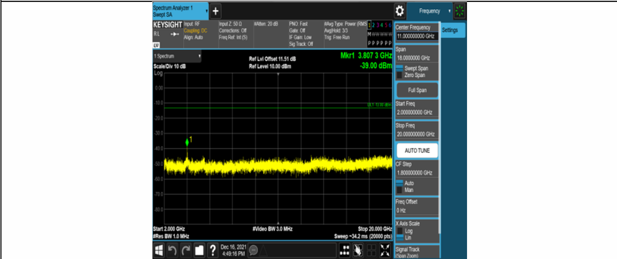
Band2-10MHz-16QAM-19150-50RB#0-Range3:2000~20000MHz
