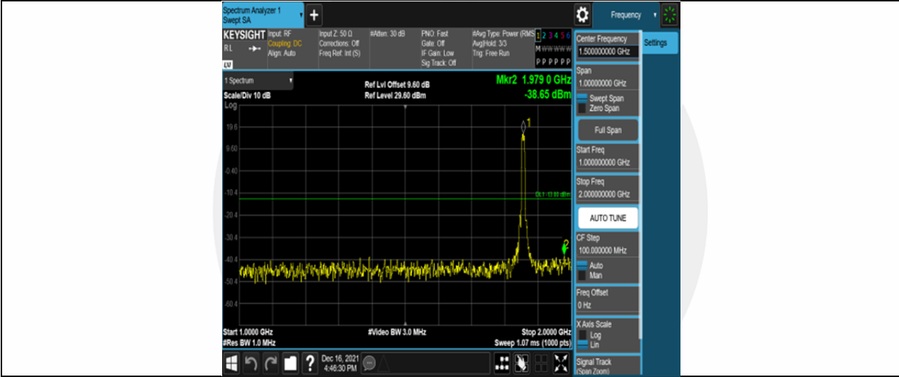
Band2-10MHz-16QAM-18650-50RB#0-Range2:1000~2000MHz
