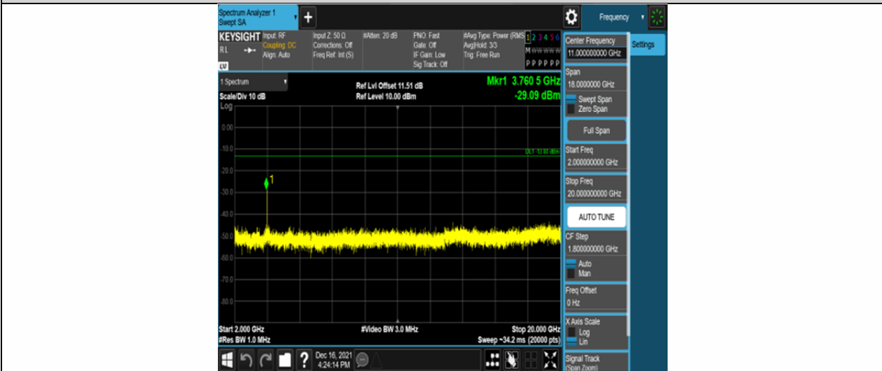
Band2-1.4MHz-QPSK-18900-6RB#0-Range3:2000~20000MHz
