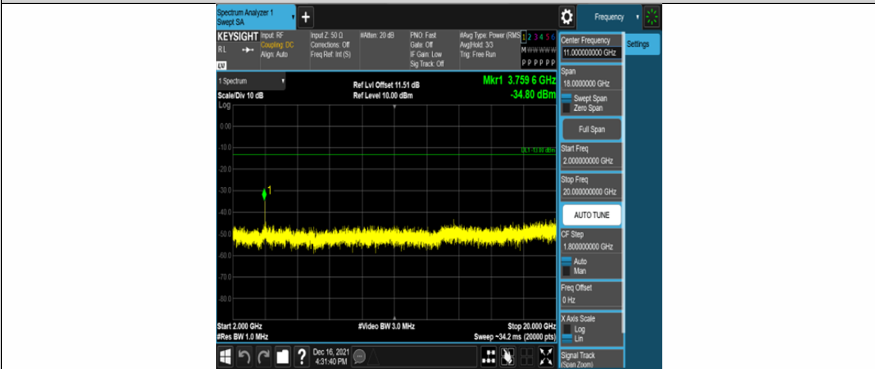
Band2-3MHz-QPSK-18900-15RB#0-Range3:2000~20000MHz
