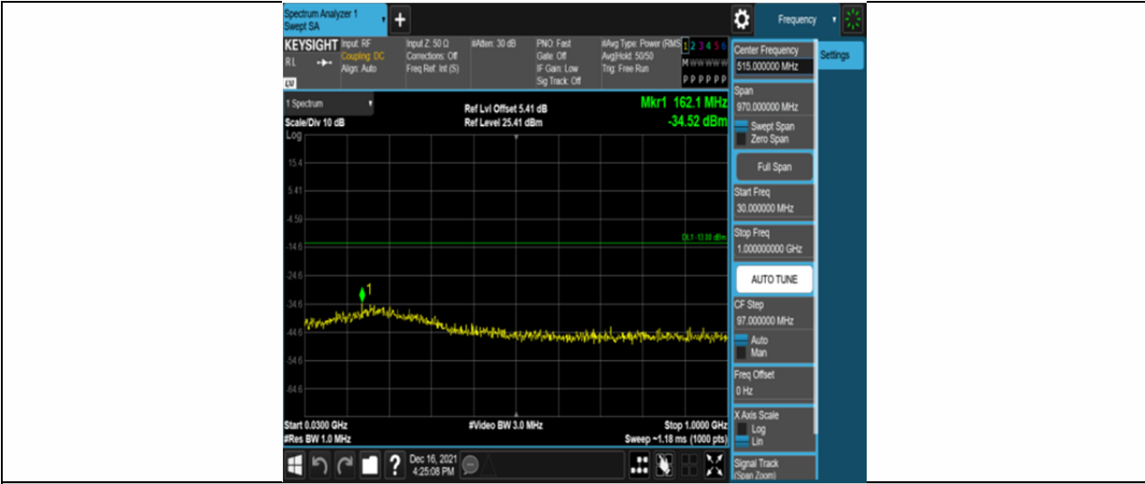
Band2-1.4MHz-QPSK-19193-6RB#0-Range1:30~1000MHz
