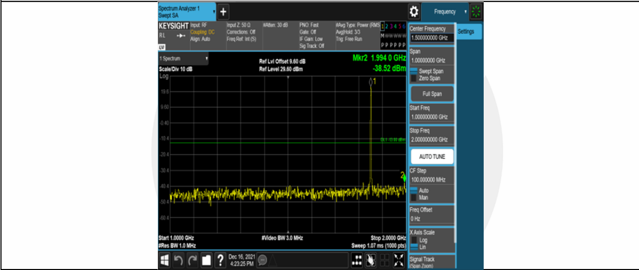
Band2-1.4MHz-16QAM-18607-6RB#0-Range2:1000~2000MHz
