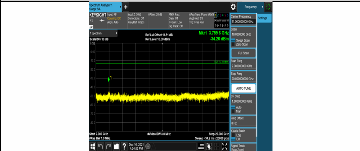
Band2-1.4MHz-16QAM-18900-6RB#0-Range3:2000~20000MHz
