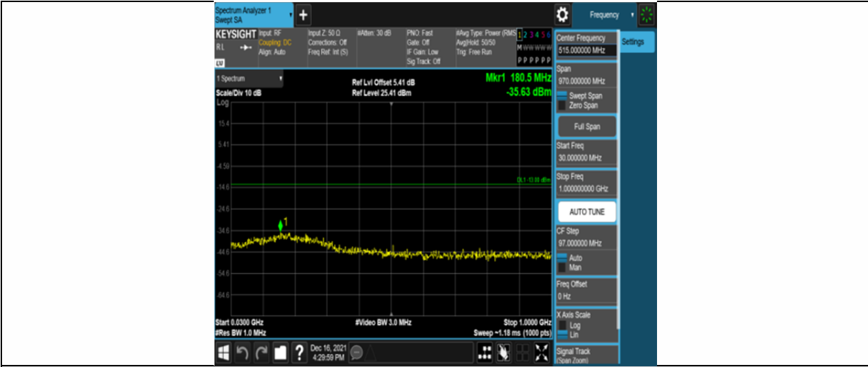
Band2-3MHz-QPSK-18615-15RB#0-Range1:30~1000MHz
