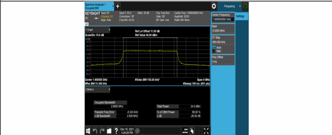
Band2-3MHz-16QAM-19185-15RB#0
