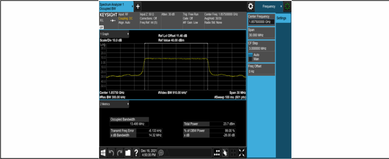
Band2-15MHz-QPSK-18675-75RB#0
