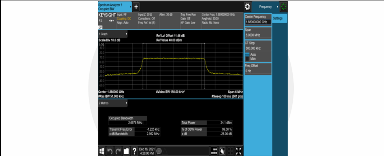
Band2-3MHz-16QAM-18900-15RB#0
