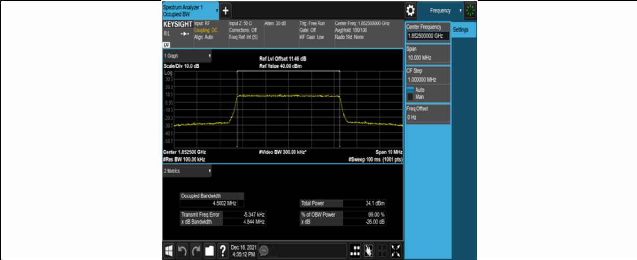
Band2-5MHz-16QAM-18625-25RB#0
