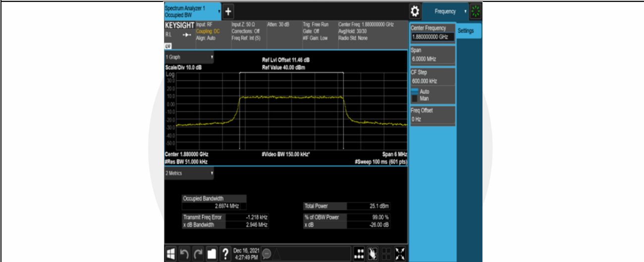
Band2-3MHz-QPSK-18900-15RB#0
