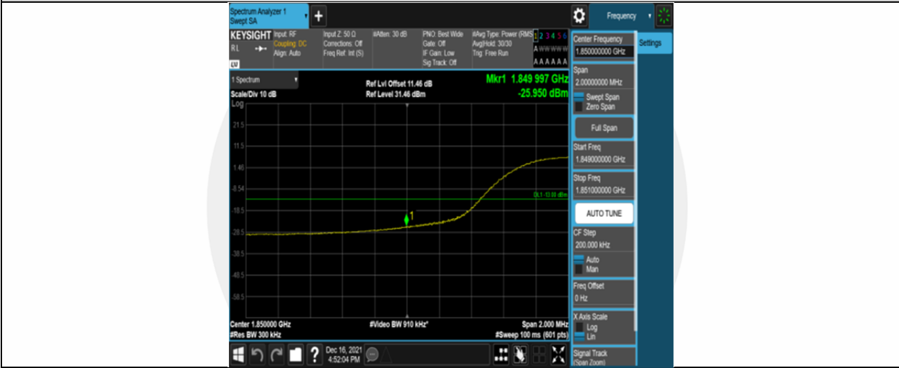
Band2-15MHz-QPSK-18675-75RB#0
