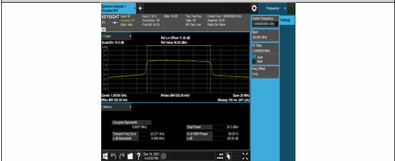
Band2-10MHz-QPSK-19150-50RB#0
