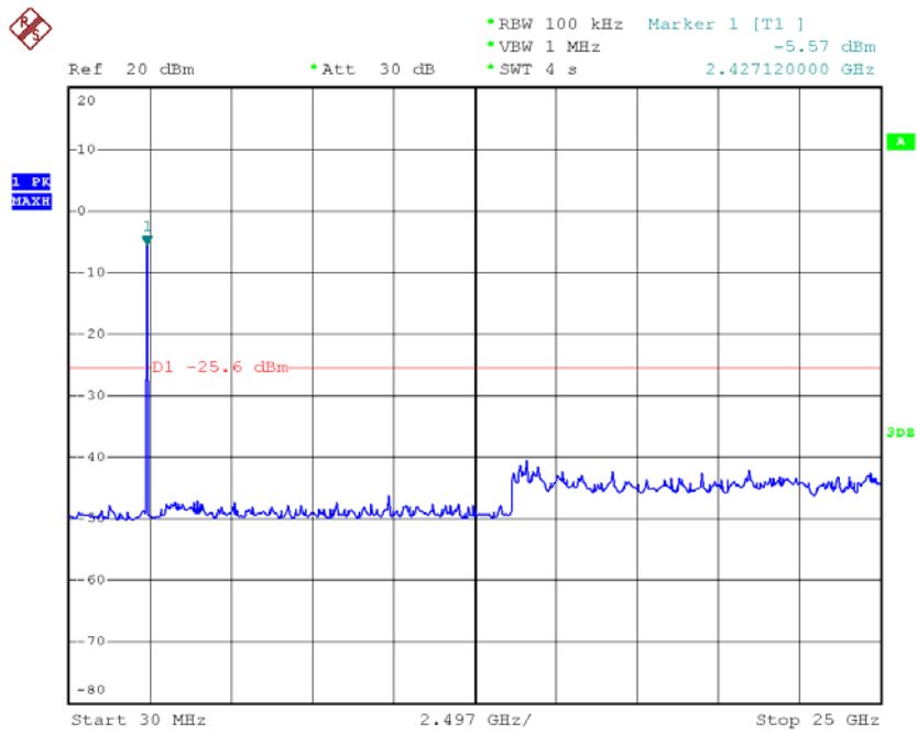
Figure Channel 39: 30MHz-25GHz
