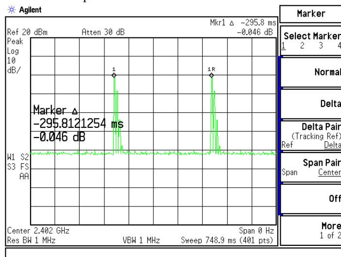
CH 2402MHz Time Interval between hops
