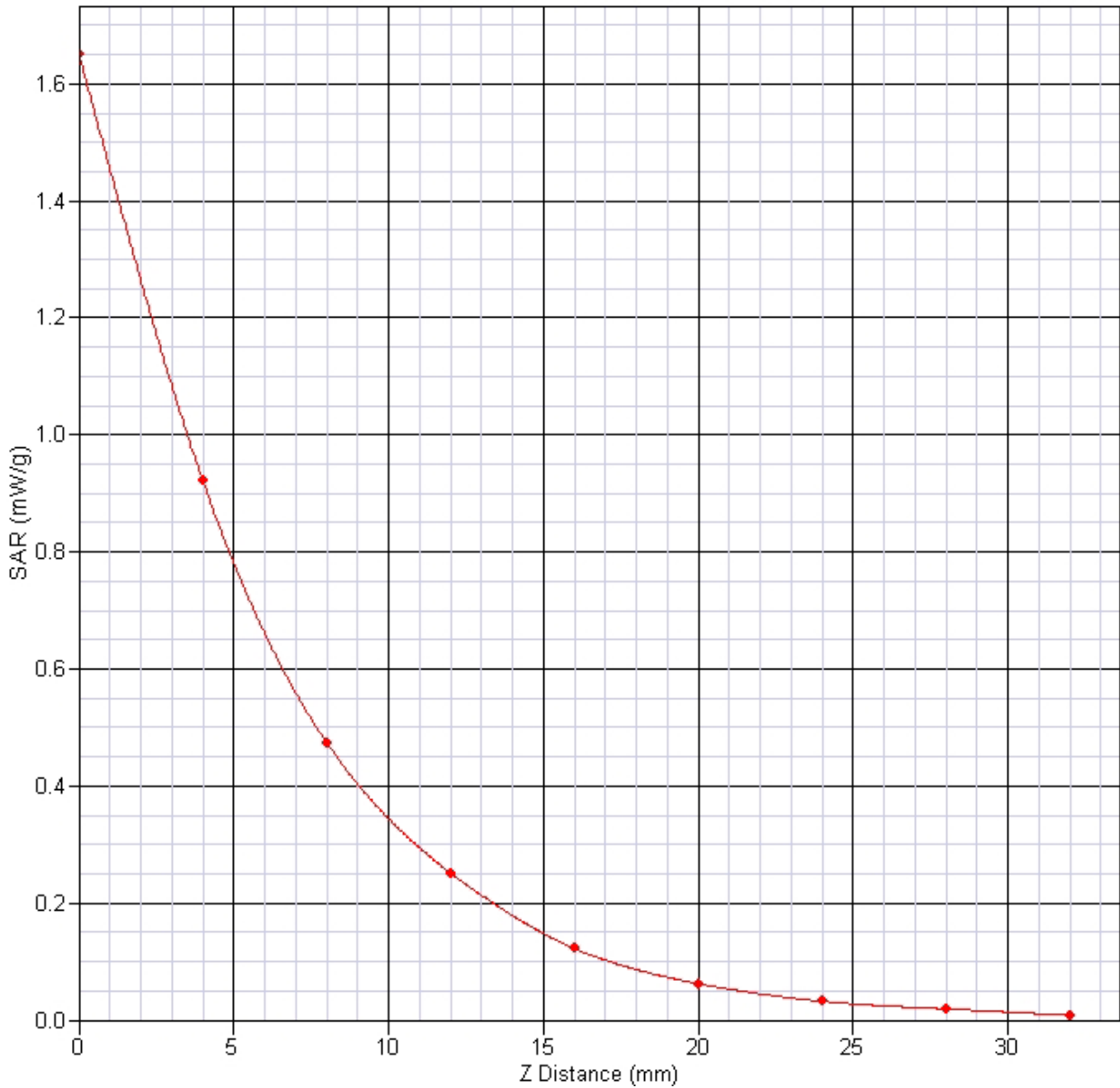
SAR-Z Axis at Hotspot x:-2.0 y:11.9
