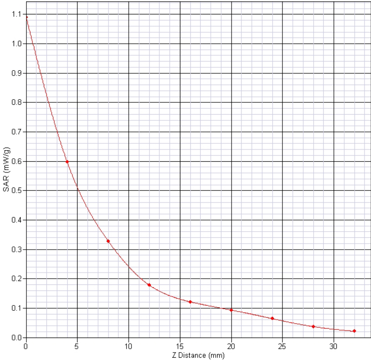
SAR-Z Axis at Hotspot x:0.0 y:0.0
