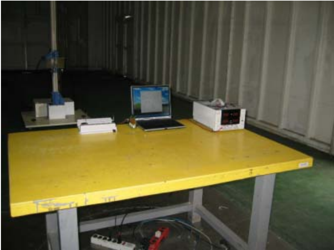
Front View of High Frequency Radiated Test (Mode 8)
