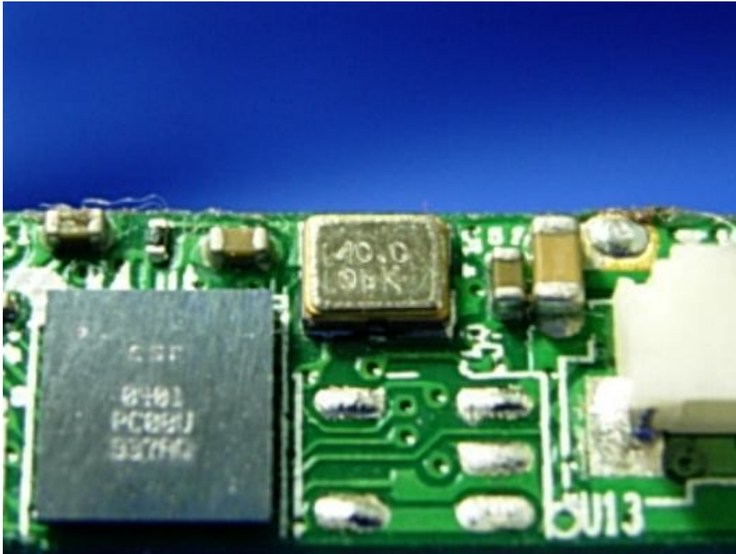
(26) EUT Photo (without U12 component)
