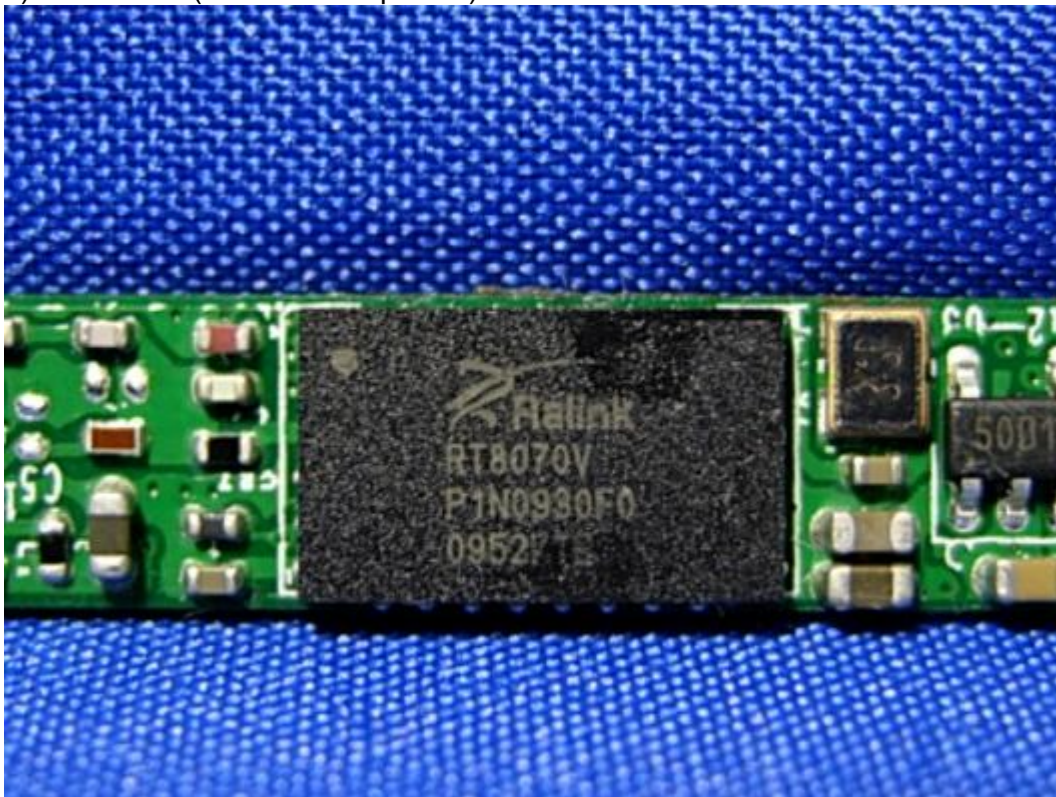
(12) EUT Photo (with U12 component)
