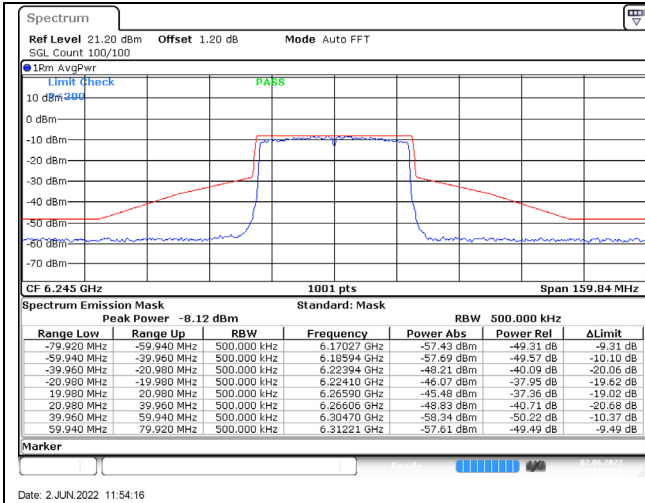
802.11ax (40MHz) / 6245MHz / Chain A / NSS-4
