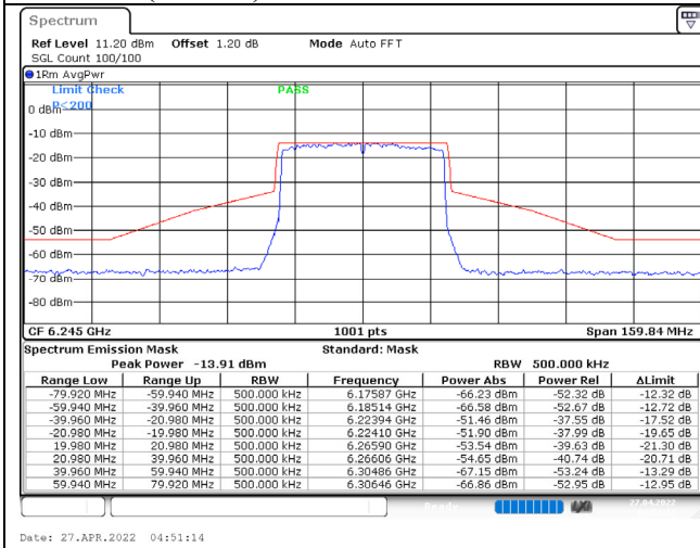
802.11ax (40MHz) / 6245MHz / Chain A / NSS-1
