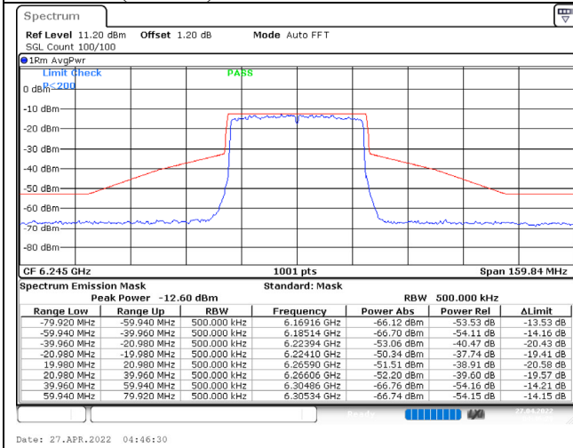
802.11ax (40MHz) / 6245MHz / Chain C / NSS-1
