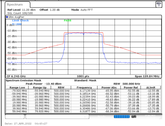
802.11ax (40MHz) / 6245MHz / Chain D / NSS-1
