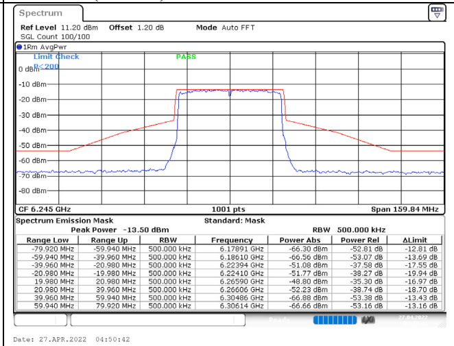
802.11ax (40MHz) / 6245MHz / Chain B / NSS-1
