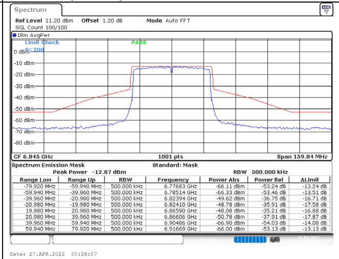
802.11ax (40MHz) / 6845MHz / Chain D / NSS-1
