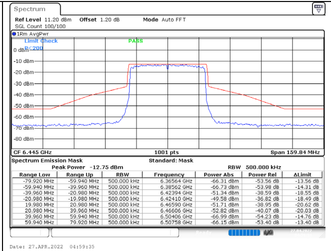
802.11ax (40MHz) / 6445MHz / Chain D / NSS-1
