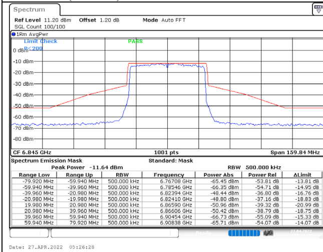
802.11ax (40MHz) / 6845MHz / Chain C / NSS-1
