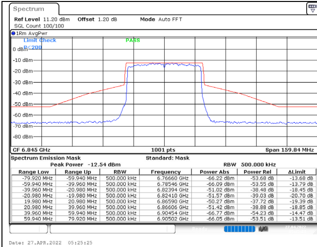
802.11ax (40MHz) / 6845MHz / Chain A / NSS-1
