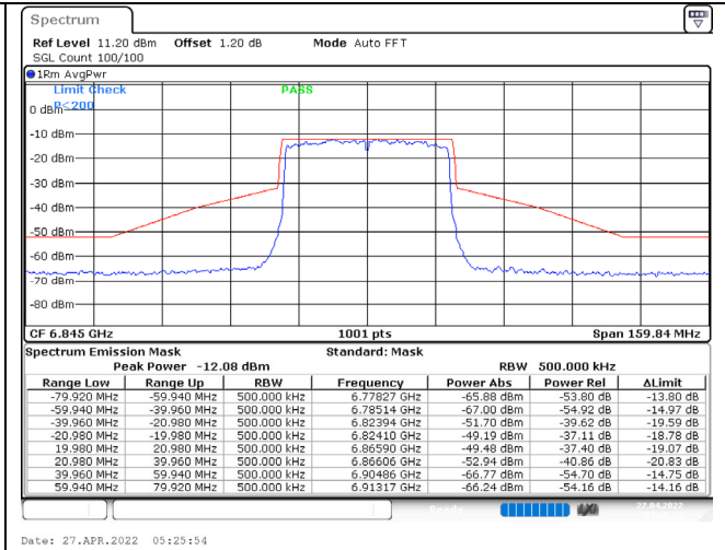
802.11ax (40MHz) / 6845MHz / Chain B / NSS-1
