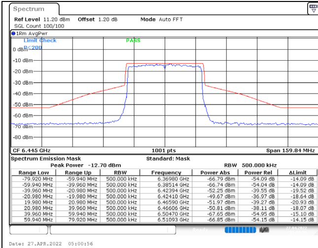
802.11ax (40MHz) / 6445MHz / Chain C / NSS-1
