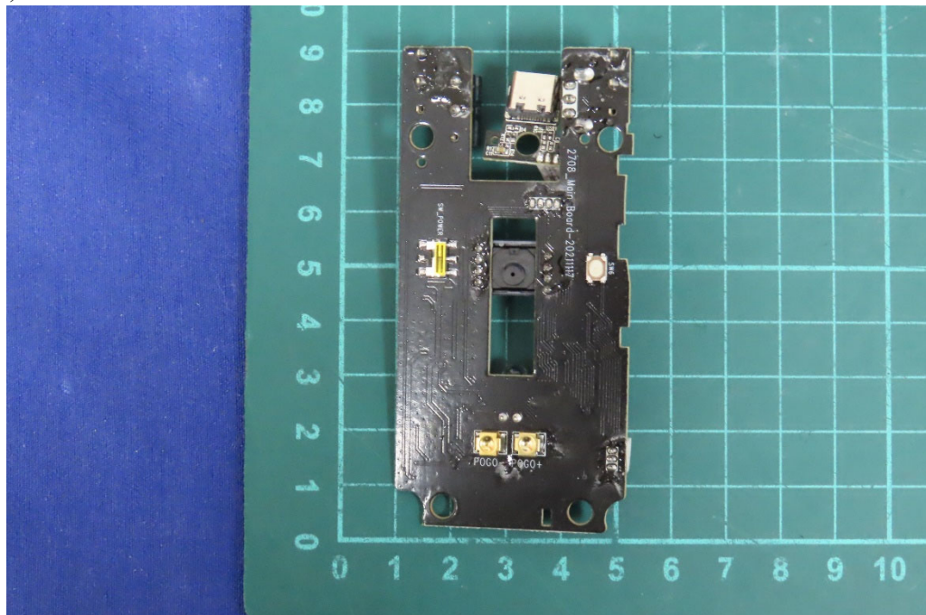
(22) EUT Photo
