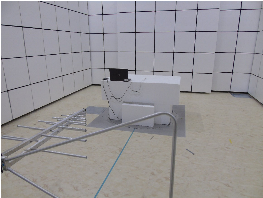
Radiated Test
