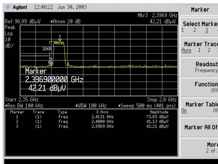
Figure Channel 1: (Vertical)
