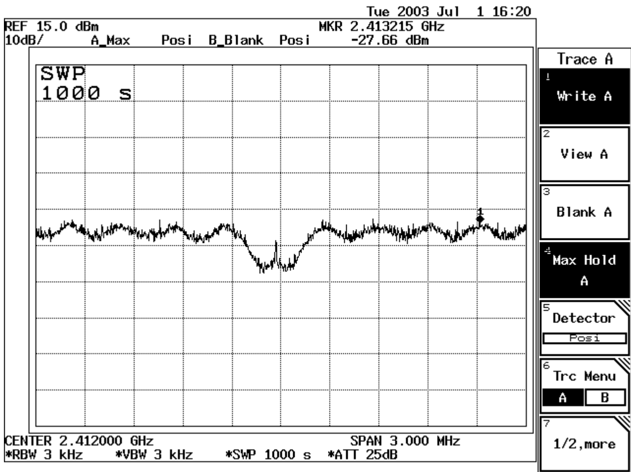
Figure Channel 1: 54Mbps
