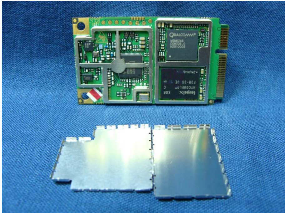
(11) EUT Photo
