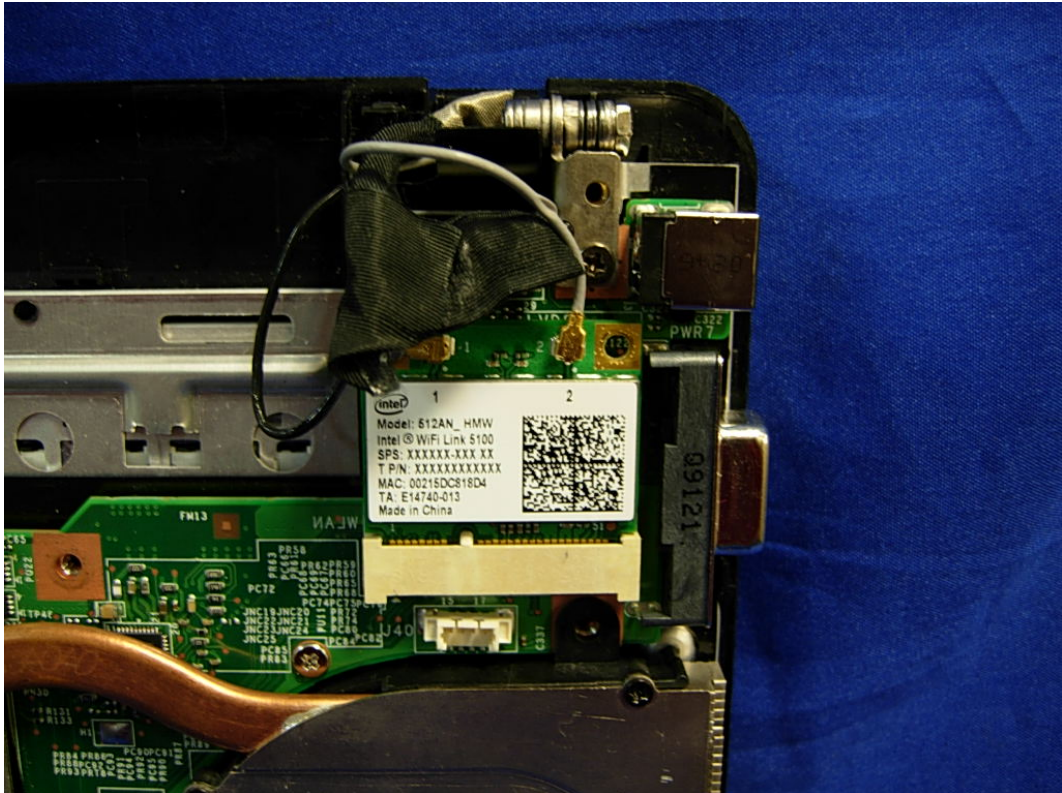
(11) EUT Photo
