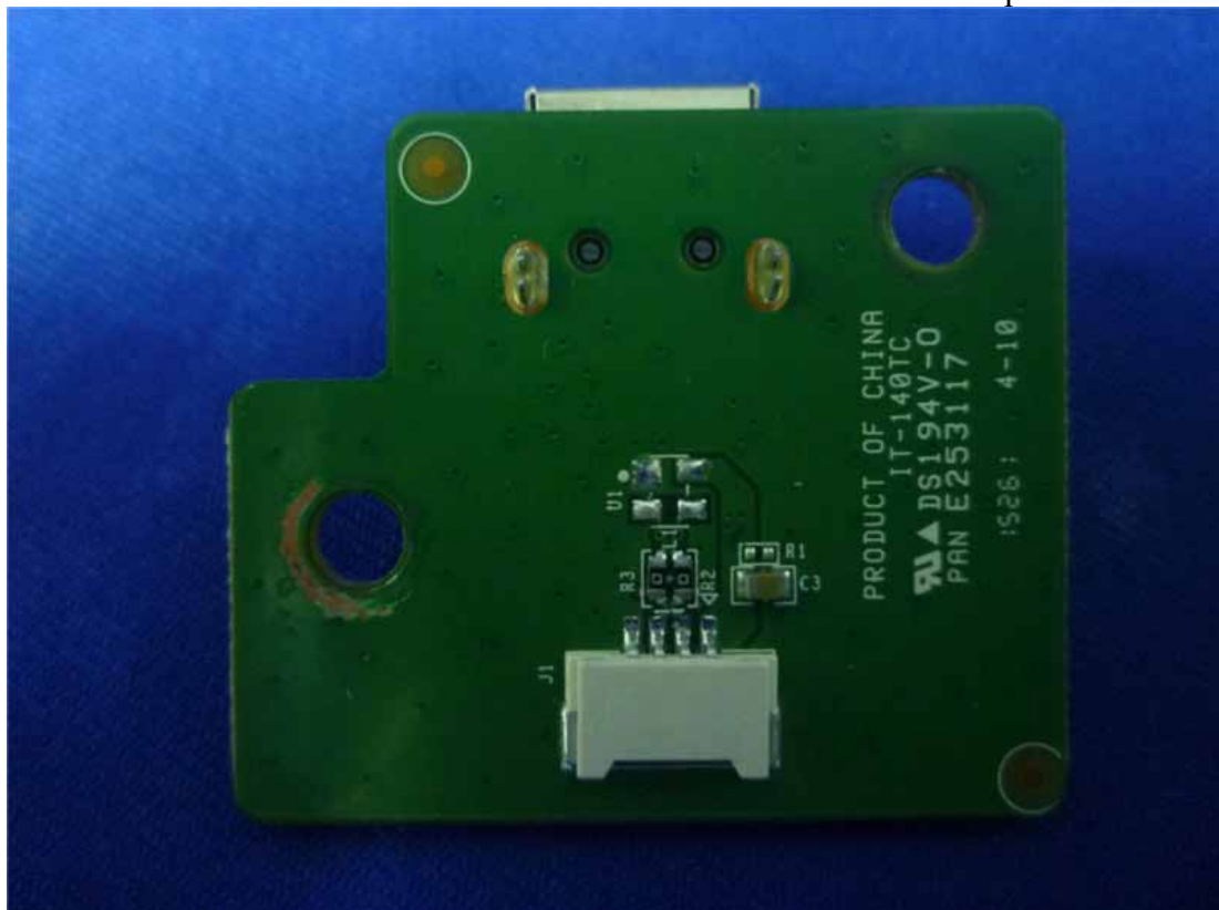
Figure 44 Components Side of the PCB
