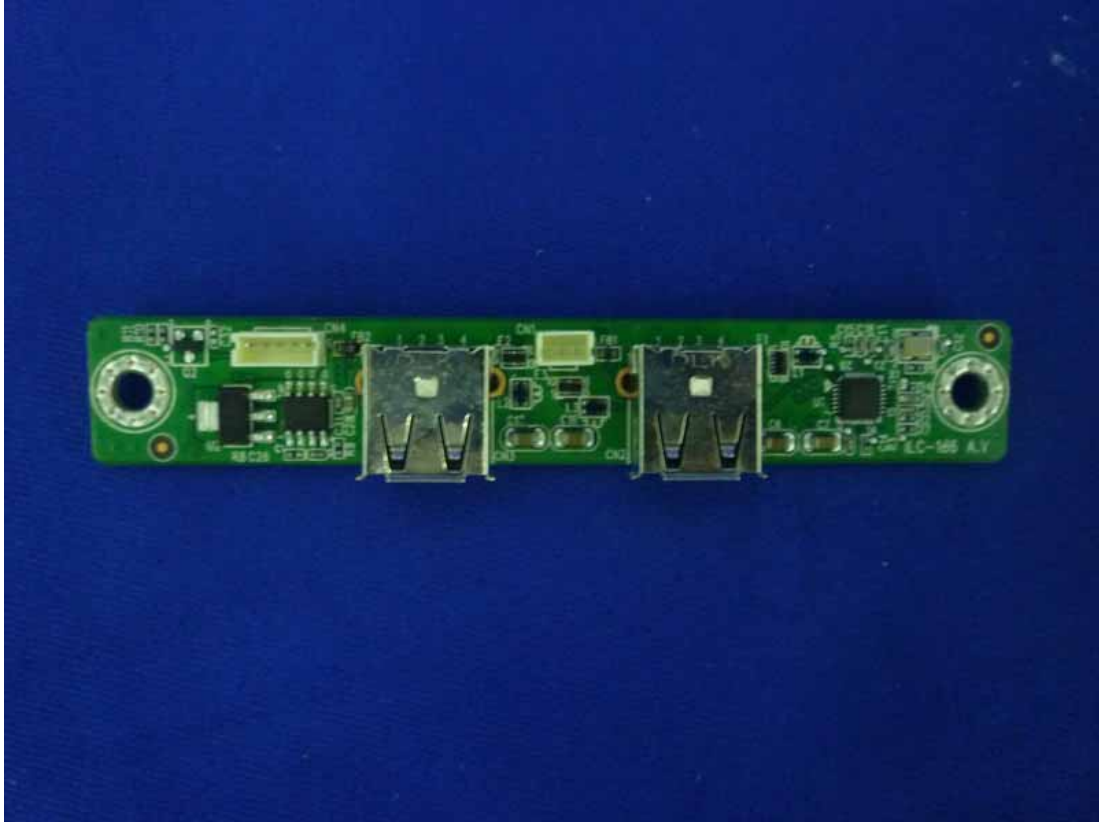
Figure 35 Components Side of the PCB
