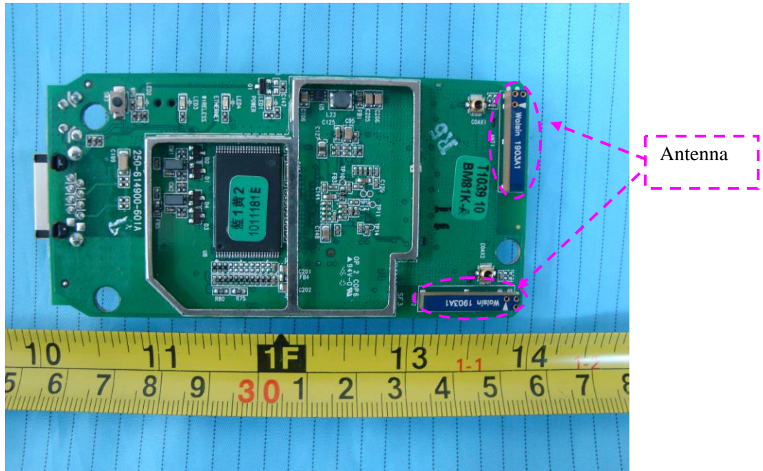
EUT – Main Board Bottom Shielding off View
