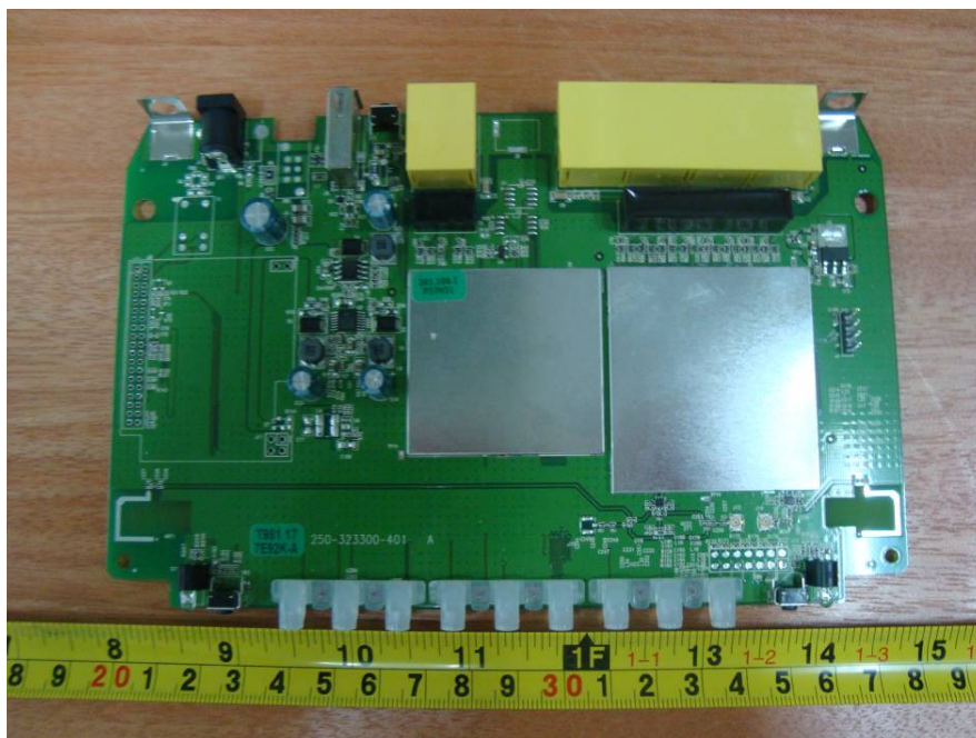
EUT – Main Board with Shielded Cover Top View
