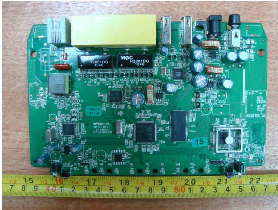
EUT – Main Board Shieding off View
