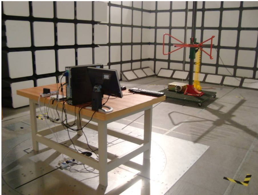
Spurious Radiated Emissions - Rear View
