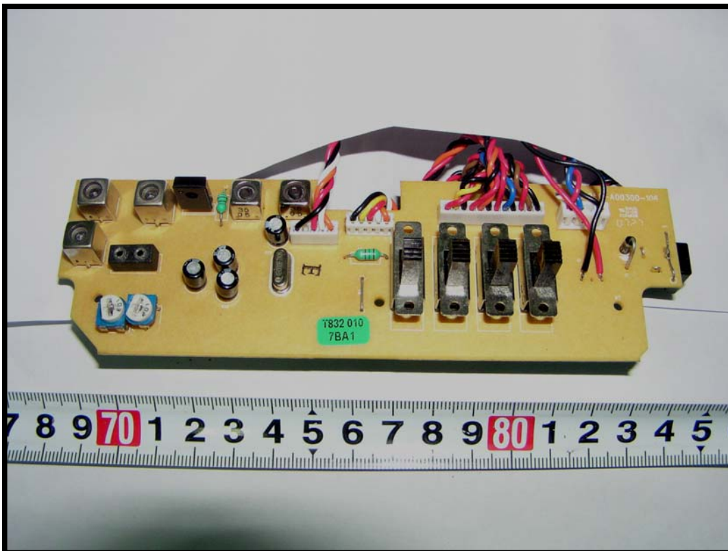
EUT- Board Top Components View
