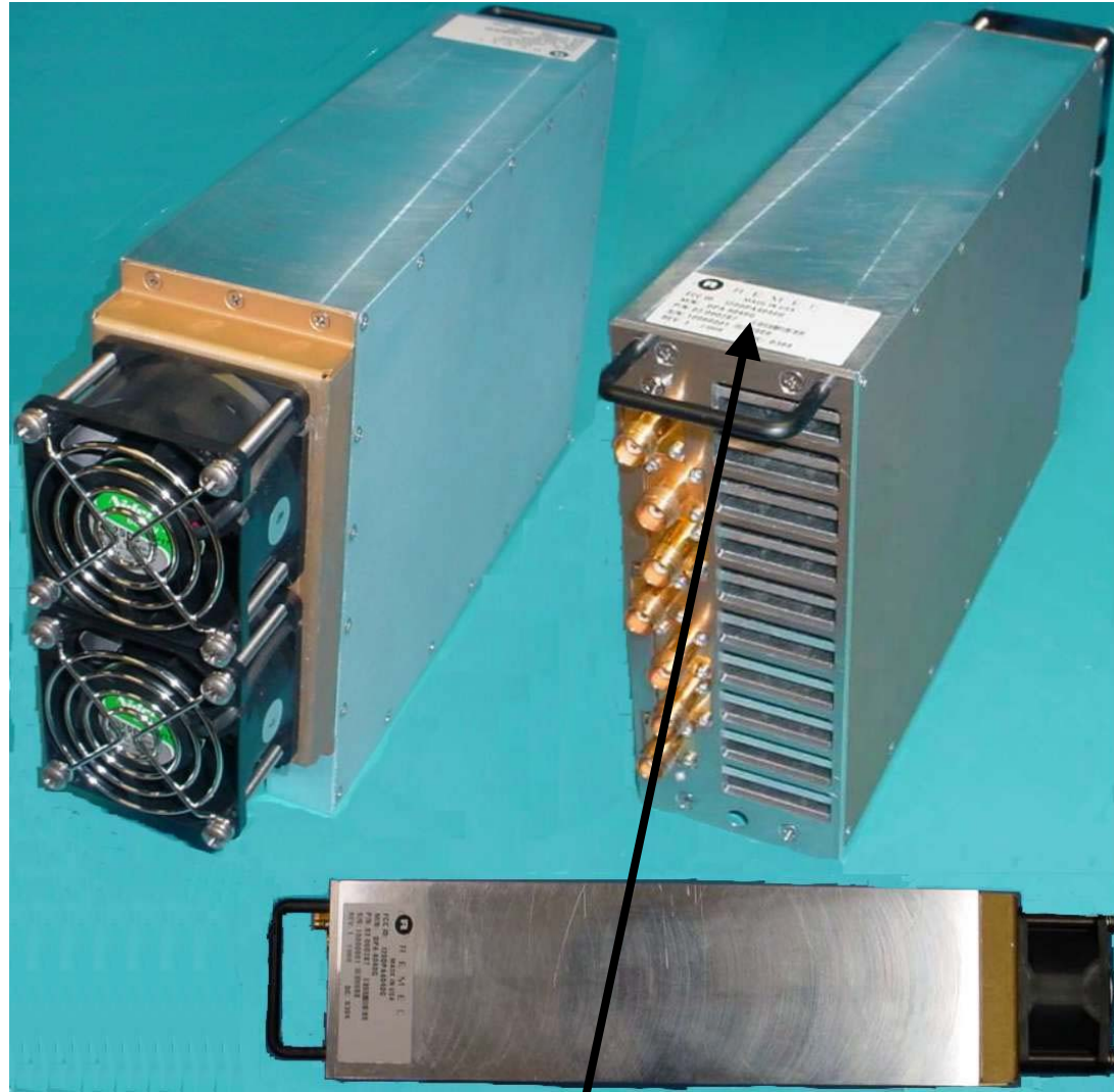
FCC ID LABEL LOCATION
