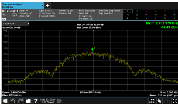
Modulation Type: GFSK(1Mbps) CH19
