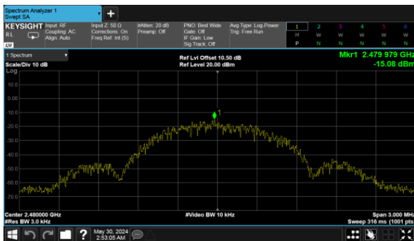
Modulation Type: GFSK(1Mbps) CH39
