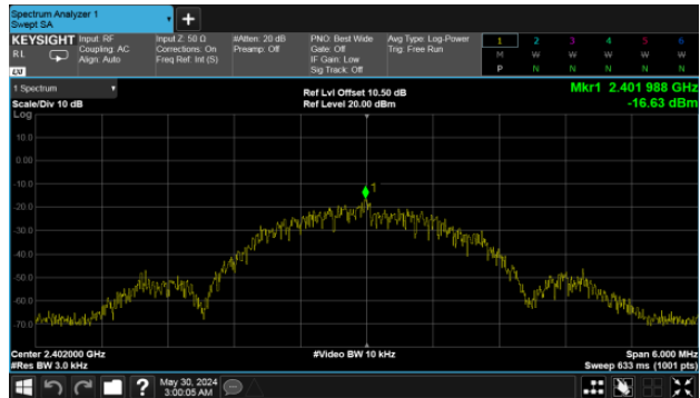
Modulation Type: GFSK(2Mbps) CH00
