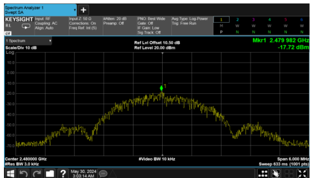
Modulation Type: GFSK(2Mbps) CH39
