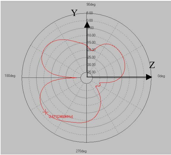
Peak Gain -2.671dBi
