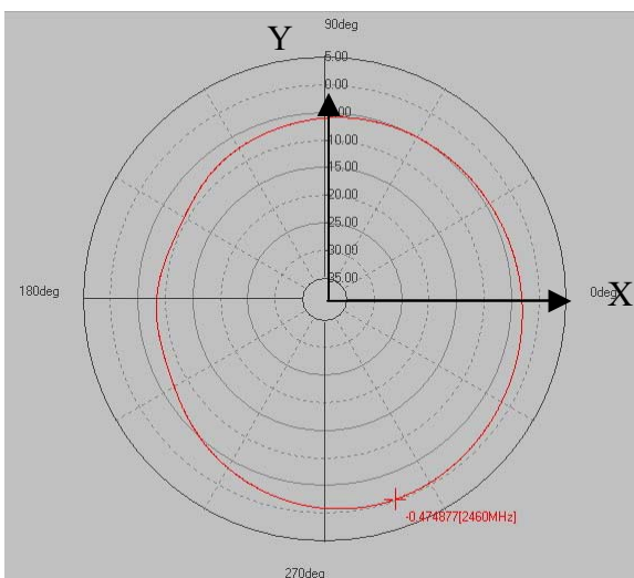
Peak Gain -3.274dBi
