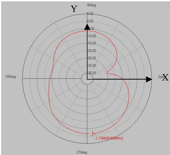
Peak Gain -1.73dBi
