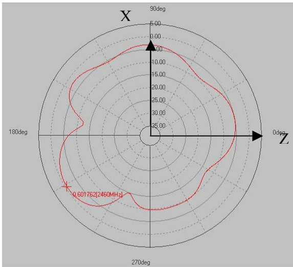
Peak Gain -0.602dBi
