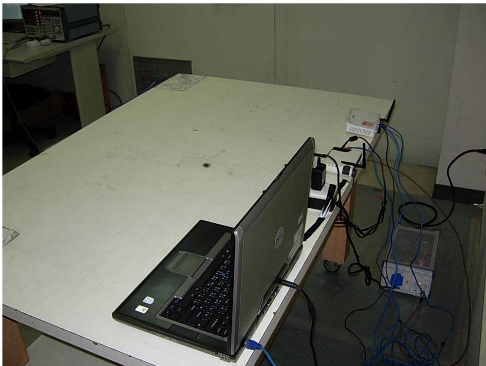
Back View of Conducted Test - Adapter: EDAC
