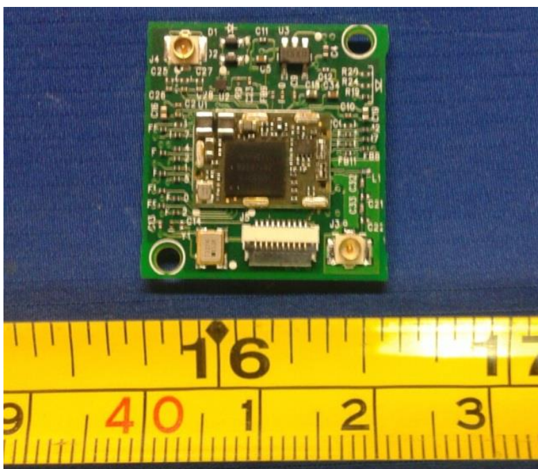
EUT Radio without Shielding Top View
