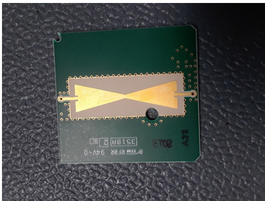
UHF PCB bow-tie antenna 3dBi
