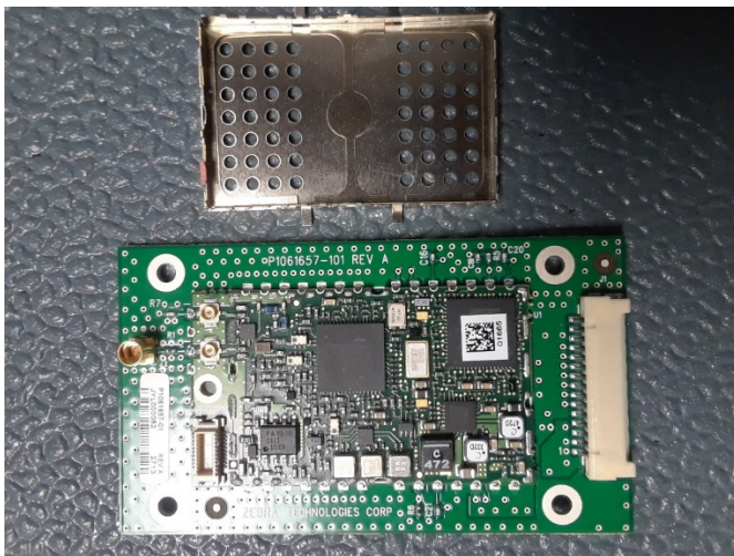
UHF PCB bow-tie antenna 3dBi
