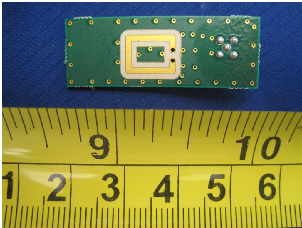
RFID Antenna-Top View
