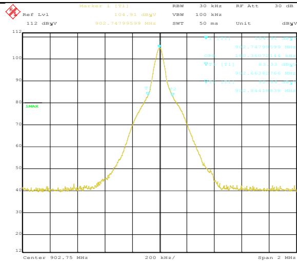
99% Occupied Bandwidth -Low Channel
