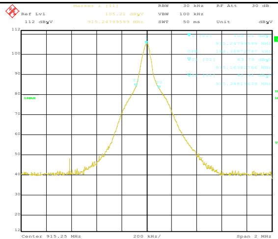
99% Occupied Bandwidth -Mid Channel
