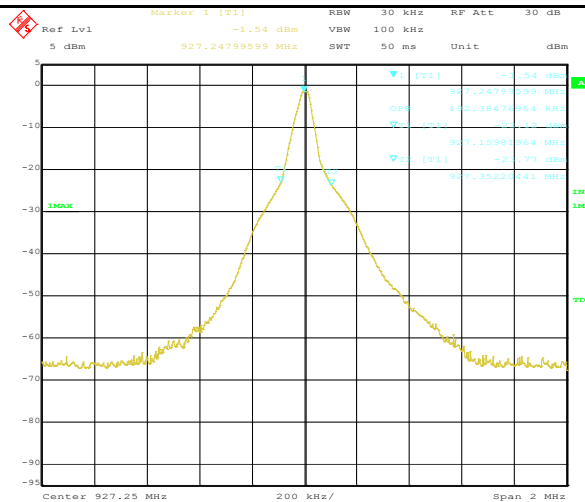
99% Occupied Bandwidth -High Channel
