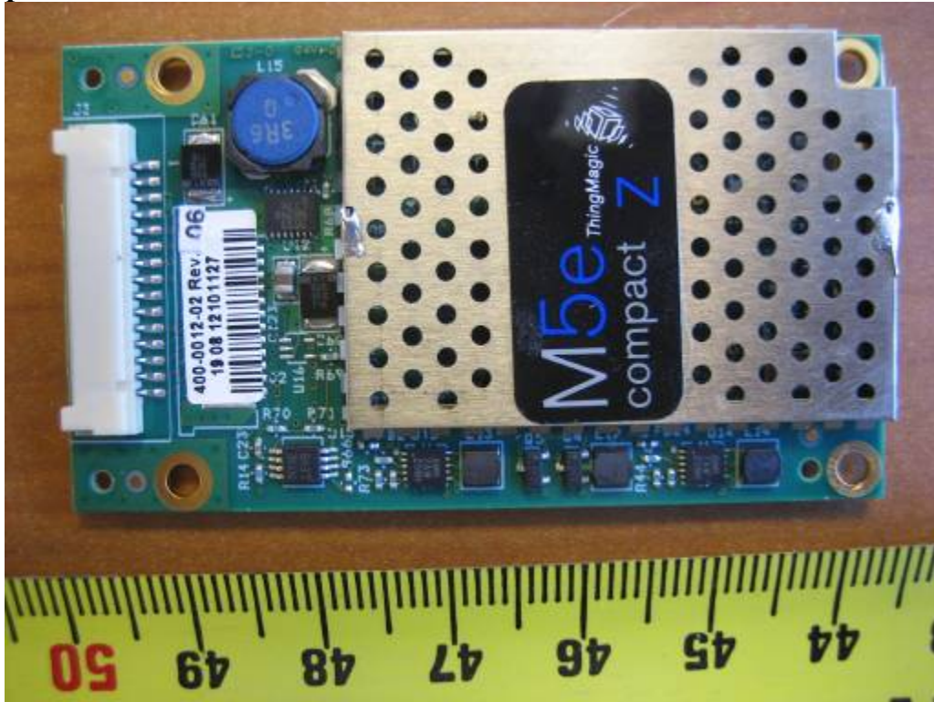
EUT Photo-RFID Radio Component View-1 with RF shield
