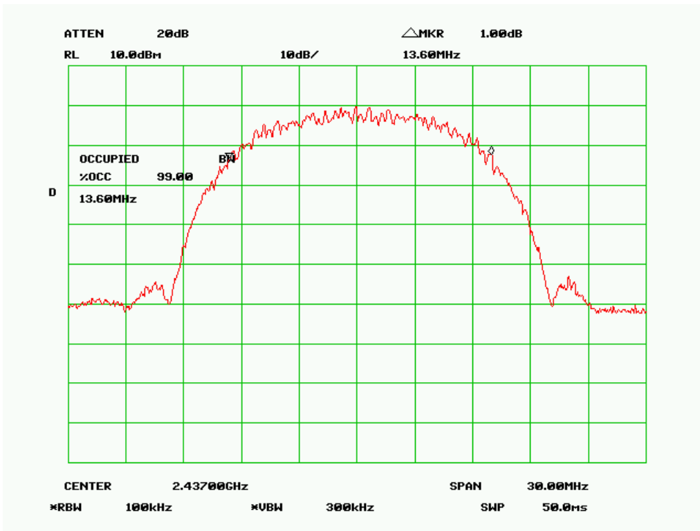
99% dB Bandwidth - 802.11b, Mid Channel
