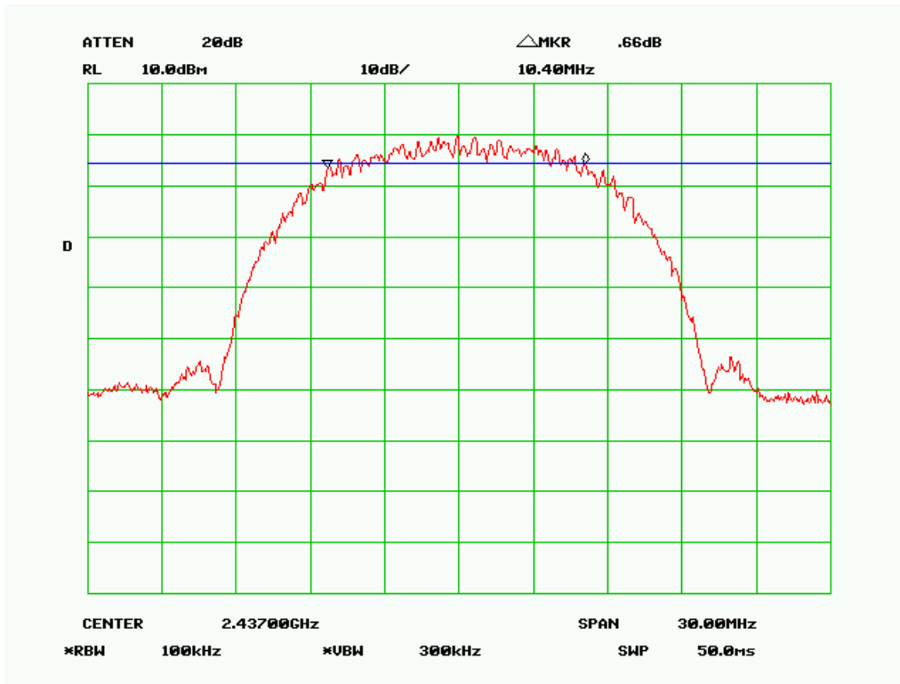
6 dB Bandwidth - 802.11b, Middle Channel
