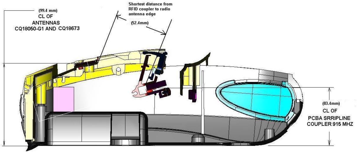
P4T CROSS SECTION 12 APRIL 2008
