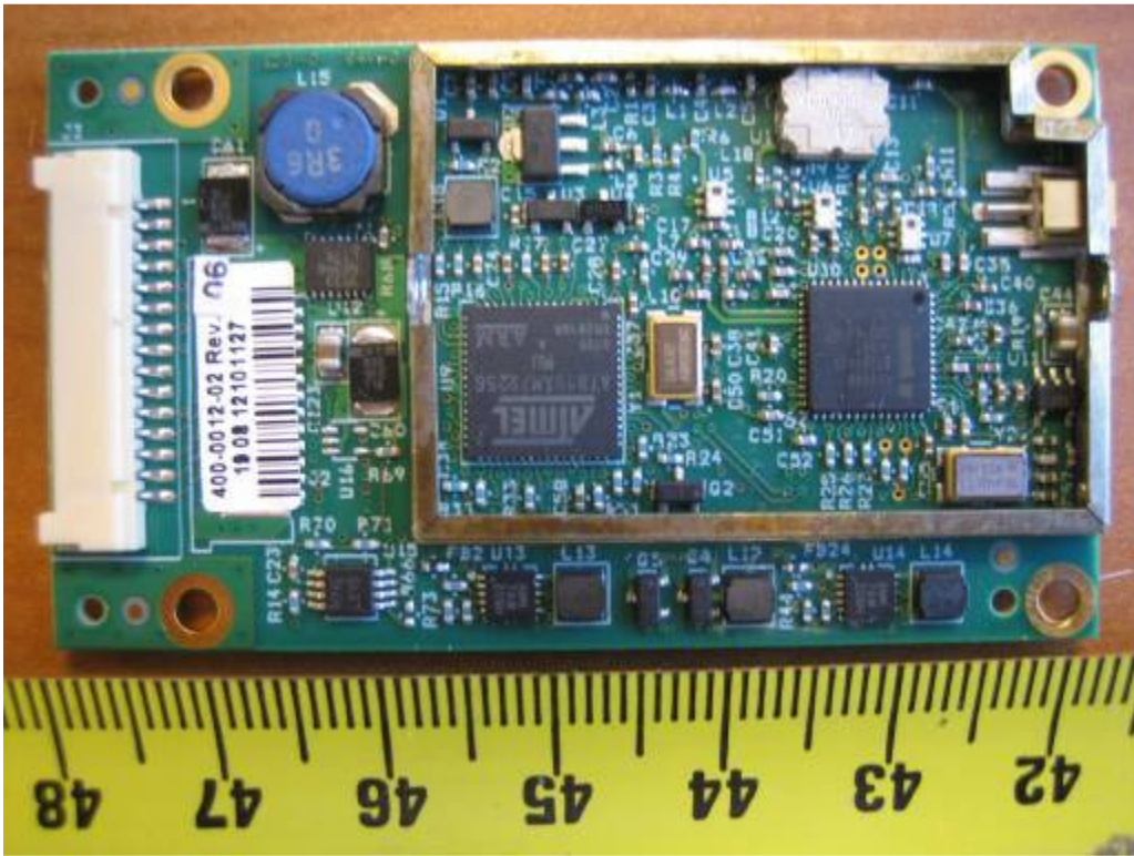
RF Module(RFID) PCBA Component View
