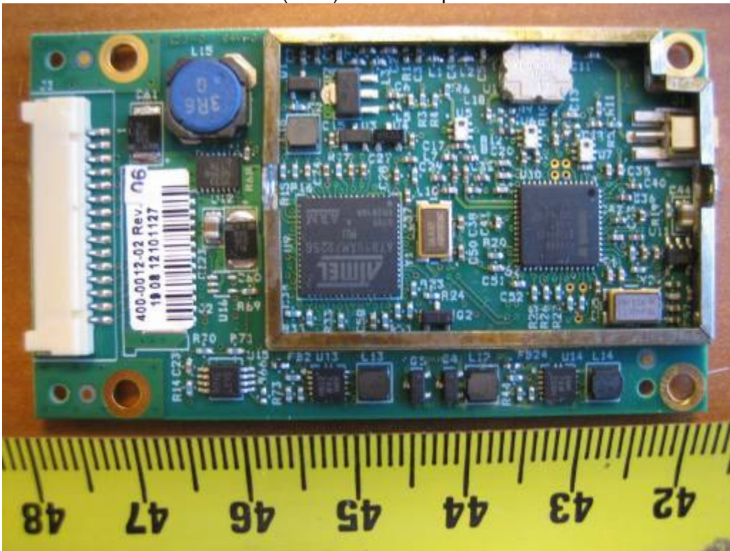
RF Module(RFID) PCBA Solder View
