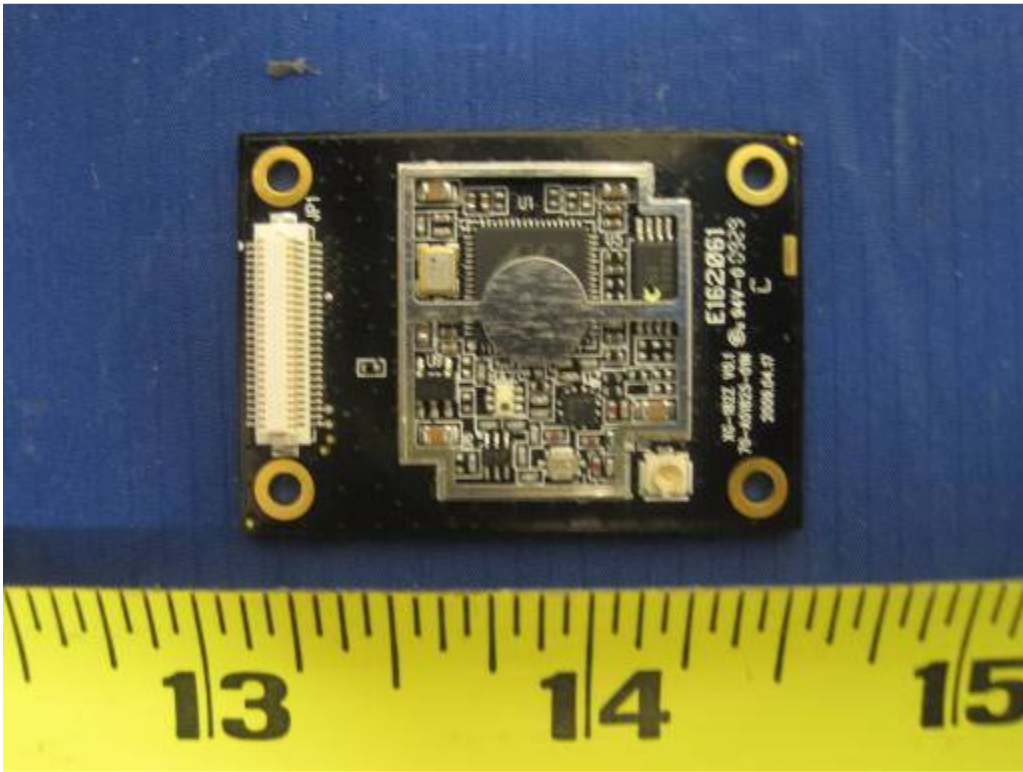
RF Module(WLAN) PCBA Component View
