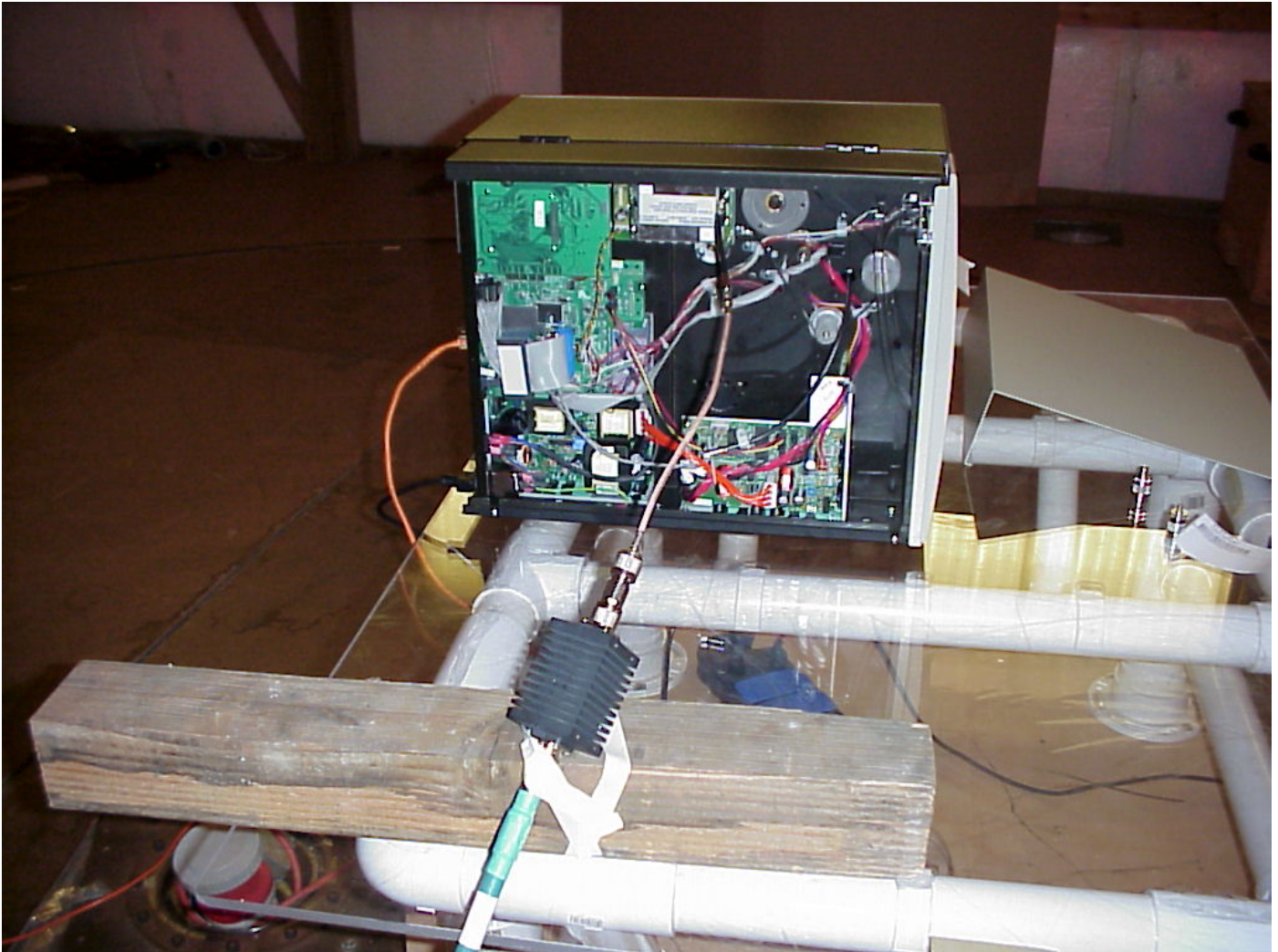
TRANSMITTER DISCONNECTED 1
